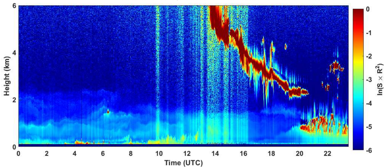
2025-01-22 RCS quick look CHM15k - ILVA LIDAR3 AGGLOMERATO
