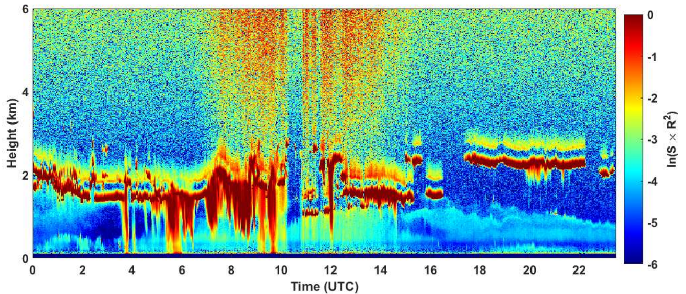
2025-01-04 RCS quick look CHM15k - ILVA LIDAR2 PARCHI
