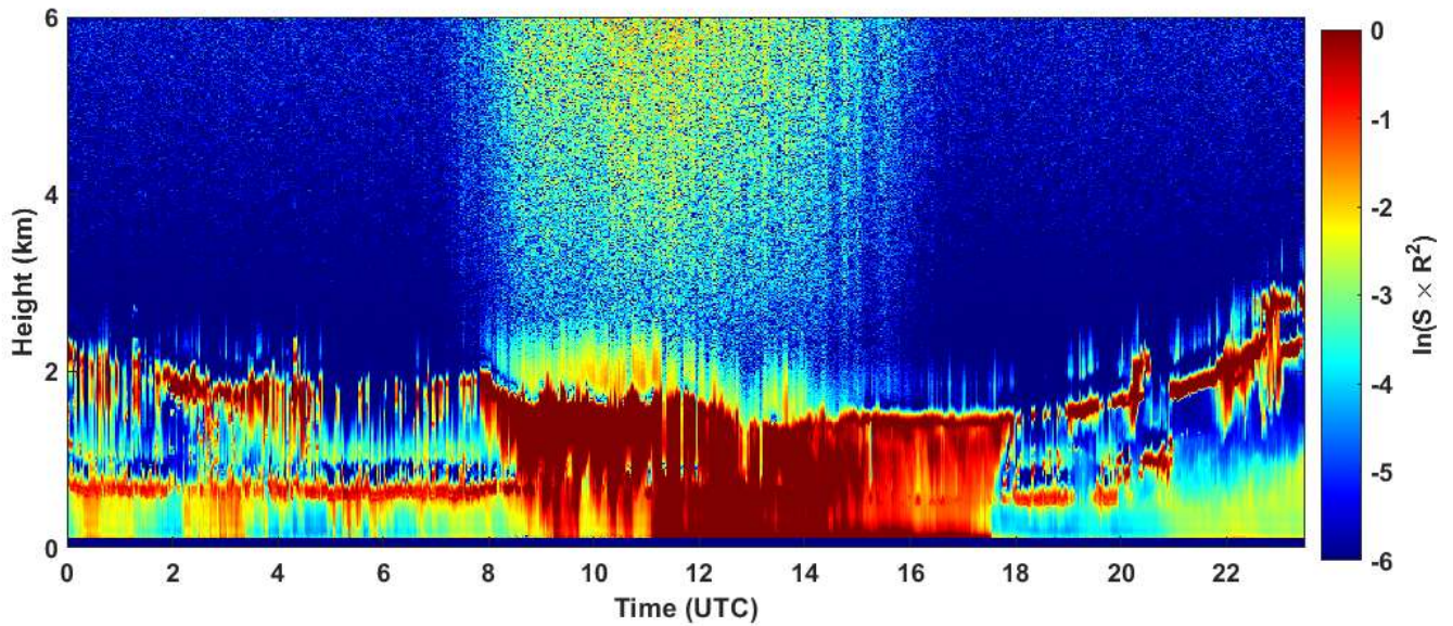
2025-01-14 RCS quick look CHM15k - ILVA LIDAR3 AGGLOMERATO
