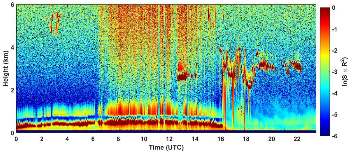
2025-01-28 RCS quick look CHM15k - ILVA LIDAR2 PARCHI
