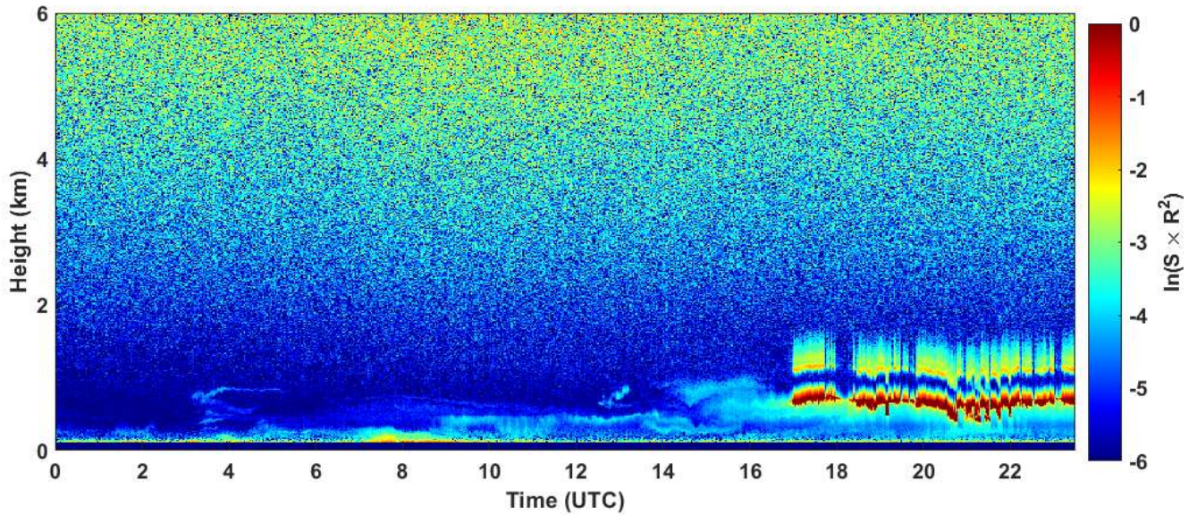
2025-01-02 RCS quick look CHM15k - ILVA LIDAR2 PARCHI
