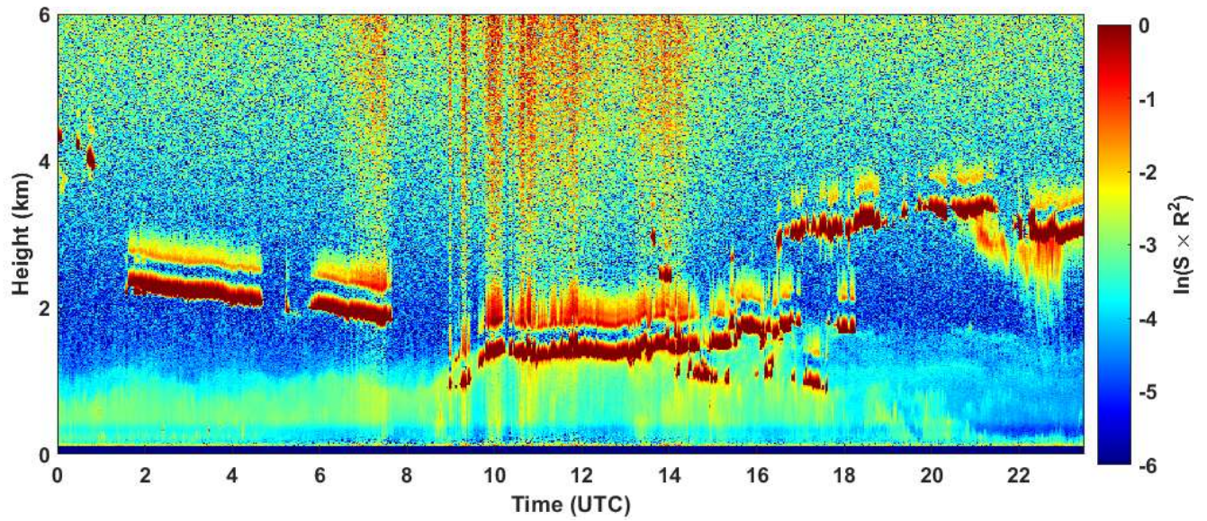
2025-01-16 RCS quick look CHM15k - ILVA LIDAR2 PARCHI
