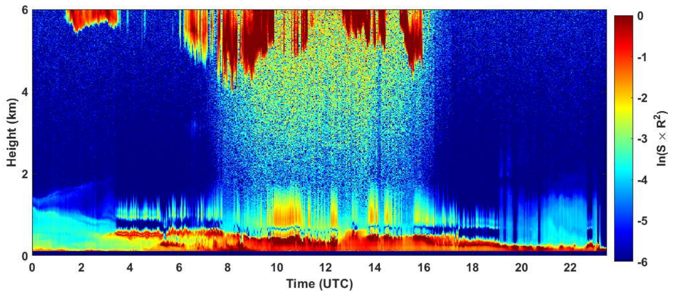
2025-01-26 RCS quick look CHM15k - ILVA LIDAR3 AGGLOMERATO
