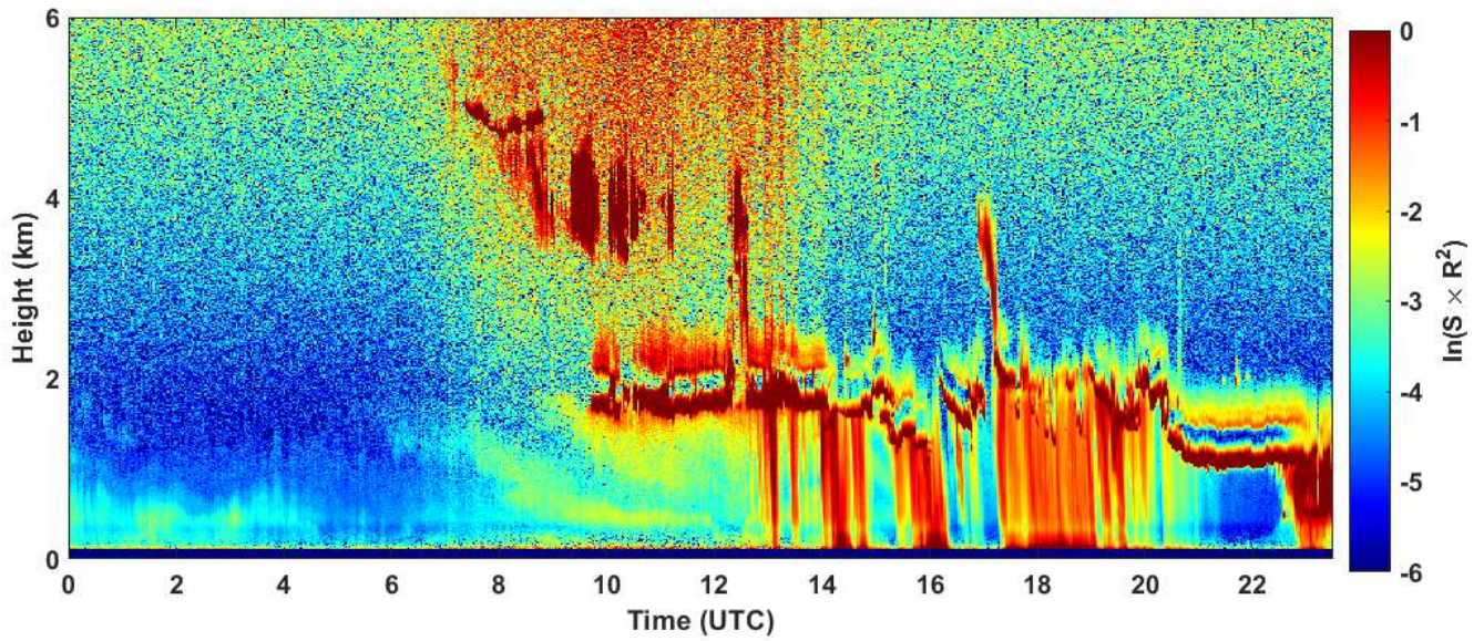
2025-01-30 RCS quick look CHM15k - ILVA LIDAR2 PARCHI
