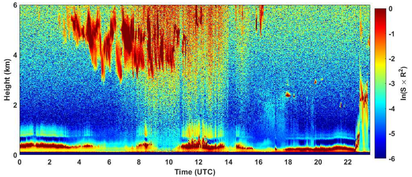
2025-01-08 RCS quick look CHM15k - ILVA LIDAR2 PARCHI
