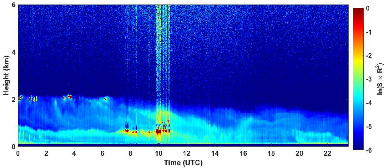
2025-01-06 RCS quick look CHM15k - ILVA LIDAR3 AGGLOMERATO
