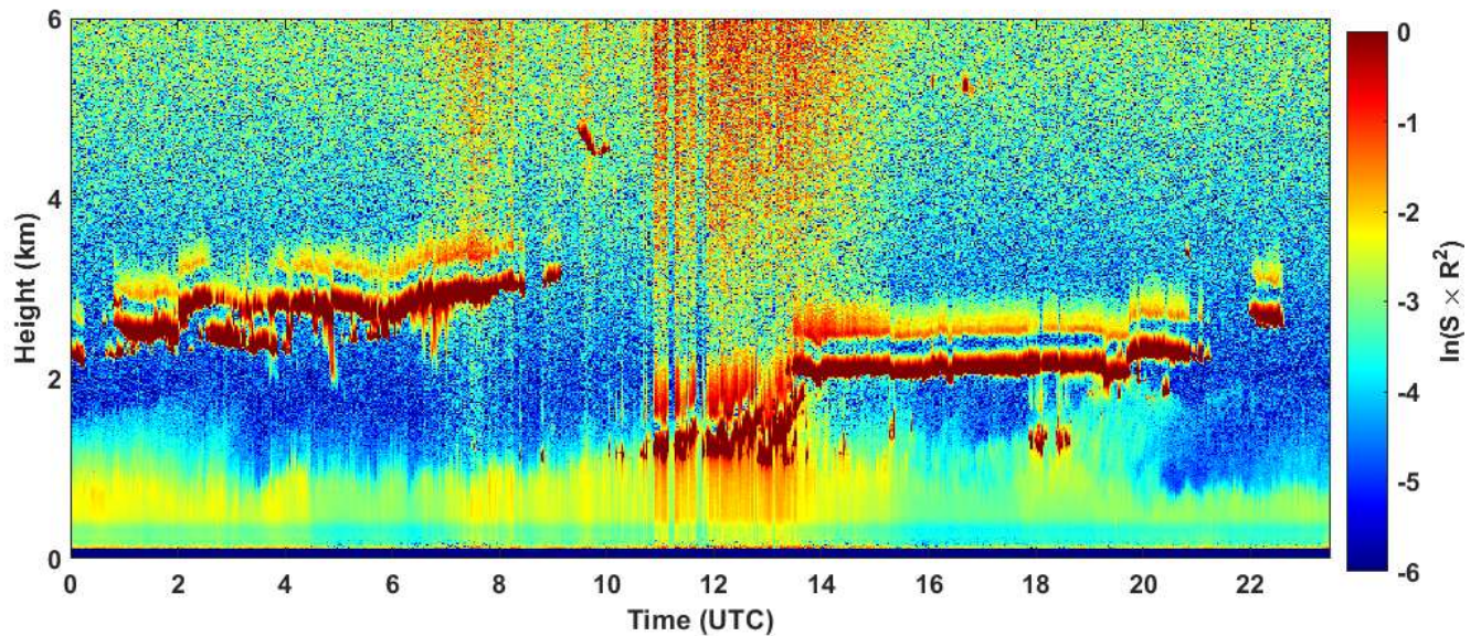
2025-01-14 RCS quick look CHM15k - ILVA LIDAR2 PARCHI
