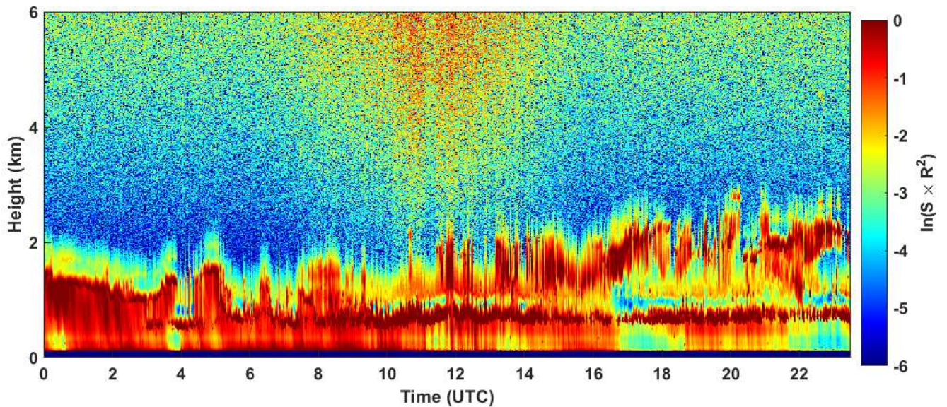
2025-01-12 RCS quick look CHM15k - ILVA LIDAR2 PARCHI
