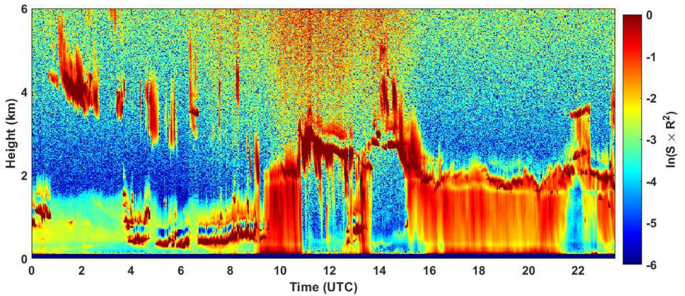
2025-01-20 RCS quick look CHM15k - ILVA LIDAR2 PARCHI
