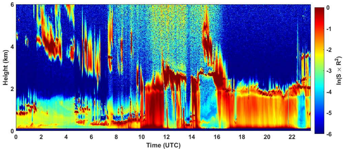
2025-01-20 RCS quick look CHM15k - ILVA LIDAR3 AGGLOMERATO
