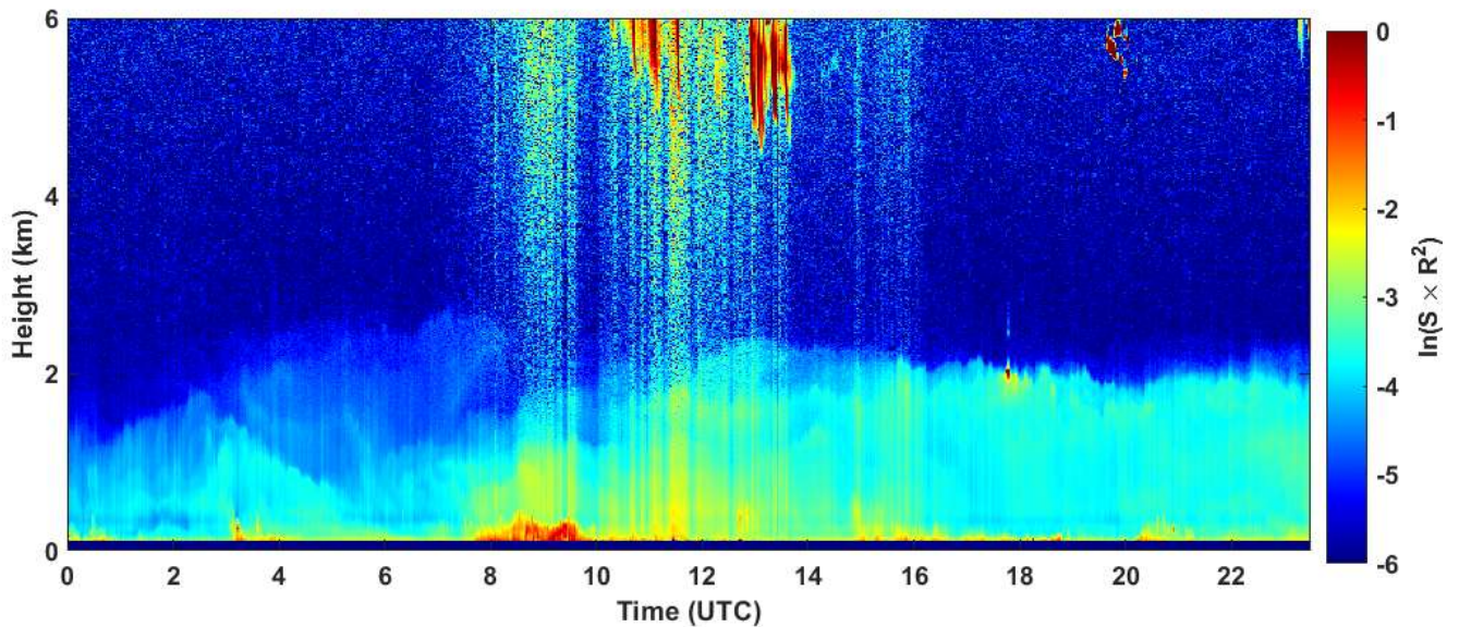
2025-01-10 RCS quick look CHM15k - ILVA LIDAR3 AGGLOMERATO
