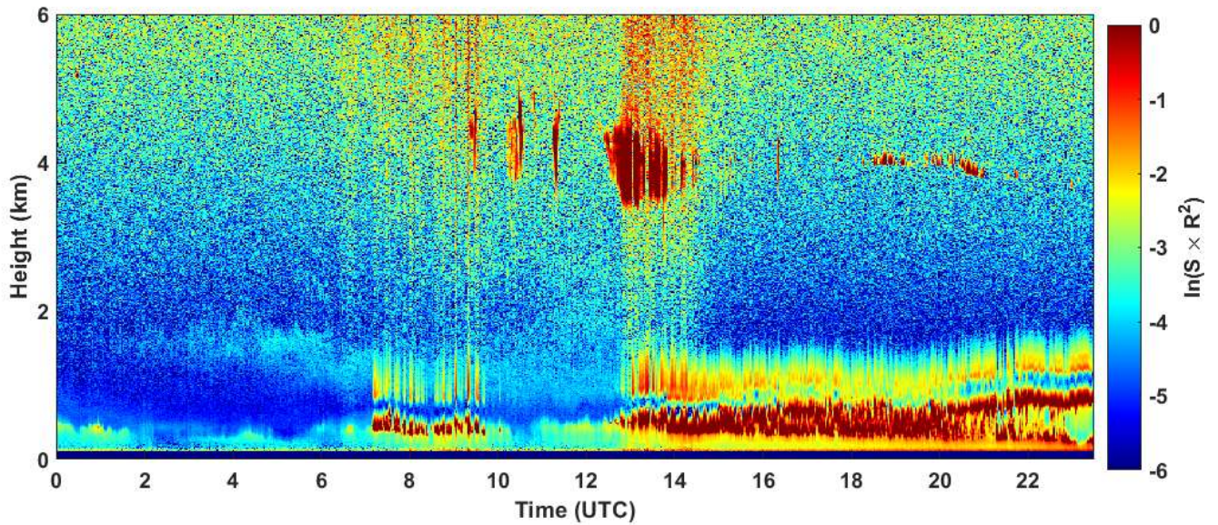
2025-01-24 RCS quick look CHM15k - ILVA LIDAR2 PARCHI
