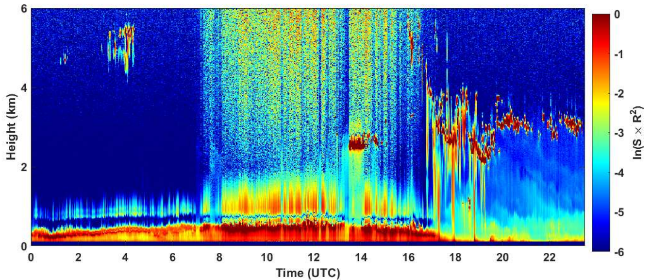
2025-01-28 RCS quick look CHM15k - ILVA LIDAR3 AGGLOMERATO
