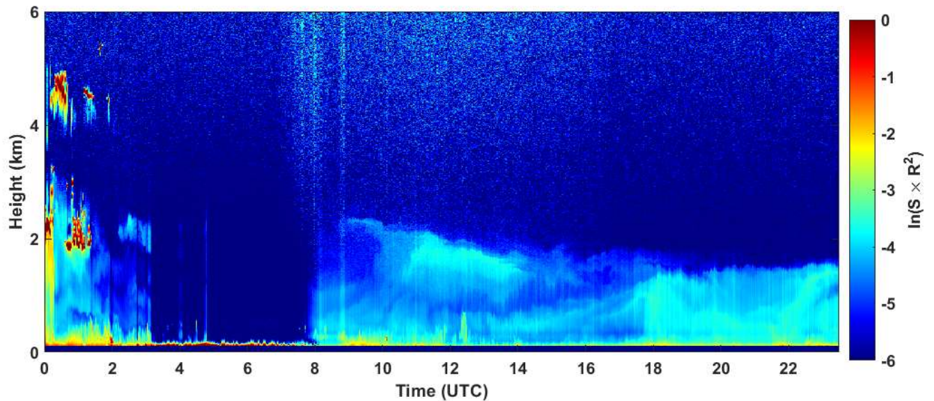
2025-01-08 RCS quick look CHM15k - ILVA LIDAR3 AGGLOMERATO
