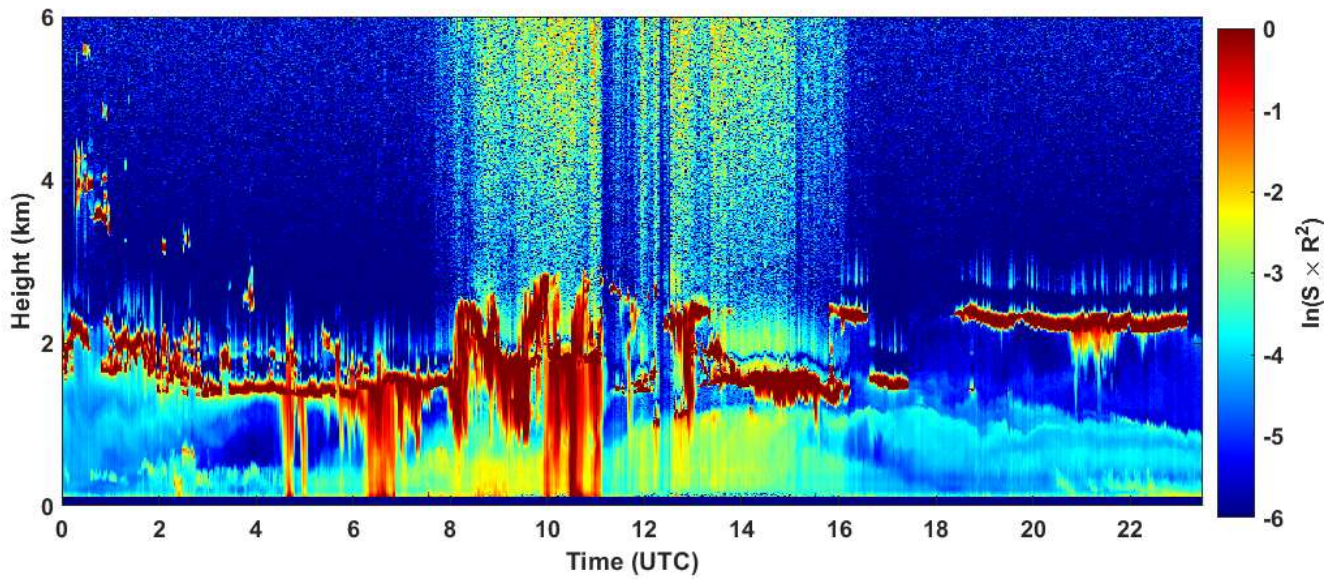
2025-01-04 RCS quick look CHM15k - ILVA LIDAR3 AGGLOMERATO
