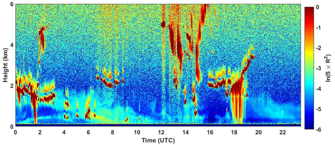
2025-01-22 RCS quick look CHM15k - ILVA LIDAR2 PARCHI
