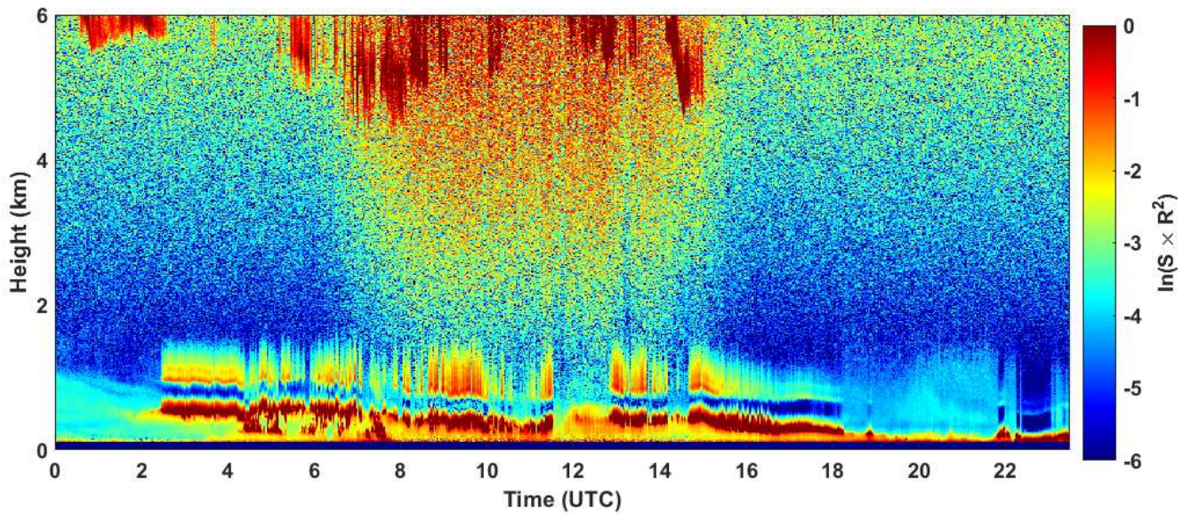
2025-01-26 RCS quick look CHM15k - ILVA LIDAR2 PARCHI
