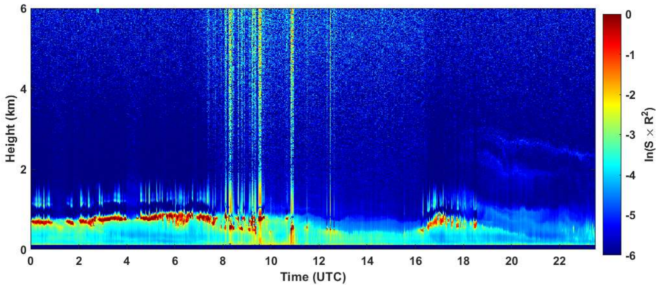
2025-01-02 RCS quick look CHM15k - ILVA LIDAR3 AGGLOMERATO
