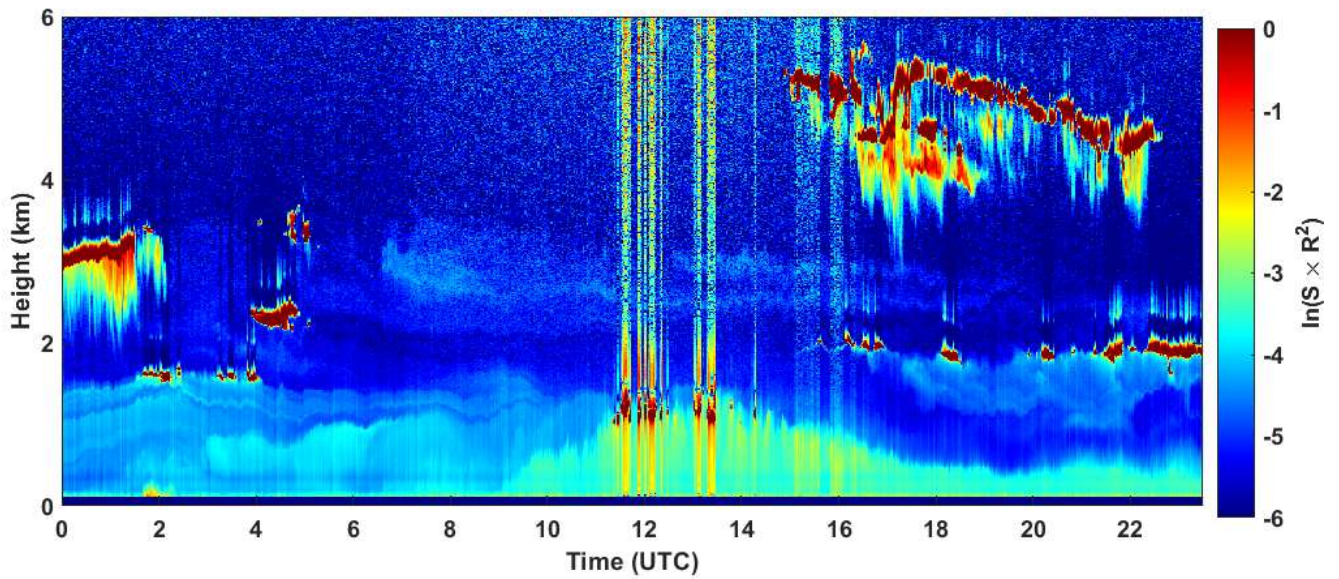
2025-01-16 RCS quick look CHM15k - ILVA LIDAR3 AGGLOMERATO
