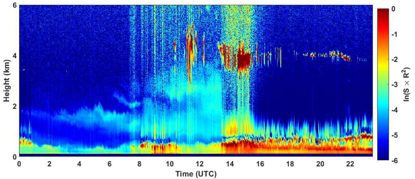
2025-01-24 RCS quick look CHM15k - ILVA LIDAR3 AGGLOMERATO
