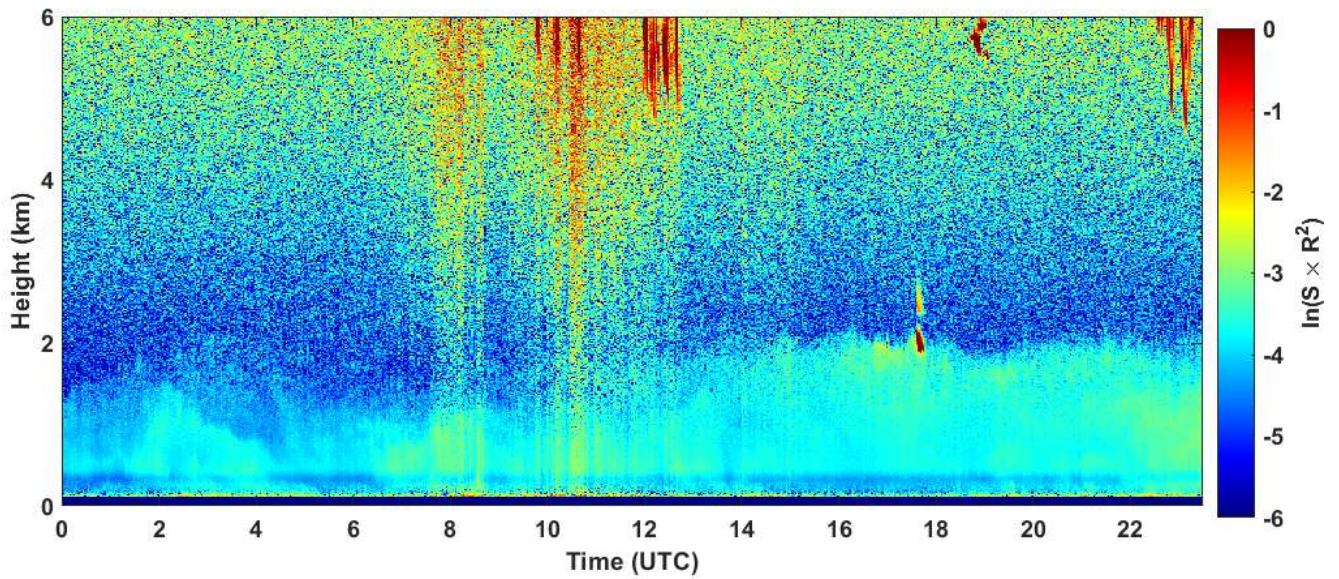
2025-01-10 RCS quick look CHM15k - ILVA LIDAR2 PARCHI
