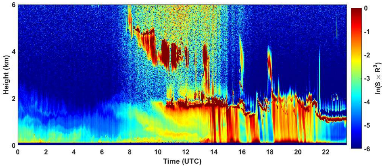
2025-01-30 RCS quick look CHM15k - ILVA LIDAR3 AGGLOMERATO
