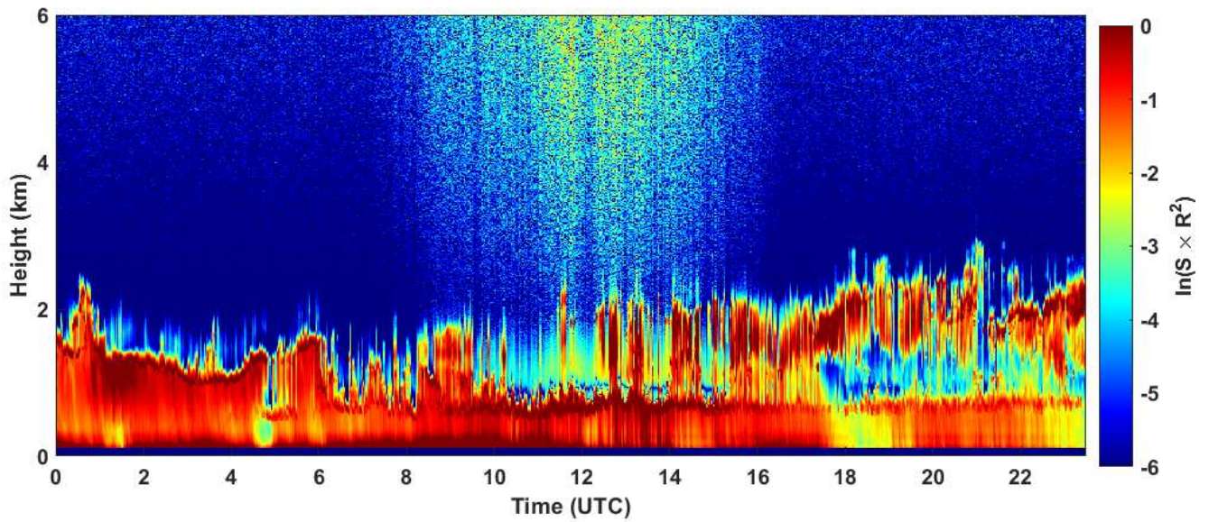
2025-01-12 RCS quick look CHM15k - ILVA LIDAR3 AGGLOMERATO
