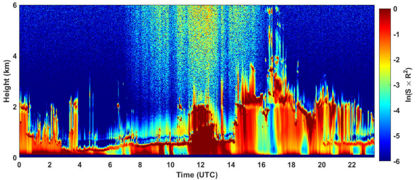
2024-12-06 RCS quick look CHM15k - ILVA LIDAR3 AGGLOMERATO
