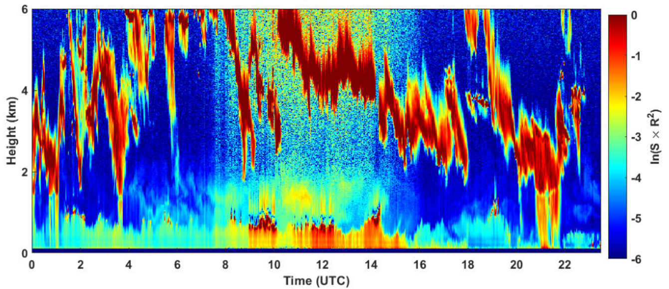
2024-12-10 RCS quick look CHM15k - ILVA LIDAR3 AGGLOMERATO
