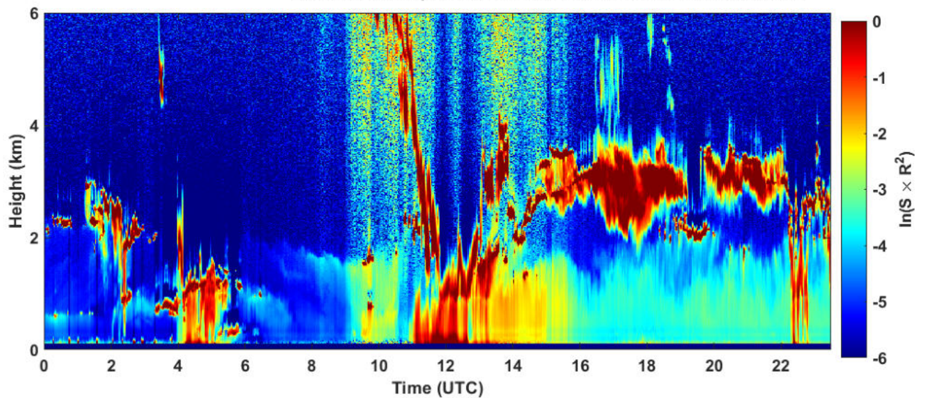
2024-12-24 RCS quick look CHM15k - ILVA LIDAR3 AGGLOMERATO
