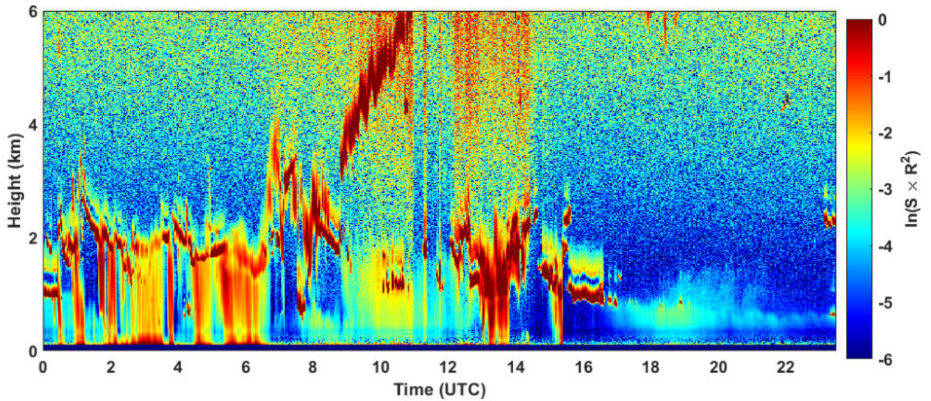
2024-12-24 RCS quick look CHM15k - ILVA LIDAR2 PARCHI
