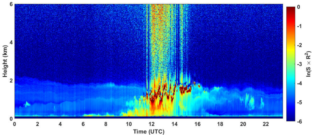
2024-12-12 RCS quick look CHM15k - ILVA LIDAR3 AGGLOMERATO
