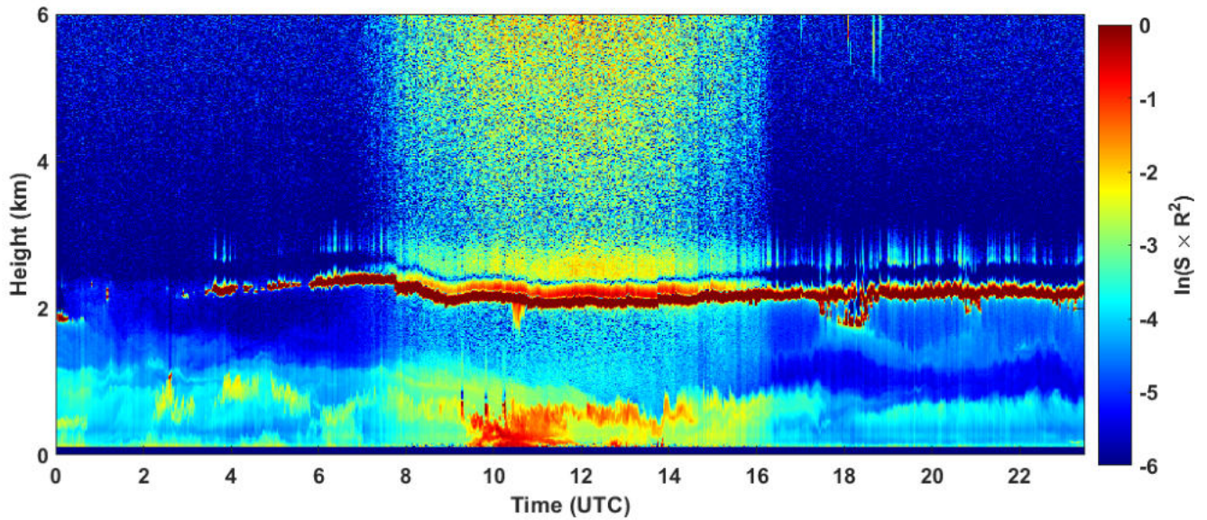
2024-12-04 RCS quick look CHM15k - ILVA LIDAR3 AGGLOMERATO
