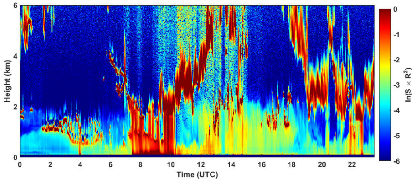
2024-12-08 RCS quick look CHM15k - ILVA LIDAR3 AGGLOMERATO
