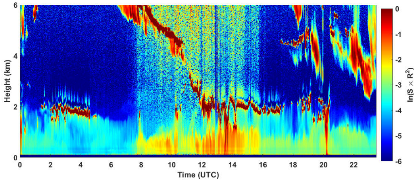
2024-12-26 RCS quick look CHM15k - ILVA LIDAR3 AGGLOMERATO
