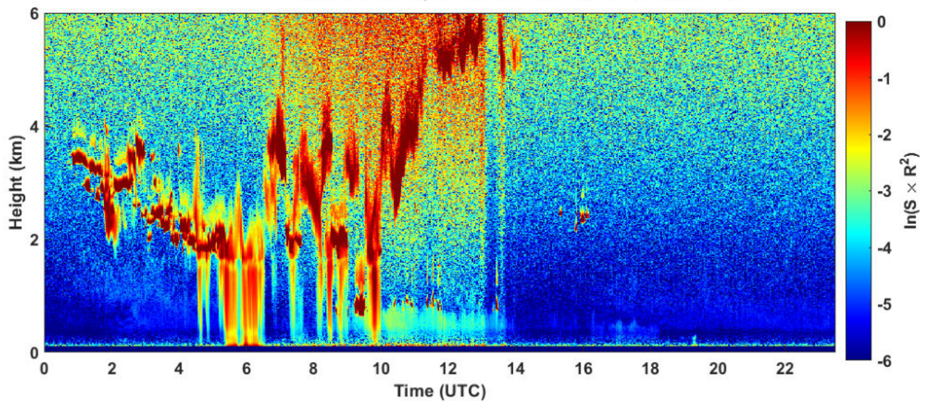
2024-12-10 RCS quick look CHM15k - ILVA LIDAR2 PARCHI
