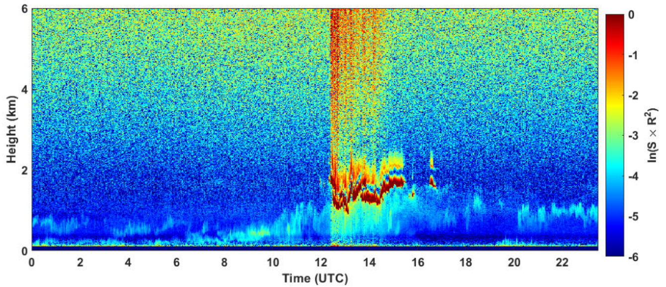
2024-12-12 RCS quick look CHM15k - ILVA LIDAR2 PARCHI
