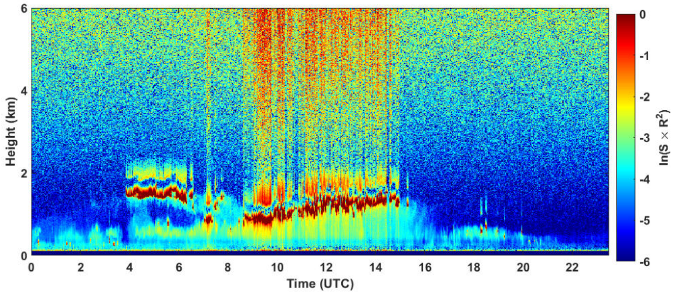
2024-12-30 RCS quick look CHM15k - ILVA LIDAR2 PARCHI
