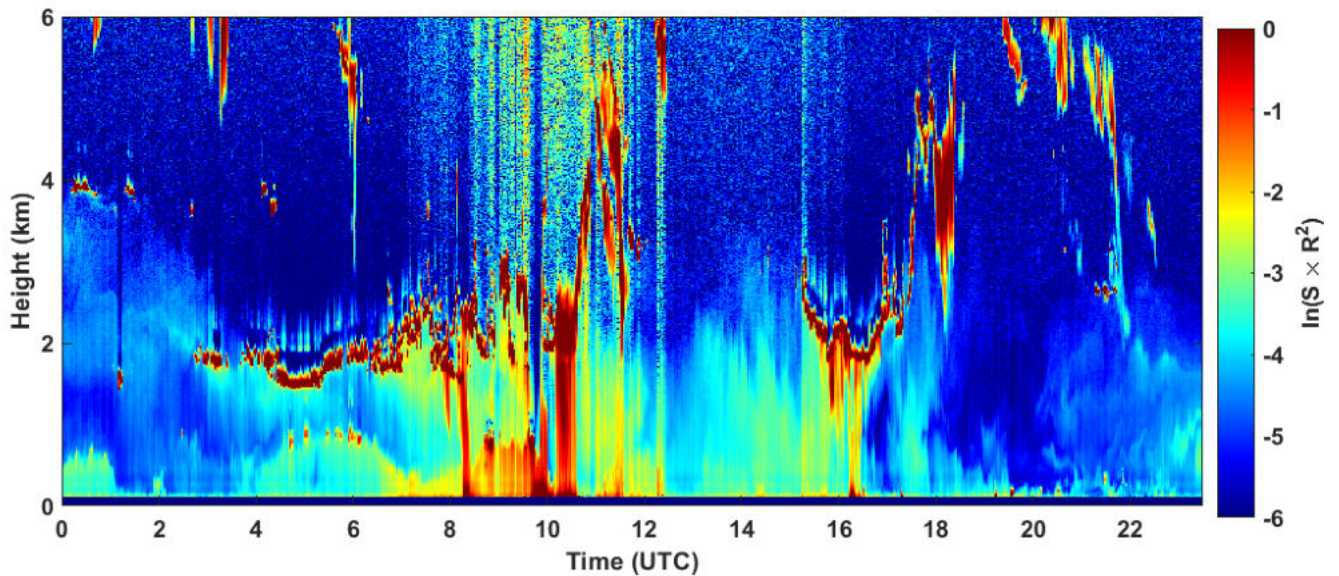
2024-12-20 RCS quick look CHM15k - ILVA LIDAR3 AGGLOMERATO
