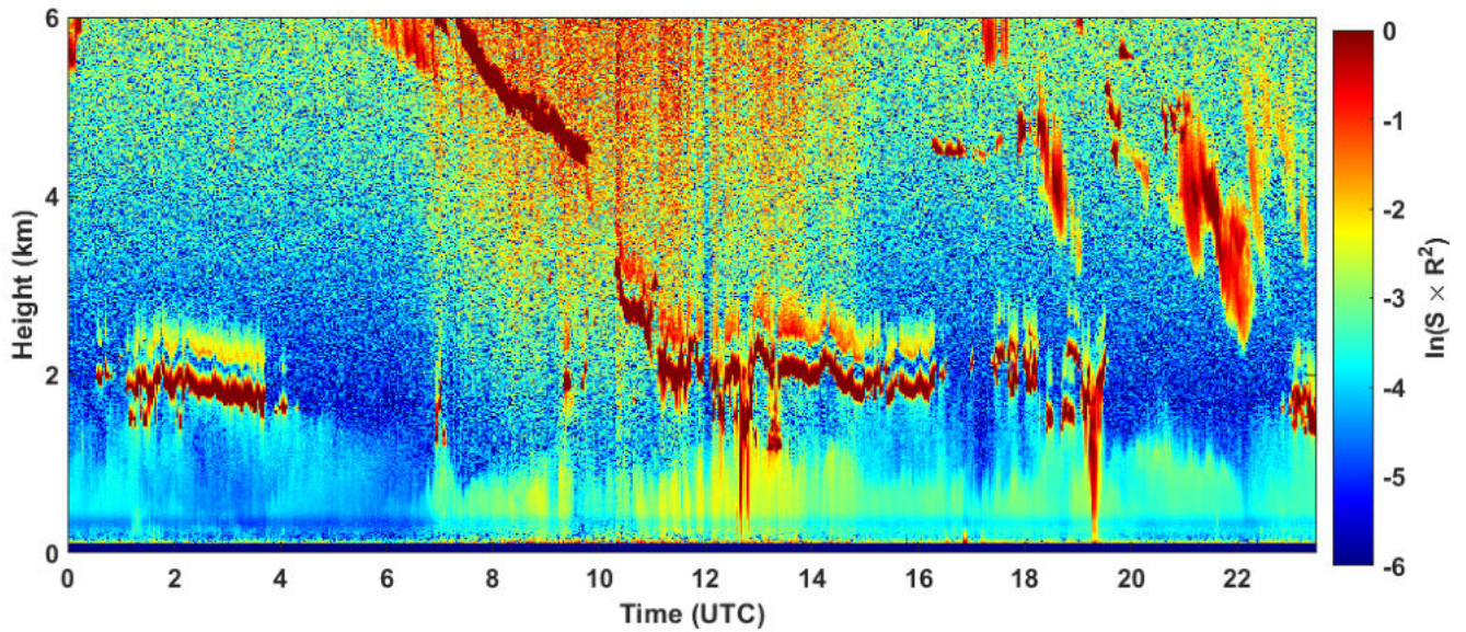
2024-12-26 RCS quick look CHM15k - ILVA LIDAR2 PARCHI
