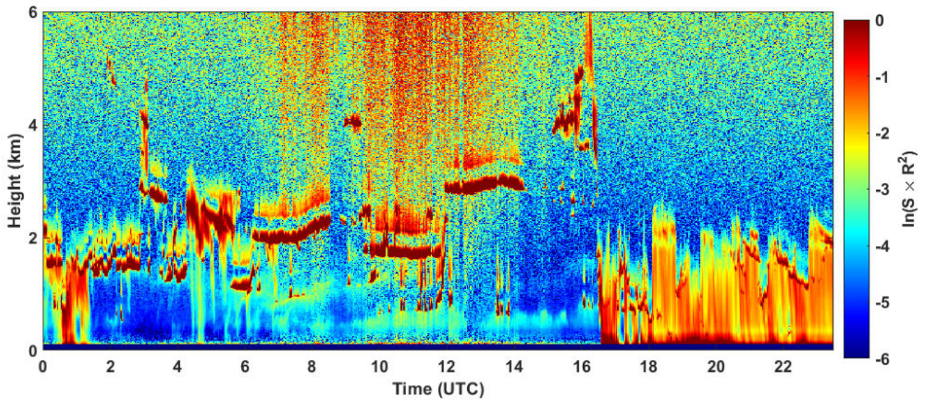
2024-12-04 RCS quick look CHM15k - ILVA LIDAR2 PARCHI
