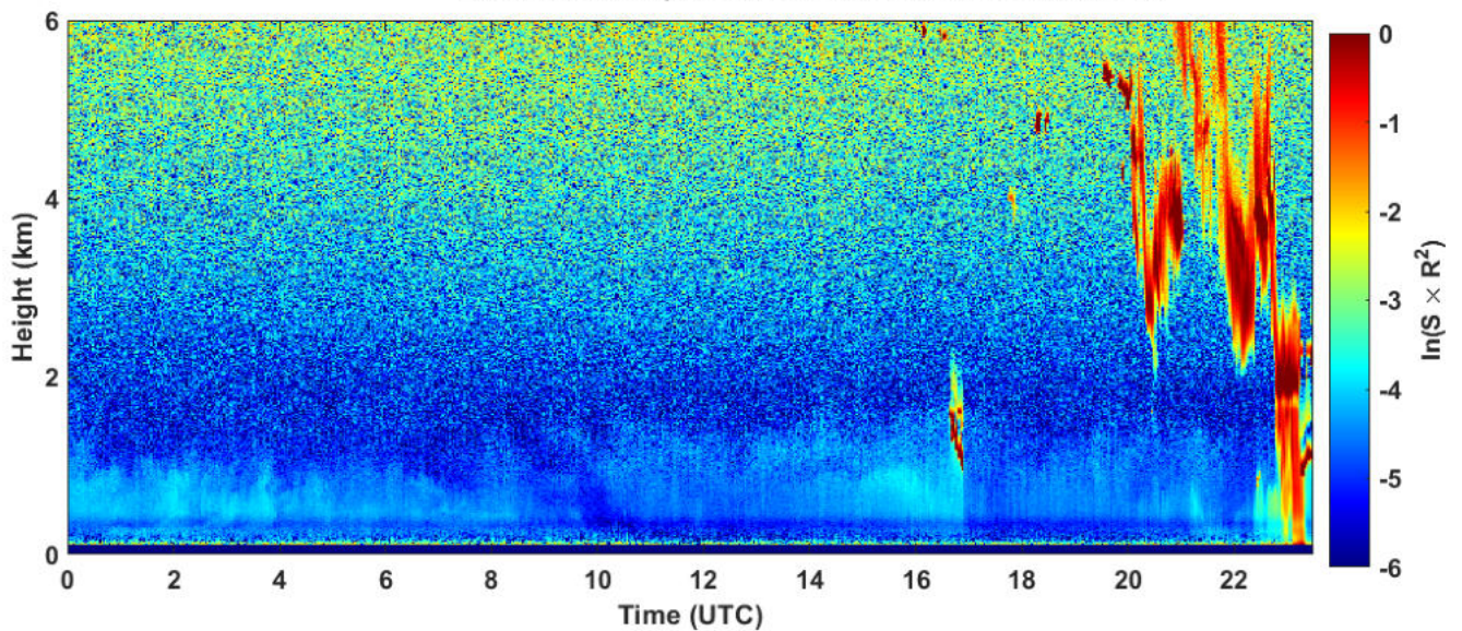
2024-12-22 RCS quick look CHM15k - ILVA LIDAR2 PARCHI
