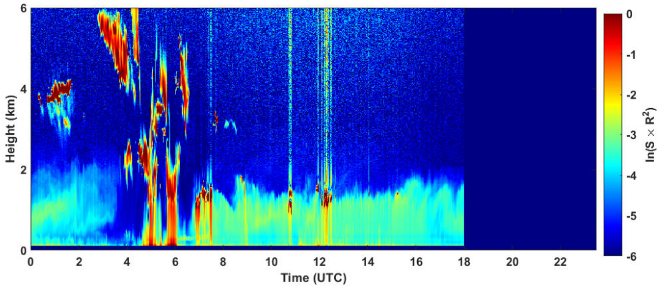
2024-12-22 RCS quick look CHM15k - ILVA LIDAR3 AGGLOMERATO
