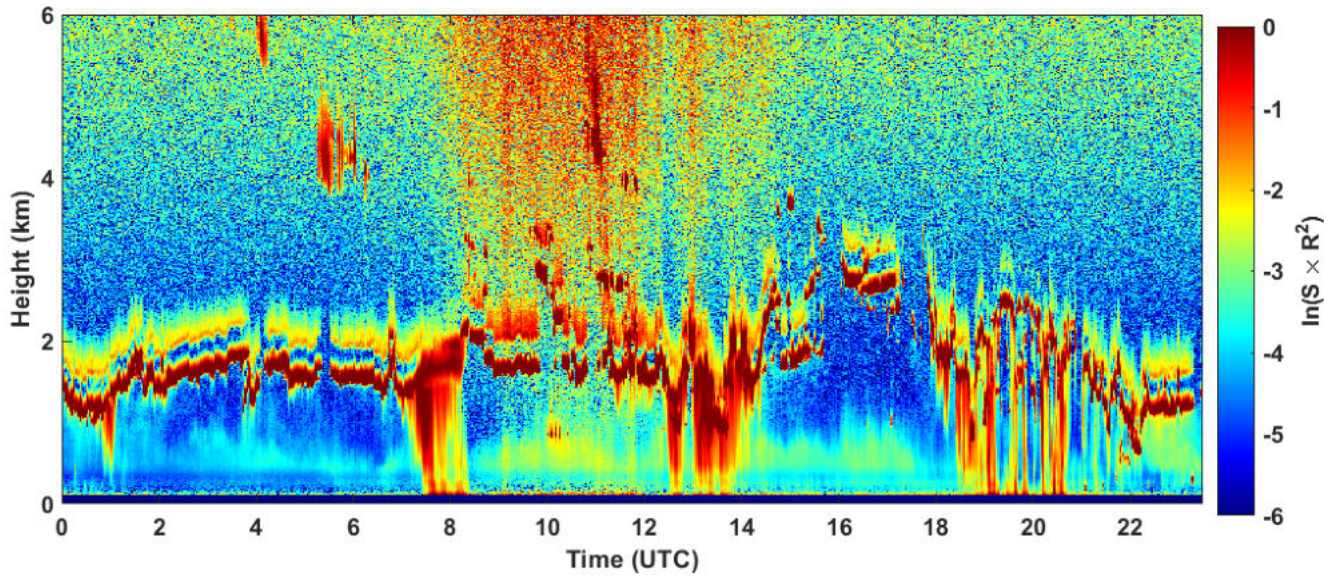
2024-12-02 RCS quick look CHM15k - ILVA LIDAR2 PARCHI
