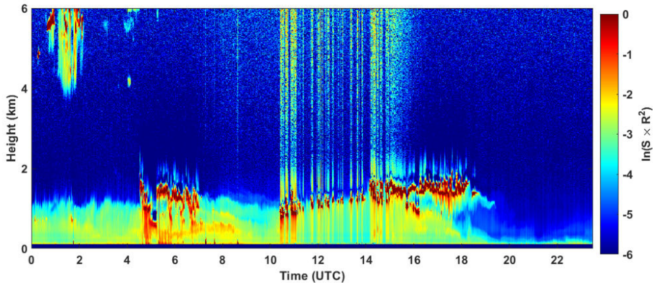
2024-12-28 RCS quick look CHM15k - ILVA LIDAR3 AGGLOMERATO
