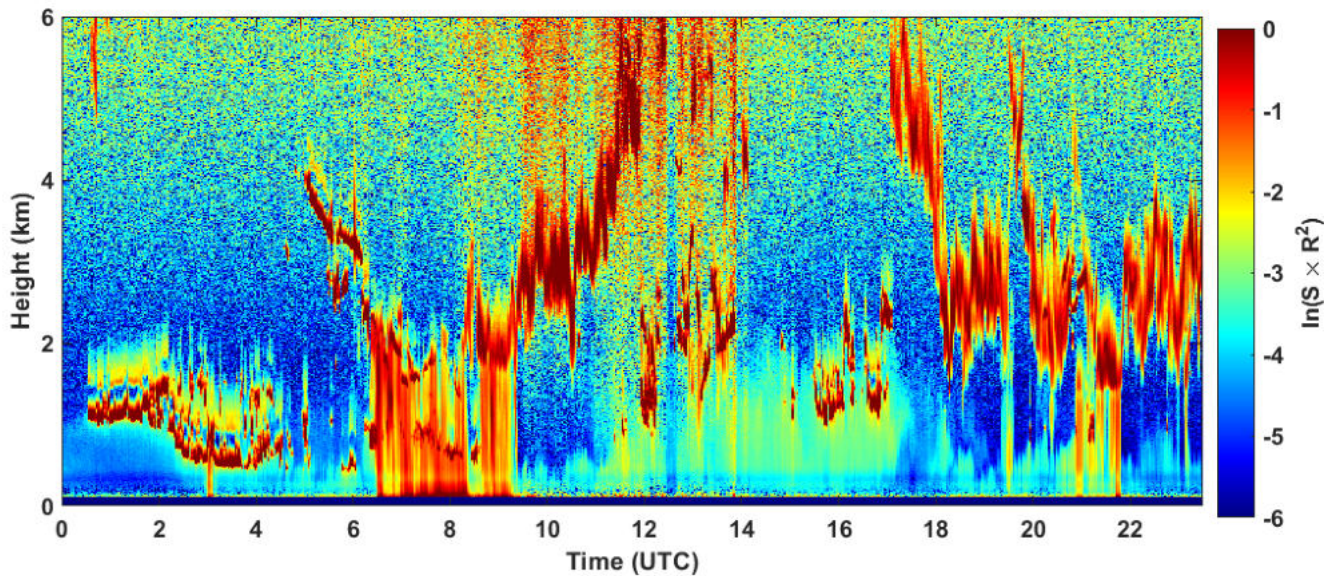
2024-12-08 RCS quick look CHM15k - ILVA LIDAR2 PARCHI
