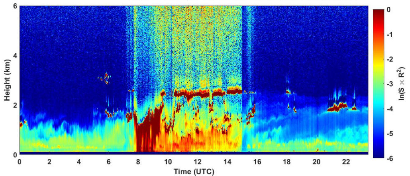
2024-12-02 RCS quick look CHM15k - ILVA LIDAR3 AGGLOMERATO
