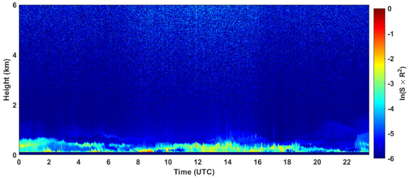
2024-12-18 RCS quick look CHM15k - ILVA LIDAR3 AGGLOMERATO
