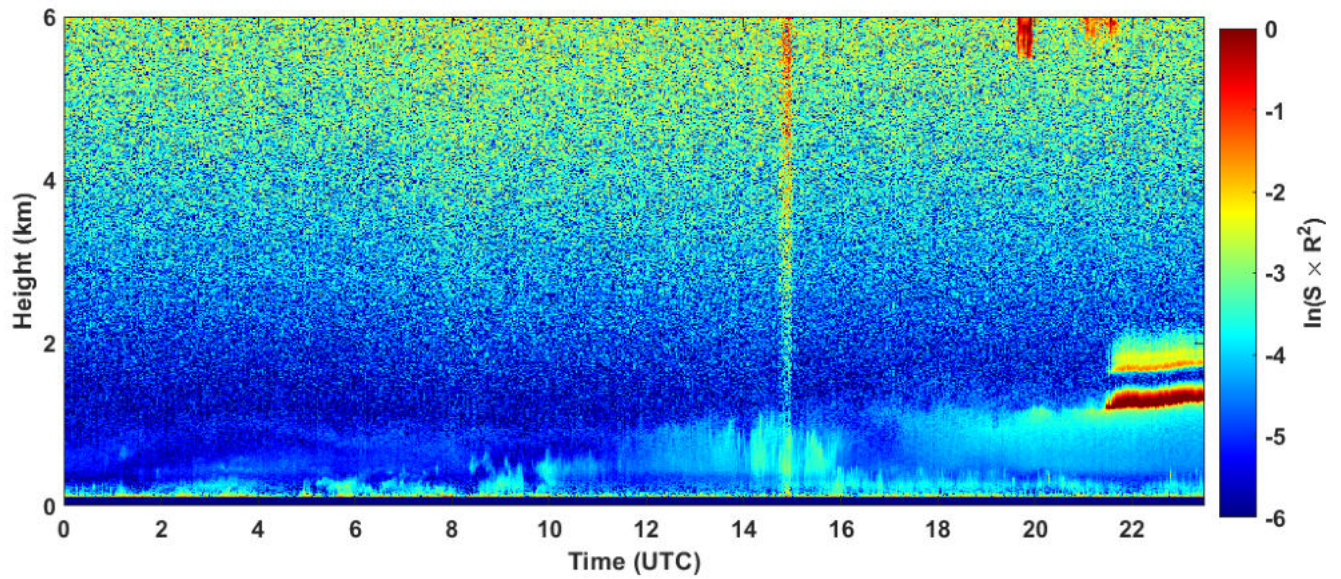
2024-12-18 RCS quick look CHM15k - ILVA LIDAR2 PARCHI
