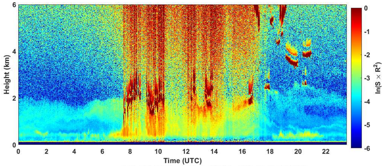
2023-06-14 RCS quick look CHM15k - ILVA LIDAR2 PARCHI
