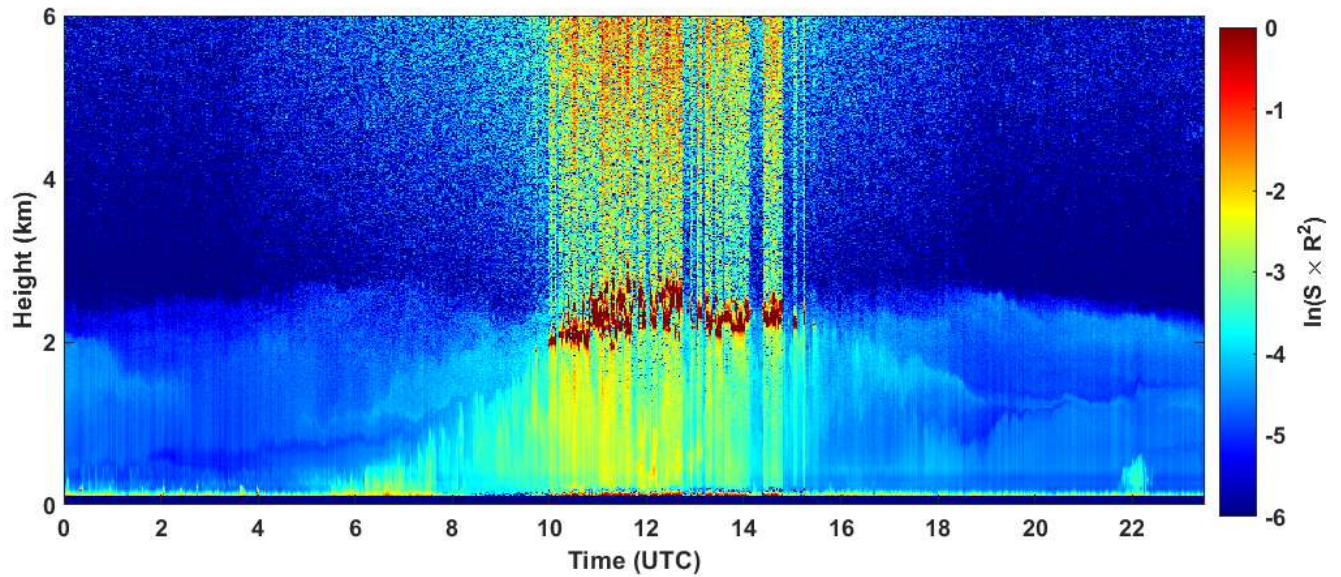
2023-06-28 RCS quick look CHM15k - ILVA LIDAR3 AGGLOMERATO
