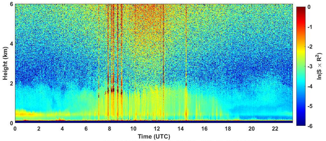
2023-06-18 RCS quick look CHM15k - ILVA LIDAR2 PARCHI
