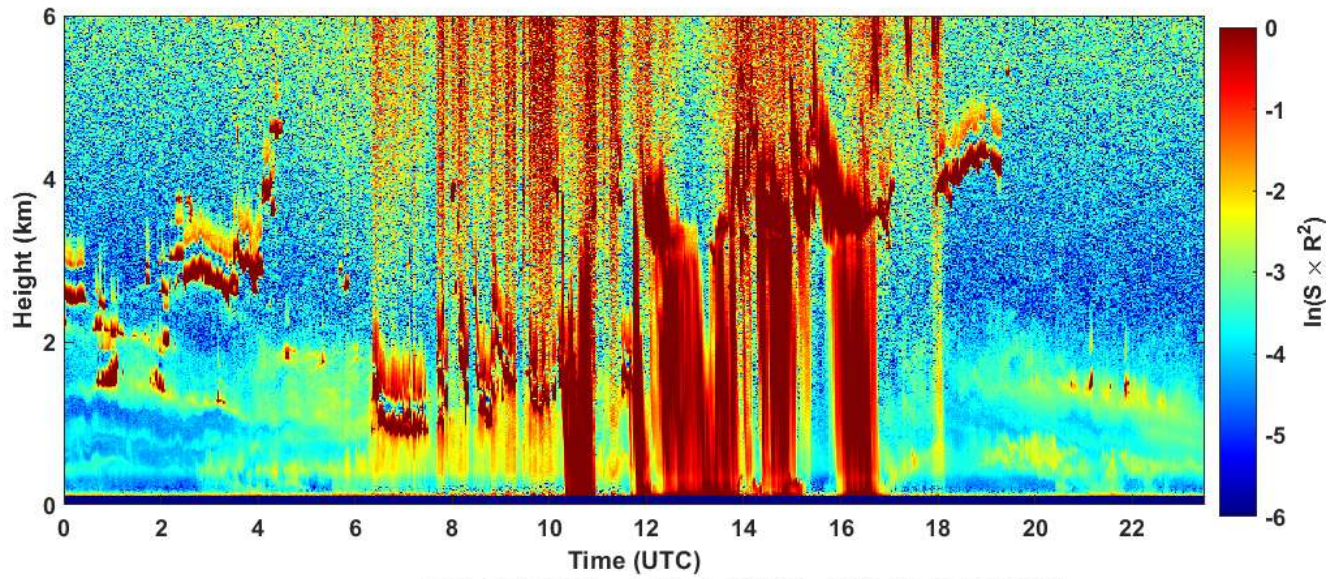
2023-06-12 RCS quick look CHM15k - ILVA LIDAR2 PARCHI
