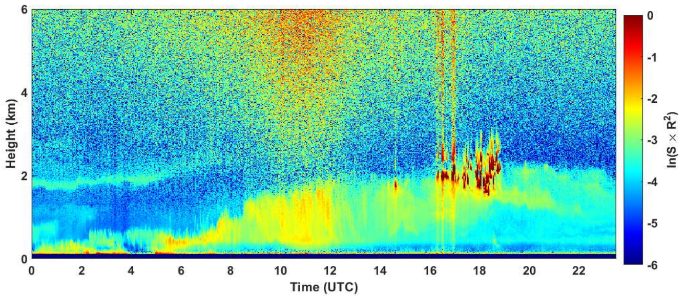
2023-06-08 RCS quick look CHM15k - ILVA LIDAR2 PARCHI
