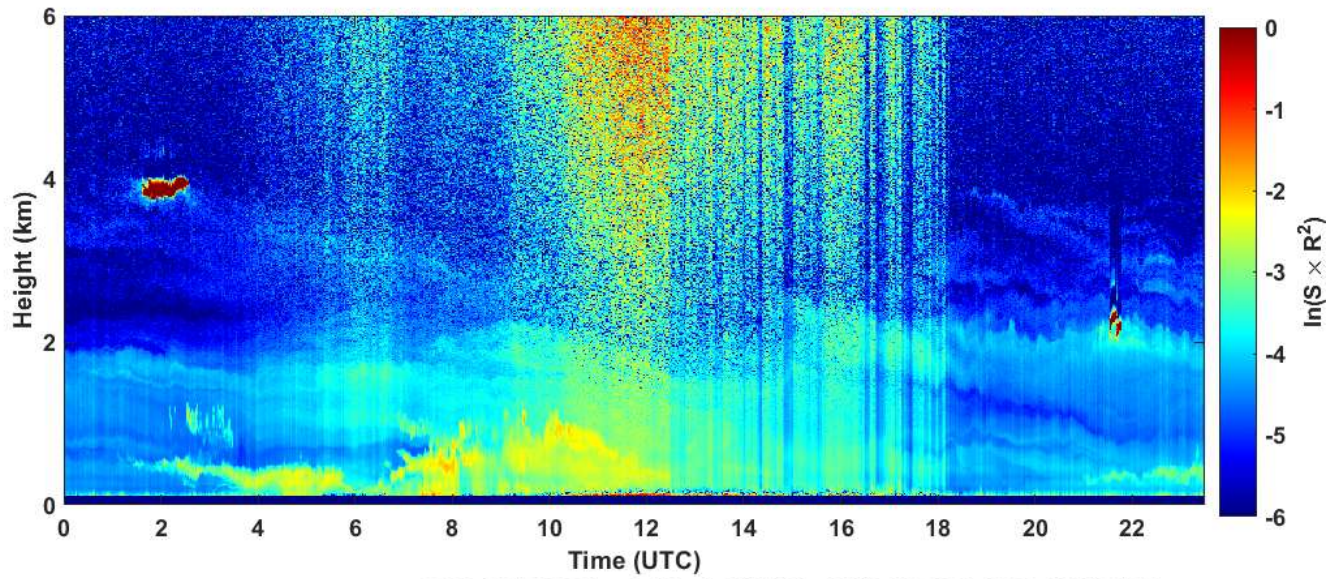
2023-06-10 RCS quick look CHM15k - ILVA LIDAR3 AGGLOMERATO
