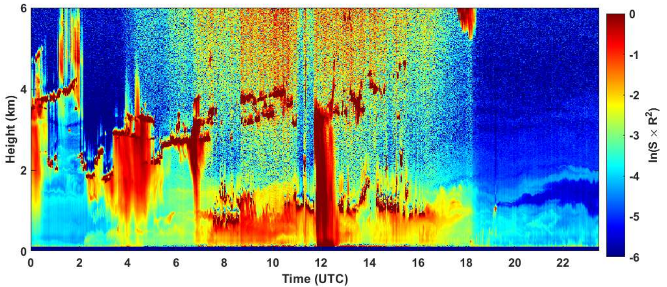
2023-06-08 RCS quick look CHM15k - ILVA LIDAR3 AGGLOMERATO
