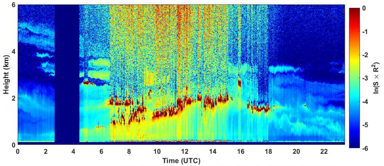
2023-06-30 RCS quick look CHM15k - ILVA LIDAR3 AGGLOMERATO
