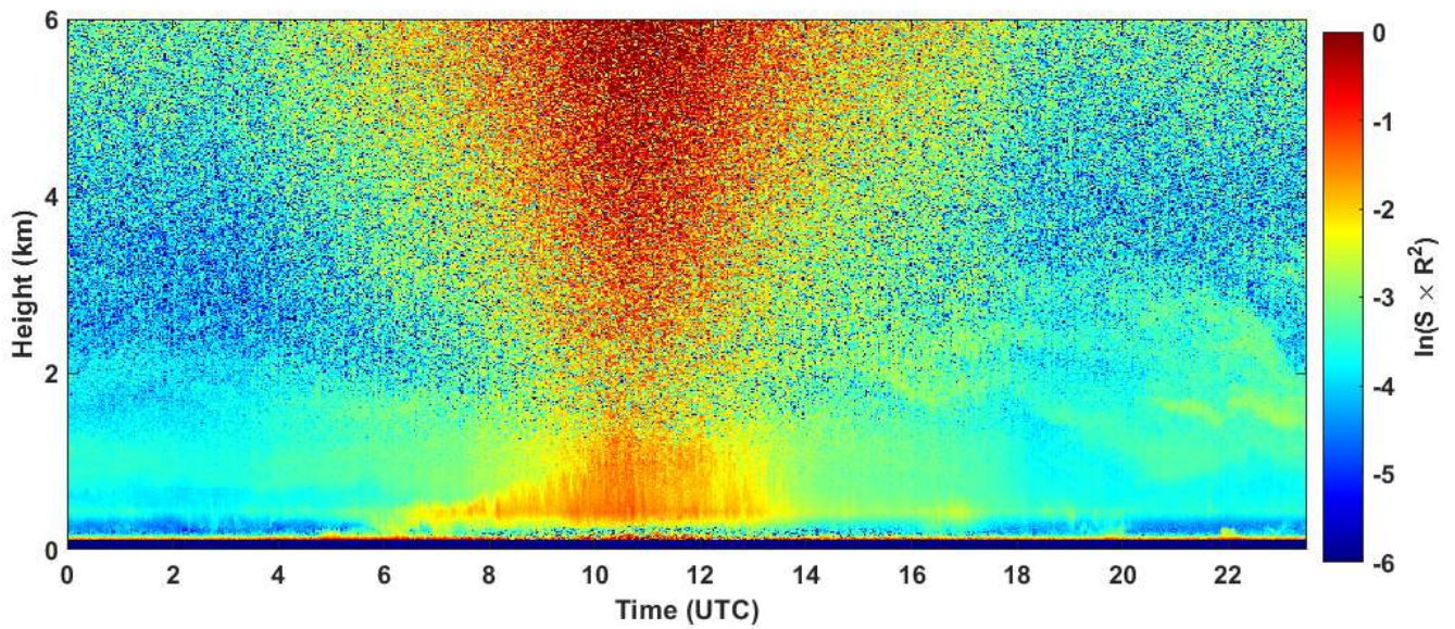
2023-06-22 RCS quick look CHM15k - ILVA LIDAR2 PARCHI
