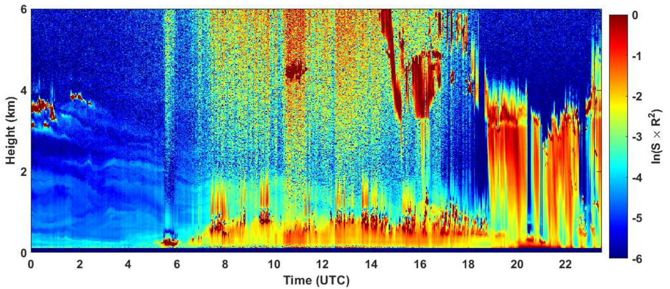
2023-06-14 RCS quick look CHM15k - ILVA LIDAR3 AGGLOMERATO
