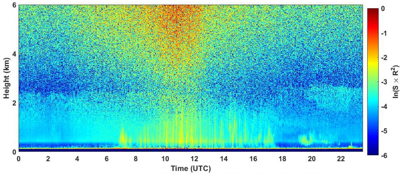
2023-06-20 RCS quick look CHM15k - ILVA LIDAR2 PARCHI
