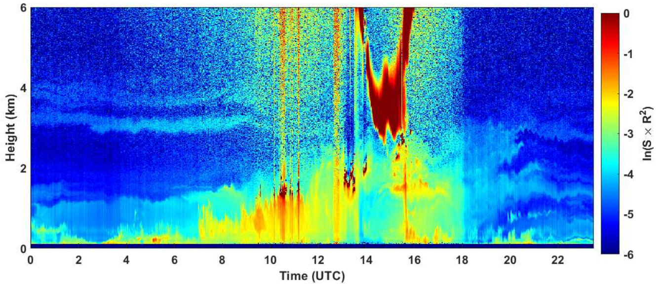
2023-06-02 RCS quick look CHM15k - ILVA LIDAR3 AGGLOMERATO
