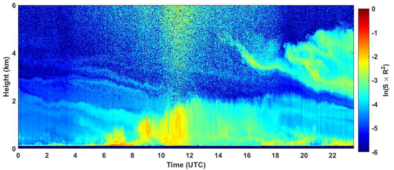
2023-06-20 RCS quick look CHM15k - ILVA LIDAR3 AGGLOMERATO
