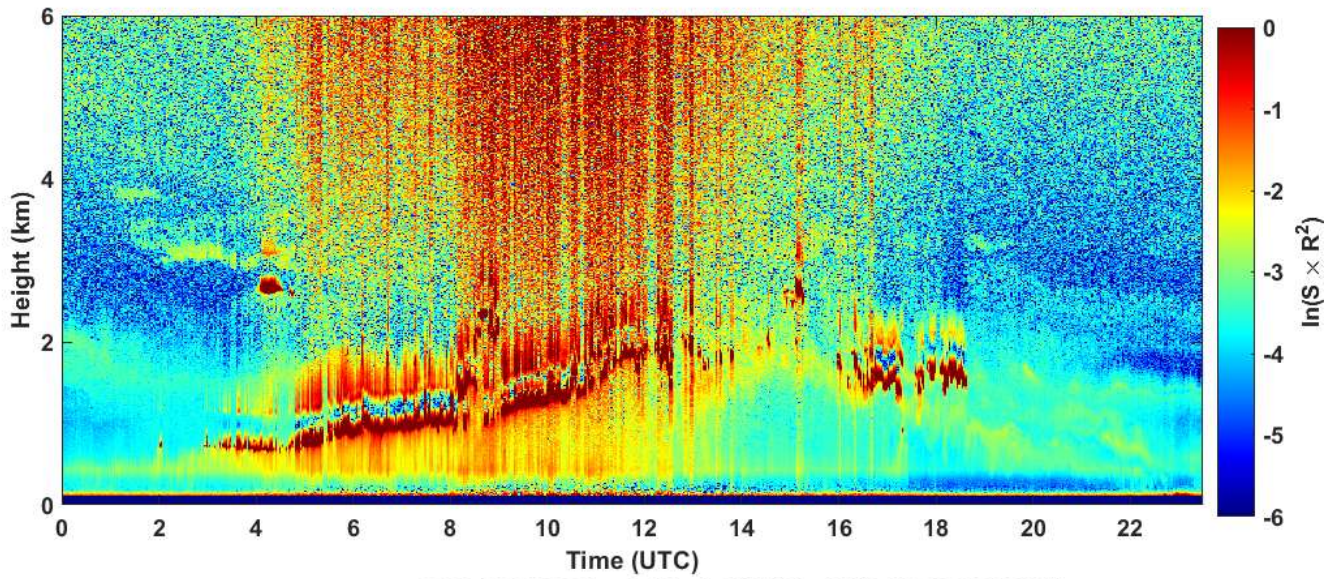
2023-06-30 RCS quick look CHM15k - ILVA LIDAR2 PARCHI
