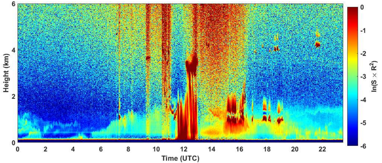
2023-06-02 RCS quick look CHM15k - ILVA LIDAR2 PARCHI
