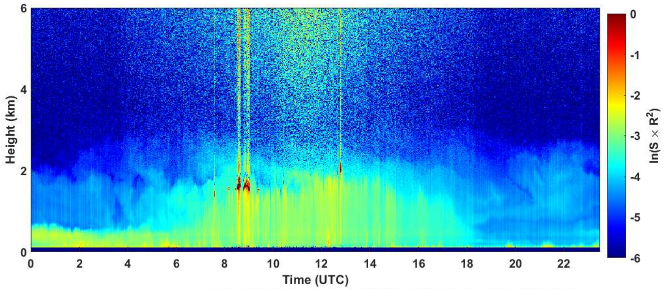
2023-06-18 RCS quick look CHM15k - ILVA LIDAR3 AGGLOMERATO
