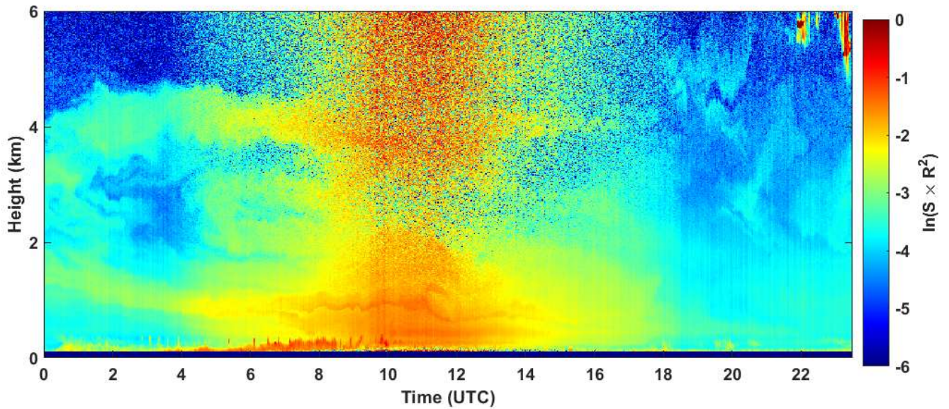
2023-06-24 RCS quick look CHM15k - ILVA LIDAR3 AGGLOMERATO
