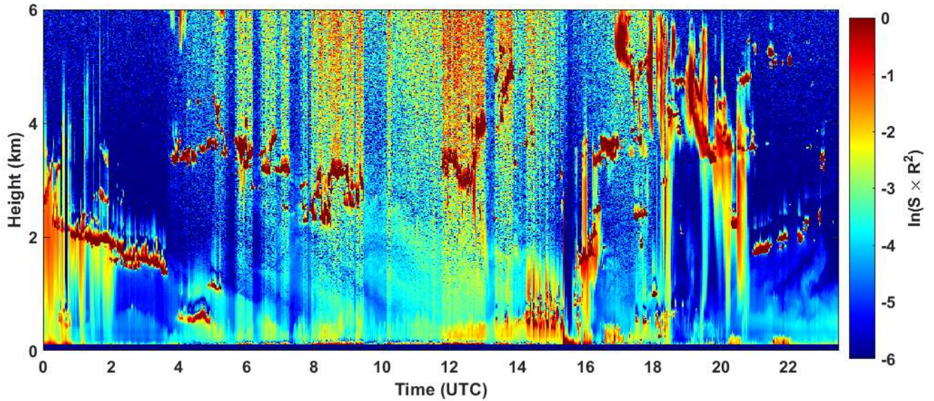
2023-06-16 RCS quick look CHM15k - ILVA LIDAR3 AGGLOMERATO
