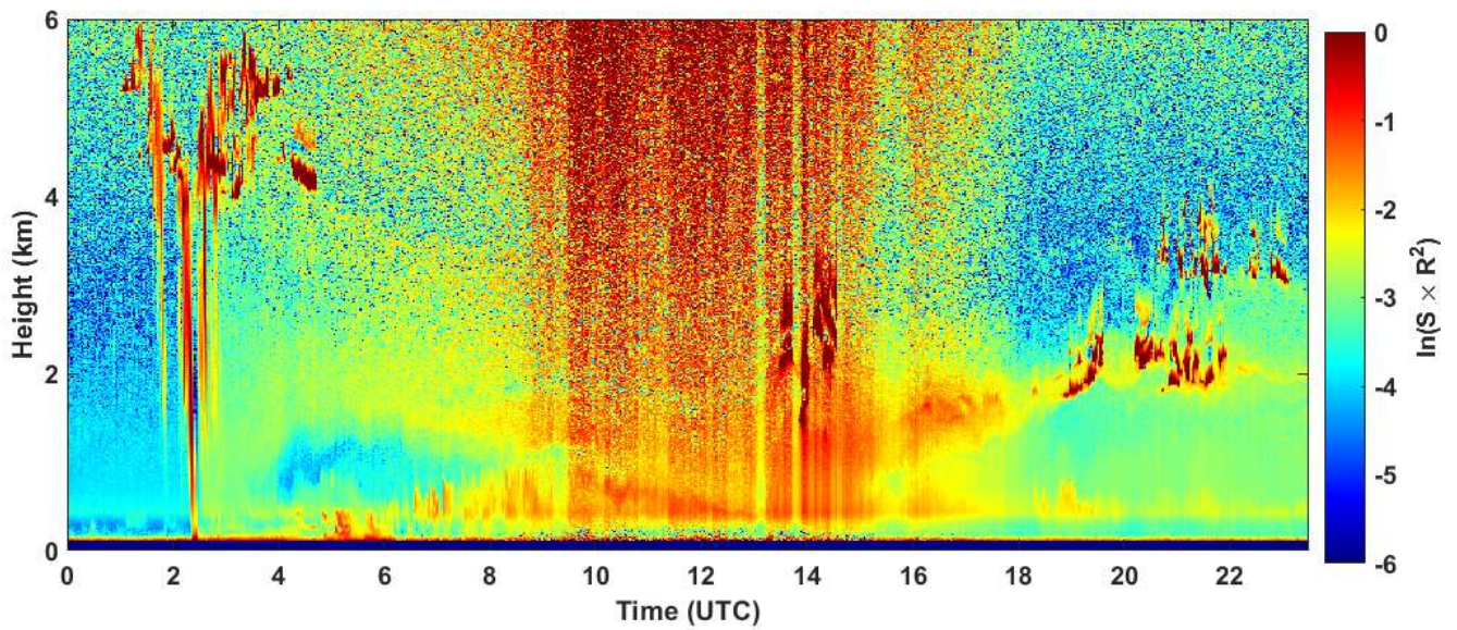
2023-06-24 RCS quick look CHM15k - ILVA LIDAR2 PARCHI
