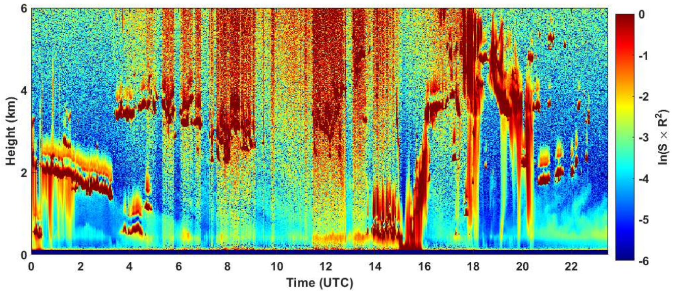
2023-06-16 RCS quick look CHM15k - ILVA LIDAR2 PARCHI
