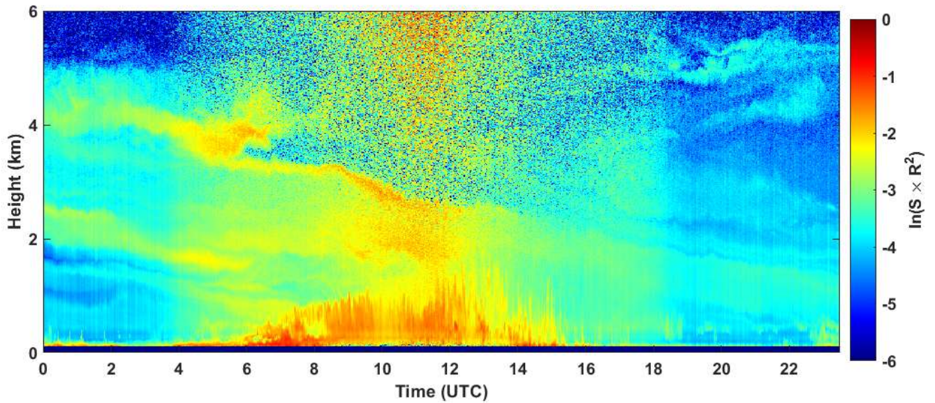
2023-06-22 RCS quick look CHM15k - ILVA LIDAR3 AGGLOMERATO
