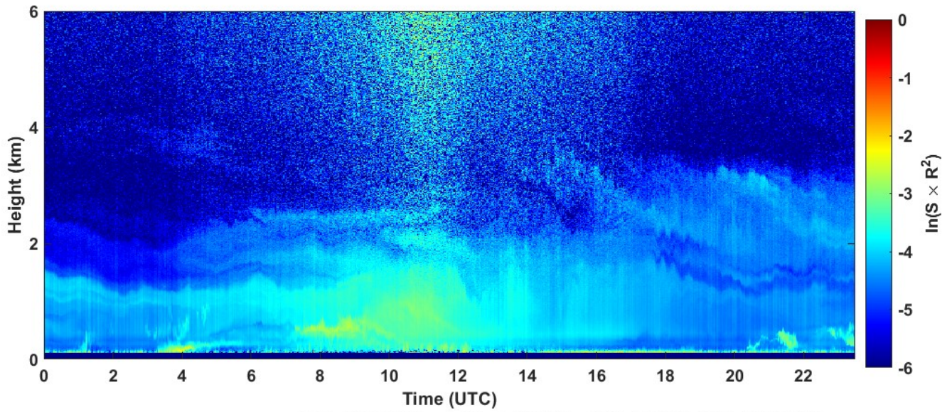
2022-07-30 RCS quick look CHM15k - ILVA LIDAR3 AGGLOMERATO
