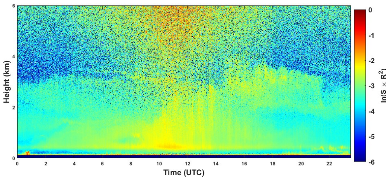
2022-07-24 RCS quick look CHM15k - ILVA LIDAR2 PARCHI
