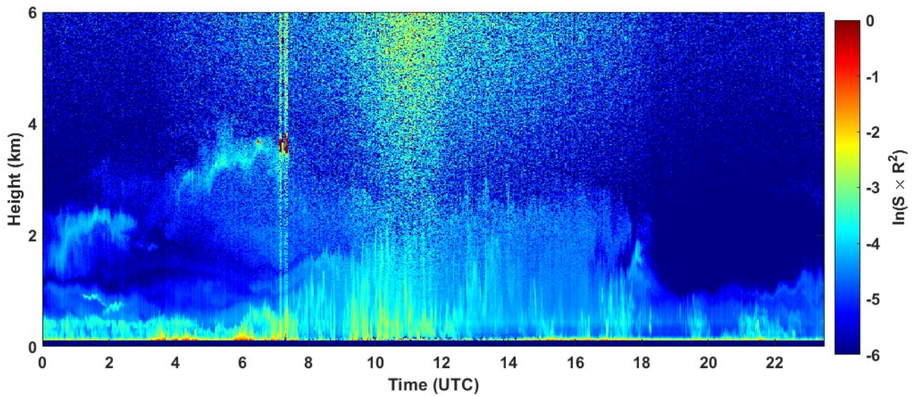
2022-07-04 RCS quick look CHM15k - ILVA LIDAR3 AGGLOMERATO
