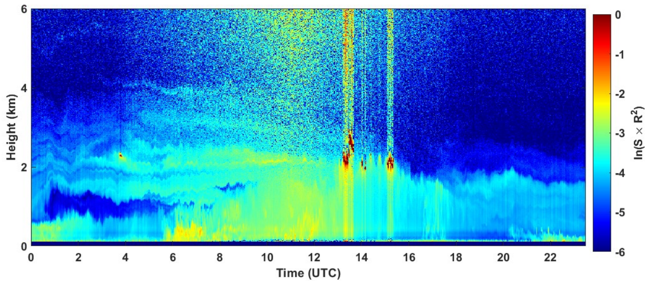
2022-07-28 RCS quick look CHM15k - ILVA LIDAR3 AGGLOMERATO
