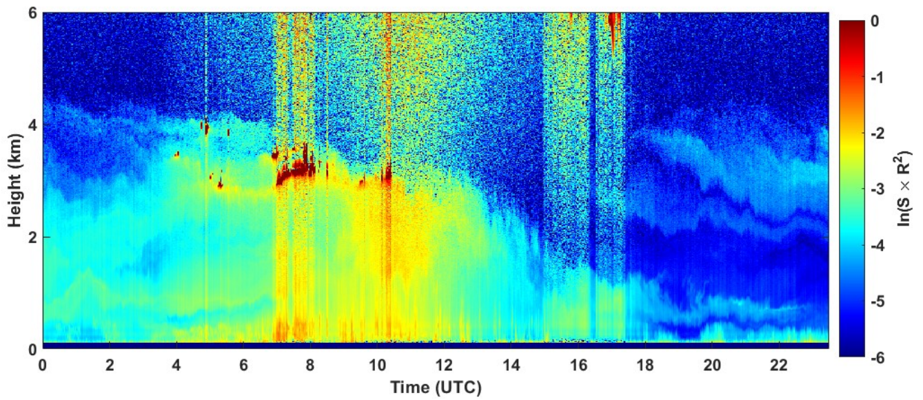
2022-07-06 RCS quick look CHM15k - ILVA LIDAR3 AGGLOMERATO
