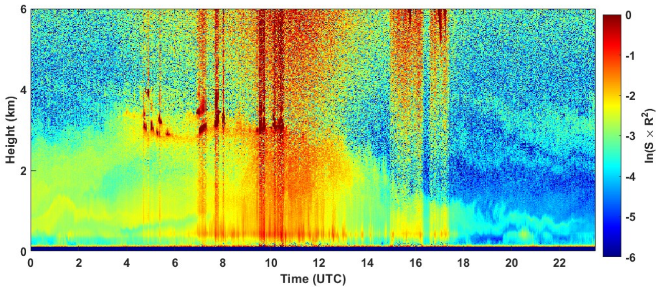
2022-07-06 RCS quick look CHM15k - ILVA LIDAR2 PARCHI
