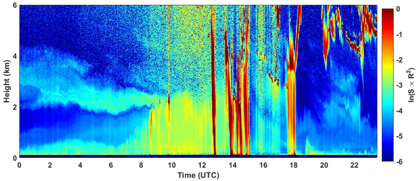
2022-07-08 RCS quick look CHM15k - ILVA LIDAR3 AGGLOMERATO
