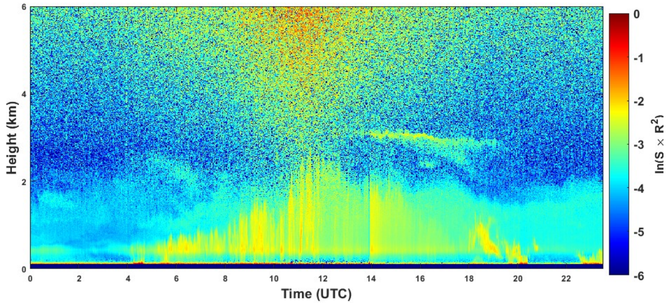
2022-07-20 RCS quick look CHM15k - ILVA LIDAR2 PARCHI
