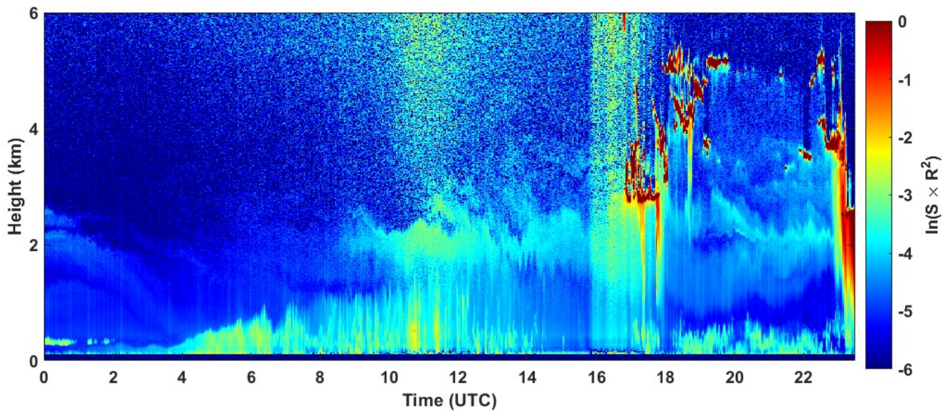
2022-07-12 RCS quick look CHM15k - ILVA LIDAR3 AGGLOMERATO
