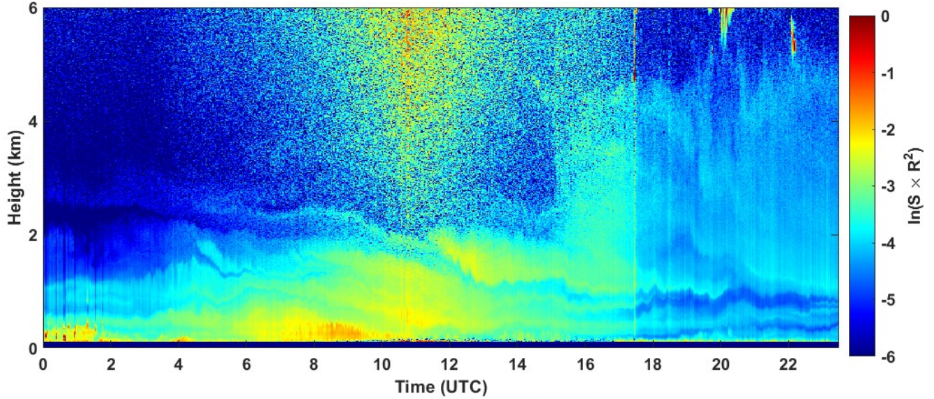
2022-07-02 RCS quick look CHM15k - ILVA LIDAR3 AGGLOMERATO
