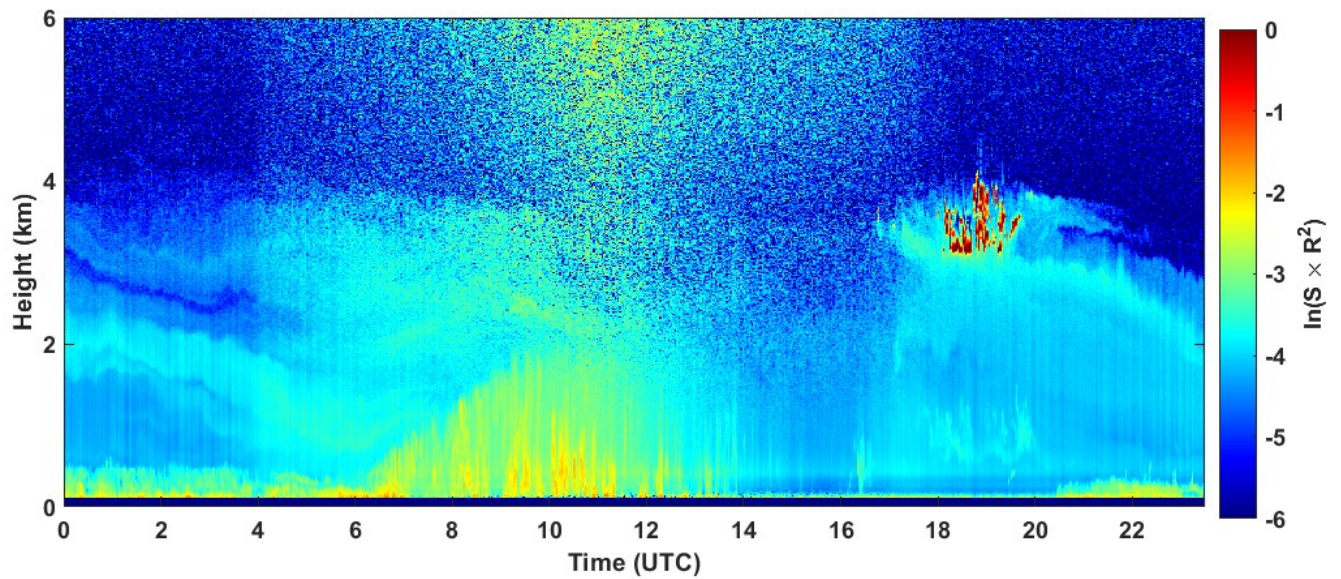
2022-07-26 RCS quick look CHM15k - ILVA LIDAR3 AGGLOMERATO
