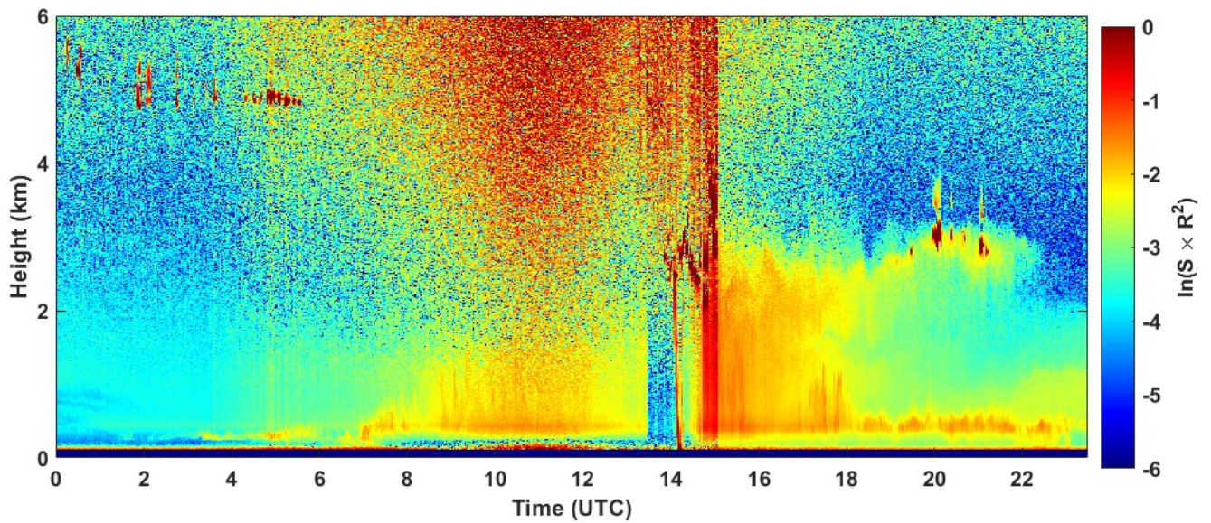
2022-07-02 RCS quick look CHM15k - ILVA LIDAR2 PARCHI
