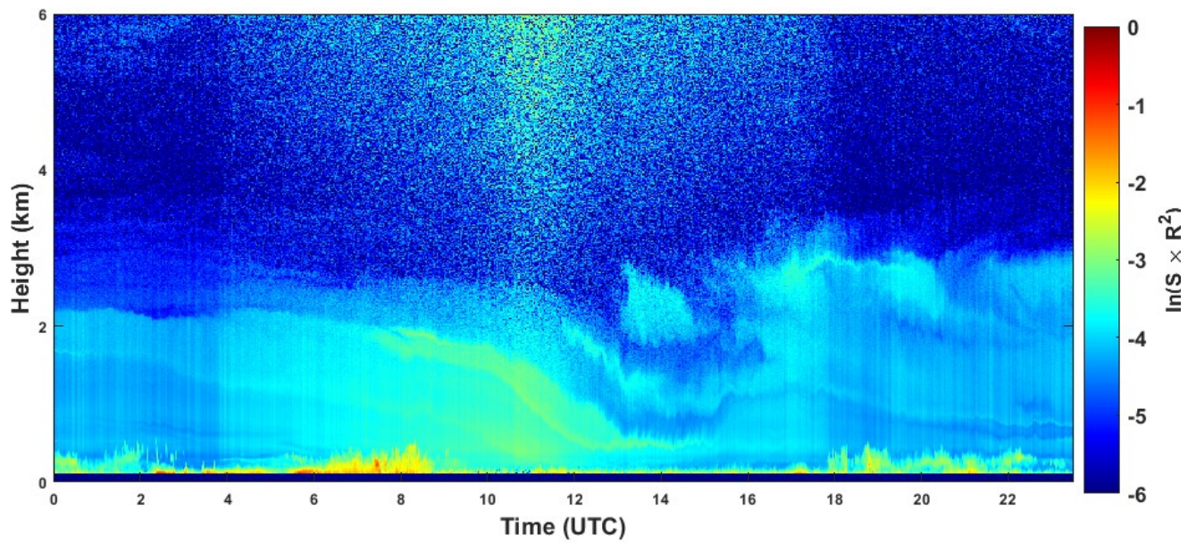
2022-07-24 RCS quick look CHM15k - ILVA LIDAR3 AGGLOMERATO
