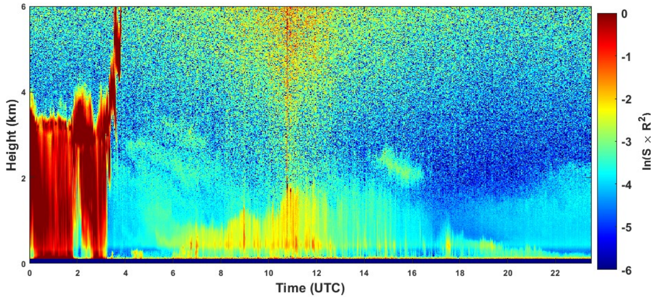
2022-07-14 RCS quick look CHM15k - ILVA LIDAR2 PARCHI
