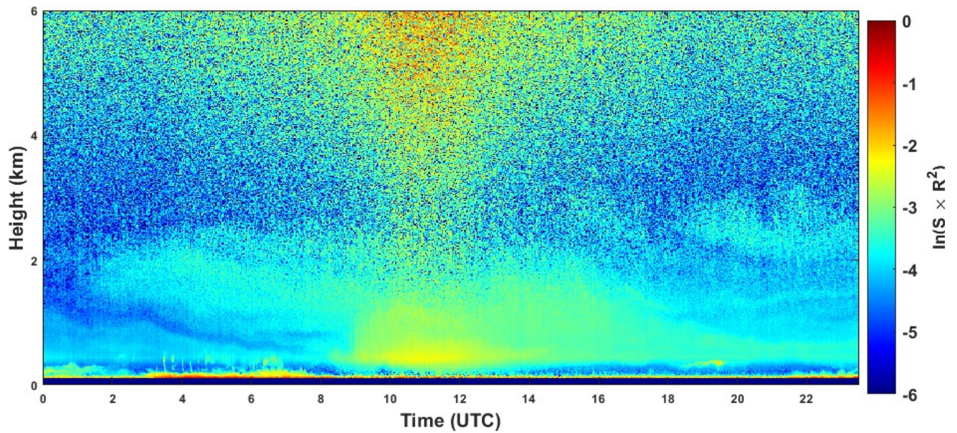
2022-07-16 RCS quick look CHM15k - ILVA LIDAR2 PARCHI
