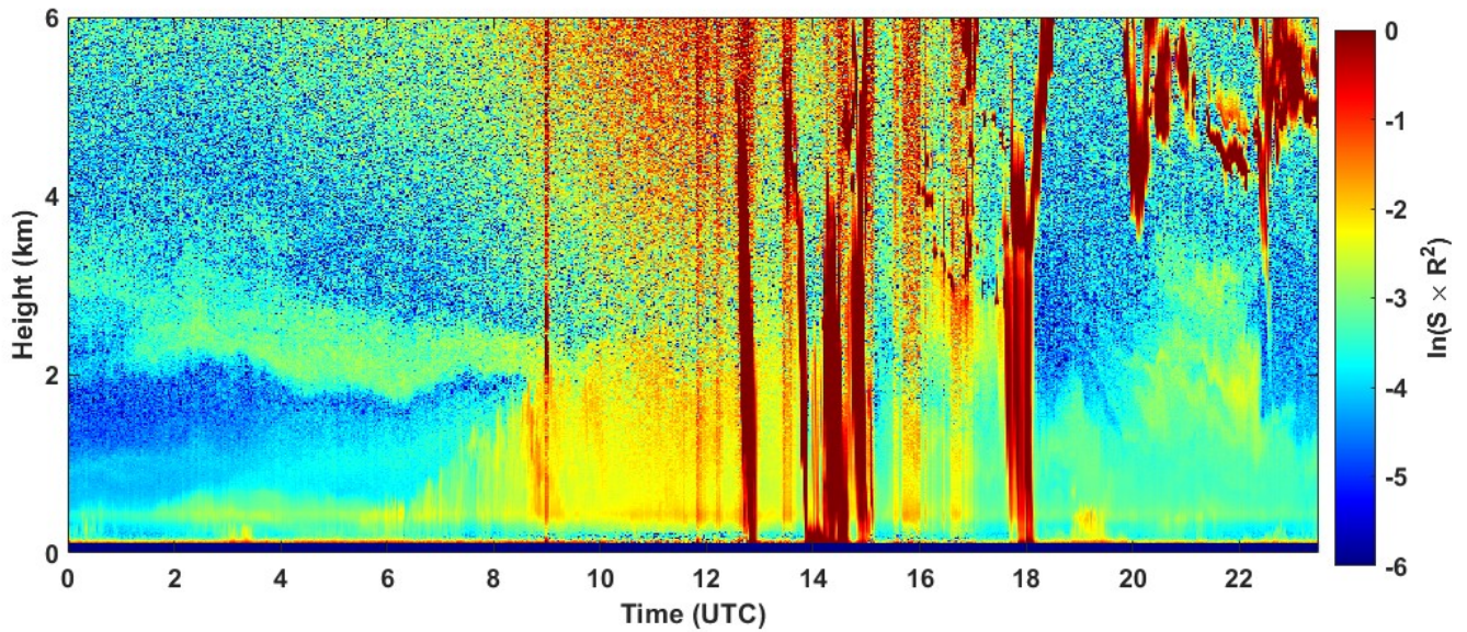
2022-07-08 RCS quick look CHM15k - ILVA LIDAR2 PARCHI
