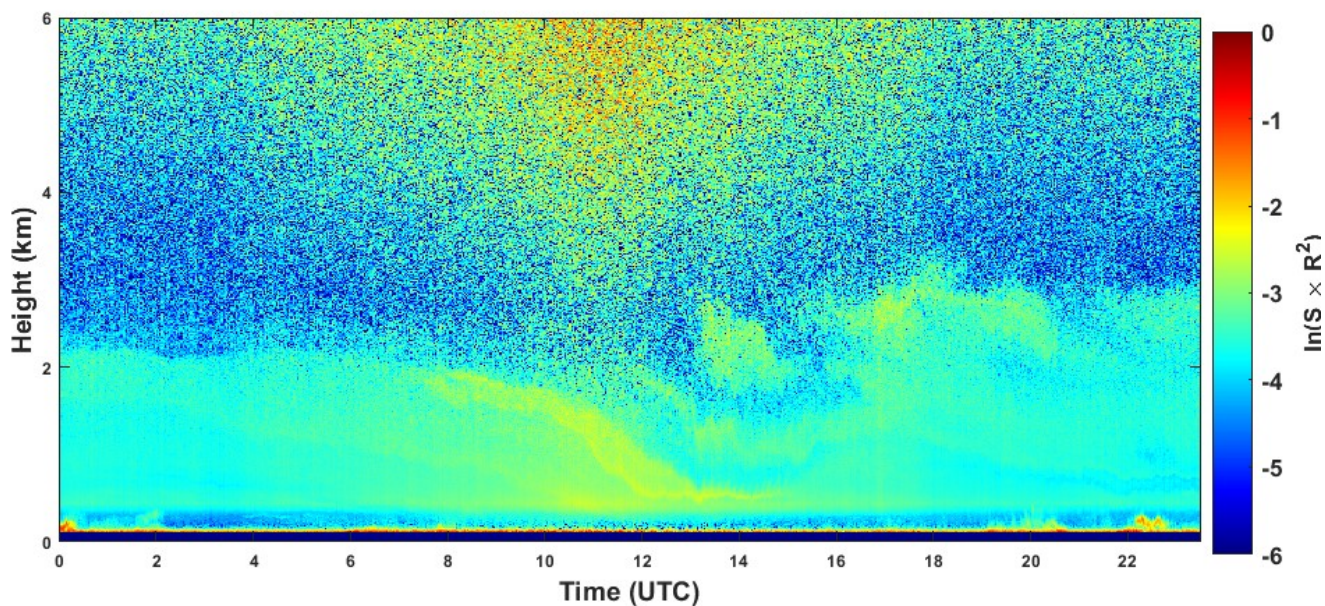
2022-07-24 RCS quick look CHM15k - ILVA LIDAR2 PARCHI
