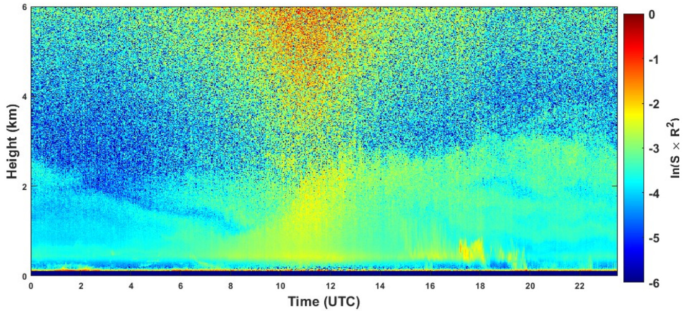
2022-07-18 RCS quick look CHM15k - ILVA LIDAR2 PARCHI
