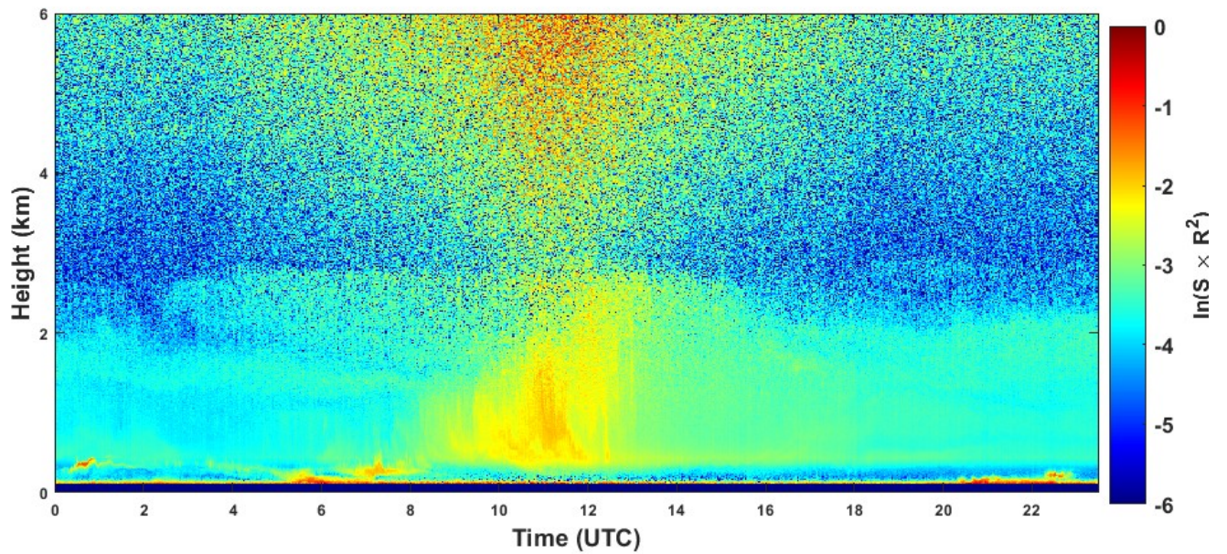
2022-07-22 RCS quick look CHM15k - ILVA LIDAR2 PARCHI
