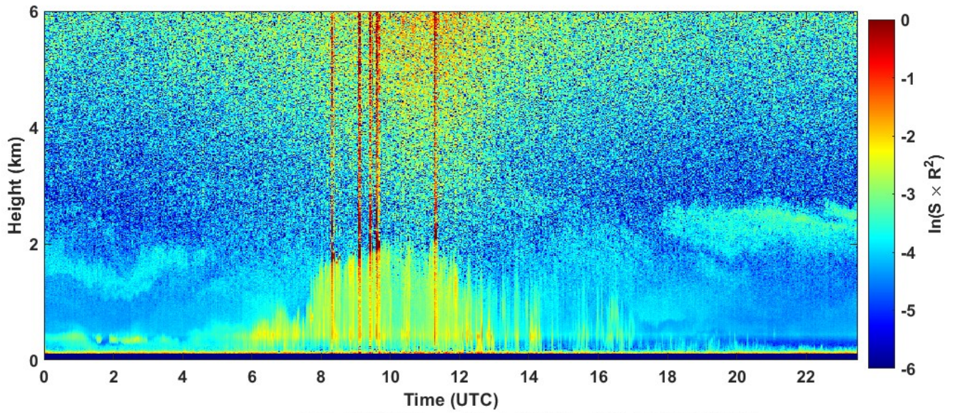
2022-07-12 RCS quick look CHM15k - ILVA LIDAR2 PARCHI
