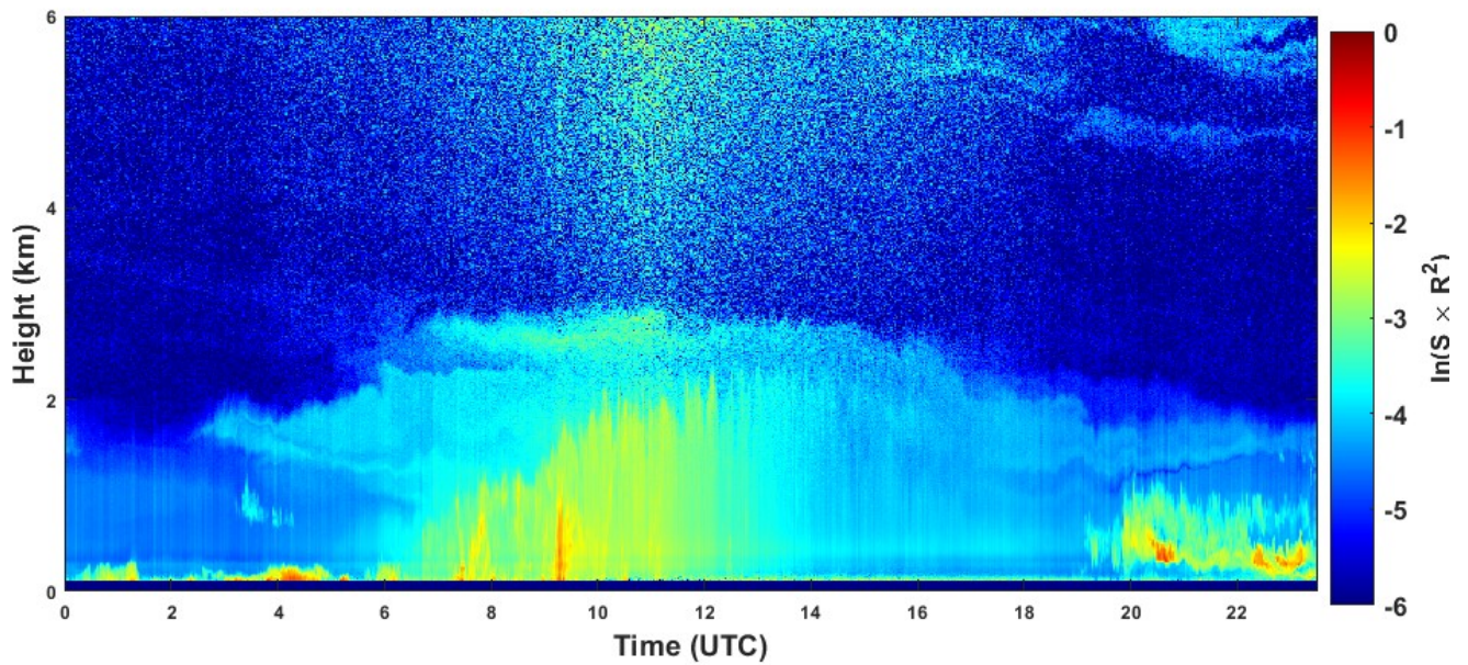
2022-07-20 RCS quick look CHM15k - ILVA LIDAR3 AGGLOMERATO
