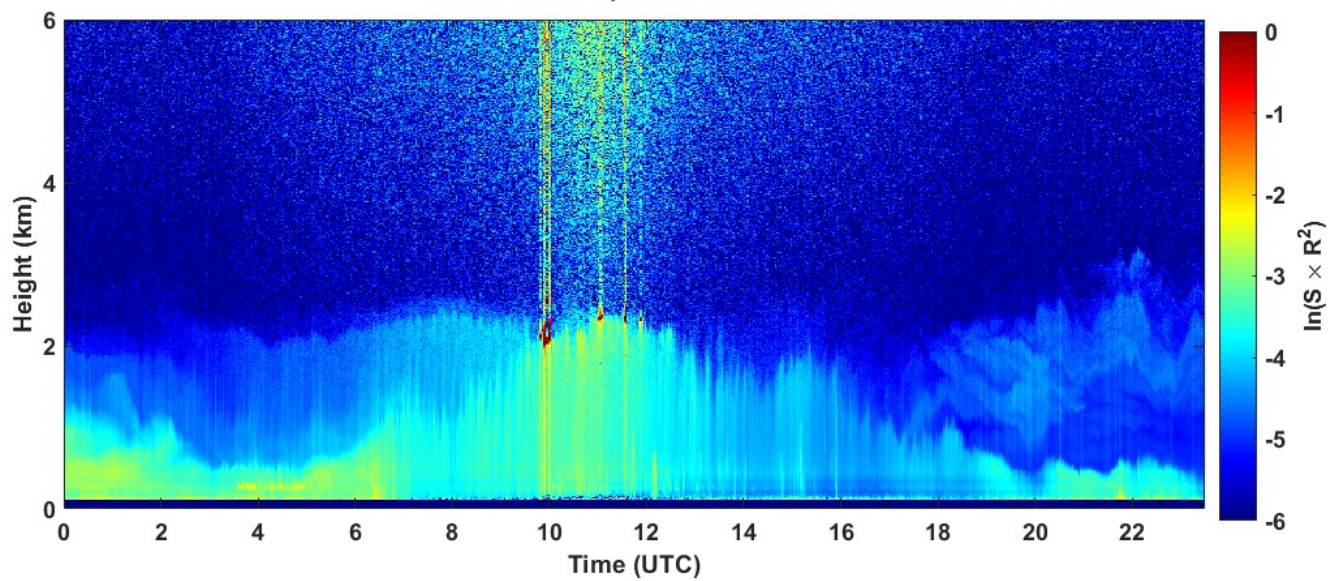
2022-07-10 RCS quick look CHM15k - ILVA LIDAR3 AGGLOMERATO
