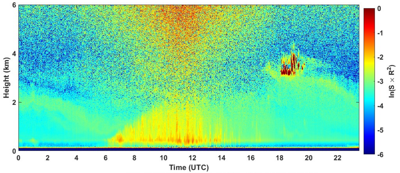
2022-07-26 RCS quick look CHM15k - ILVA LIDAR2 PARCHI
