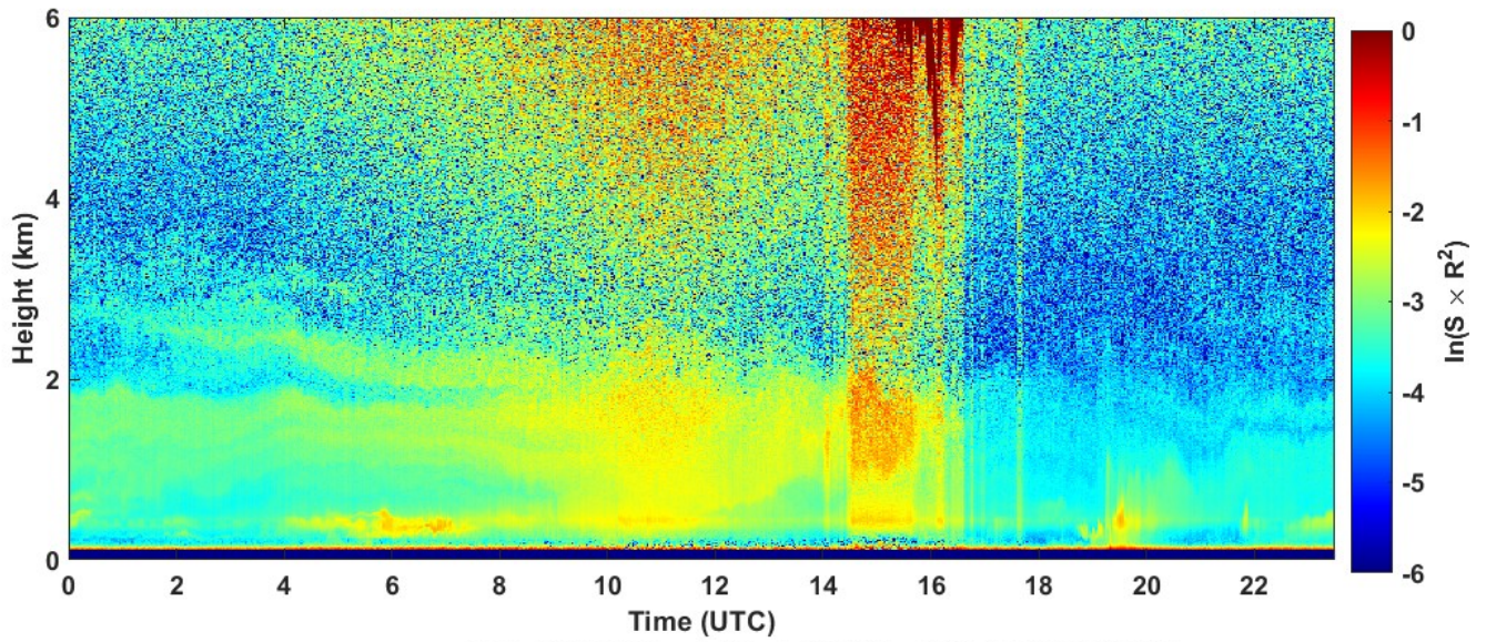
2022-07-28 RCS quick look CHM15k - ILVA LIDAR2 PARCHI
