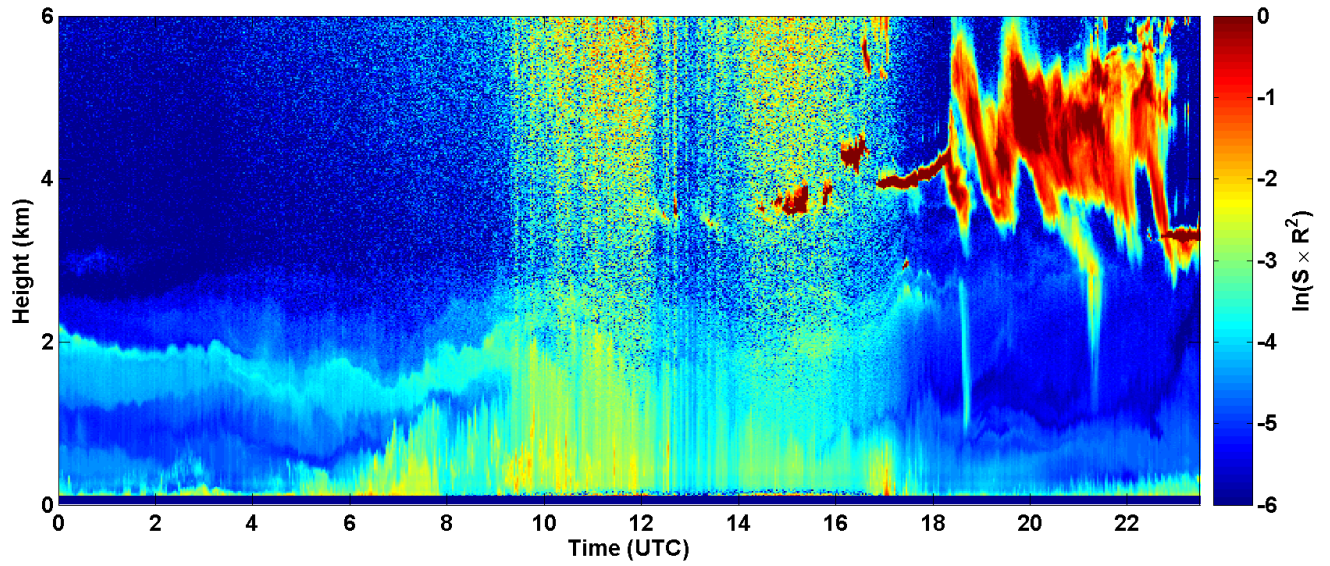
2017-05-16 RCS quick look CHM15k - ILVA LIDAR3 AGGLOMERATO
