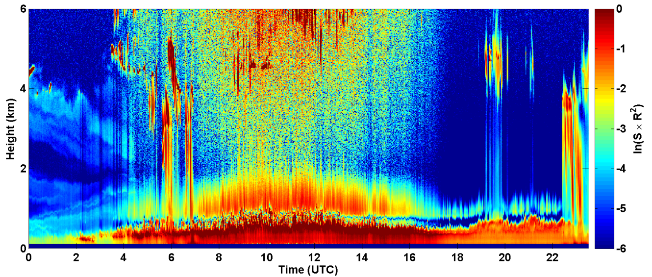
2017-05-12 RCS quick look CHM15k - ILVA LIDAR3 AGGLOMERATO
