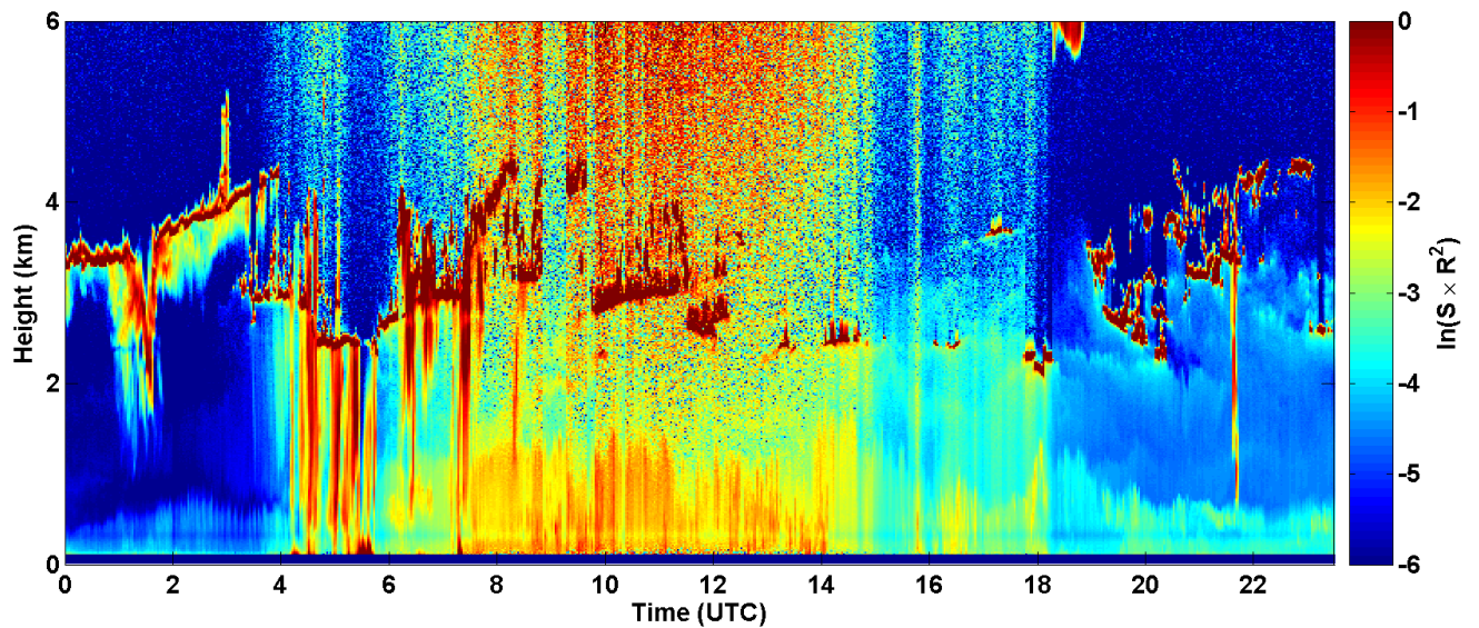
2017-05-16 RCS quick look CHM15k - ILVA LIDAR2 PARCHI
