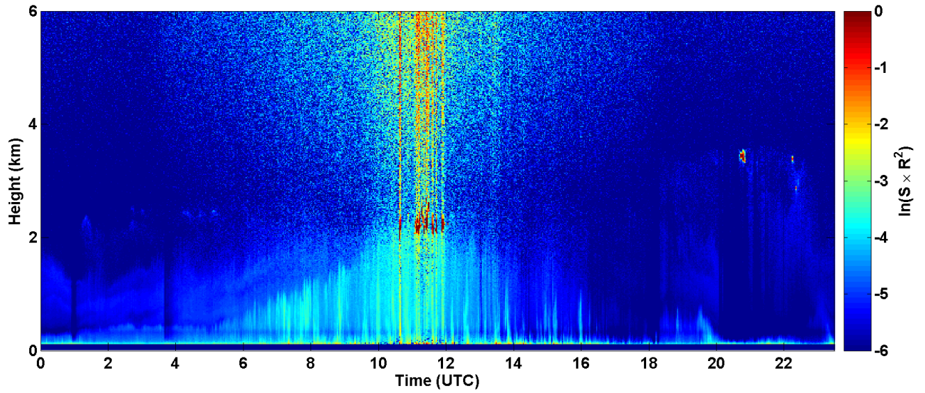
2017-05-28 RCS quick look CHM15k - ILVA LIDAR2 PARCHI
