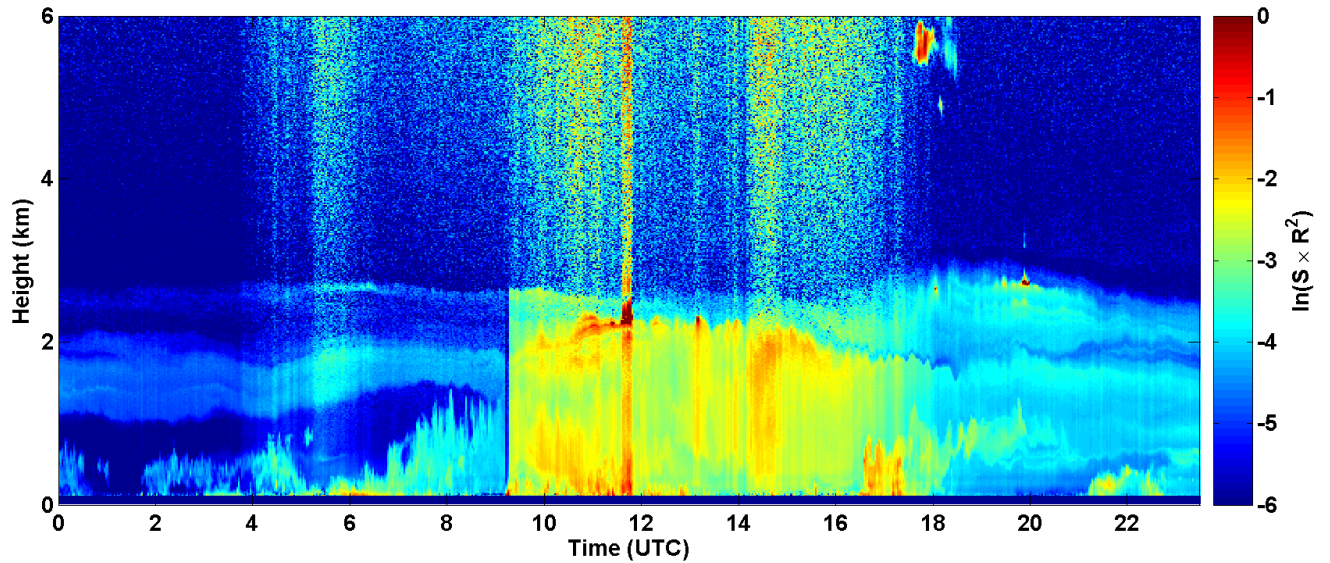
2017-05-04 RCS quick look CHM15k - ILVA LIDAR3 AGGLOMERATO
