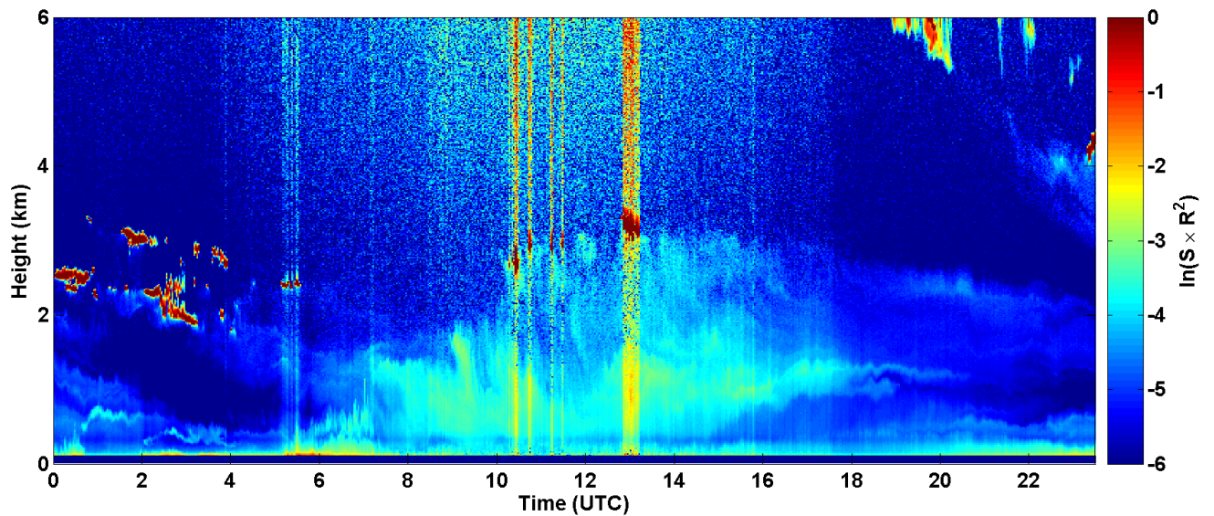
2017-05-10 RCS quick look CHM15k - ILVA LIDAR2 PARCHI
