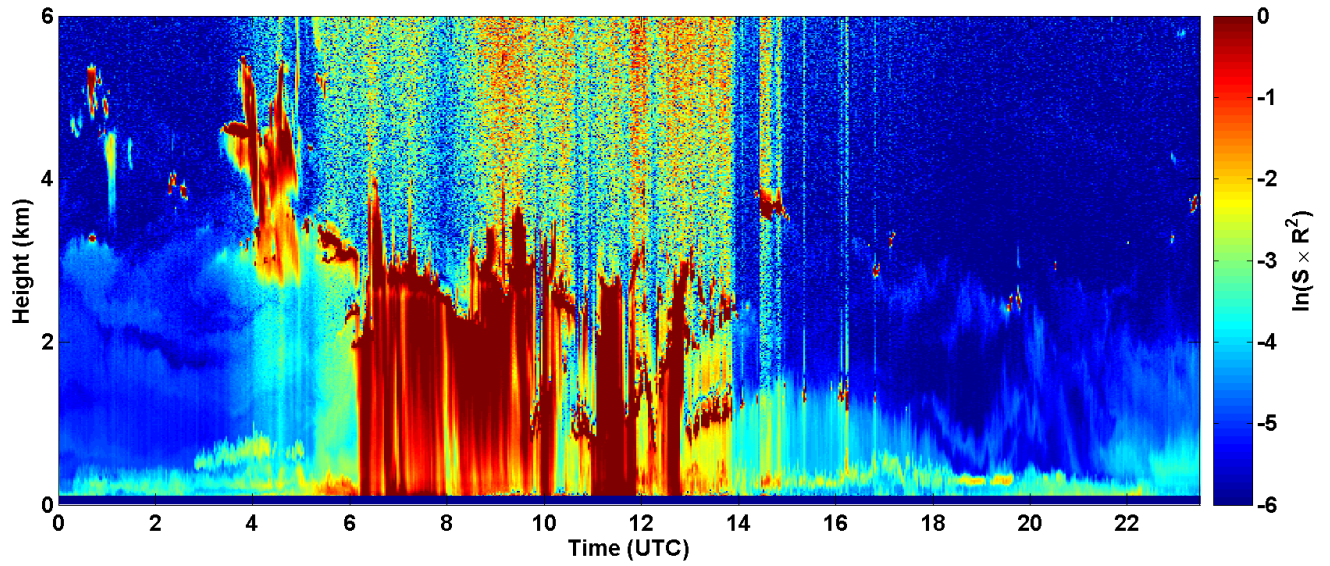
2017-05-26 RCS quick look CHM15k - ILVA LIDAR3 AGGLOMERATO
