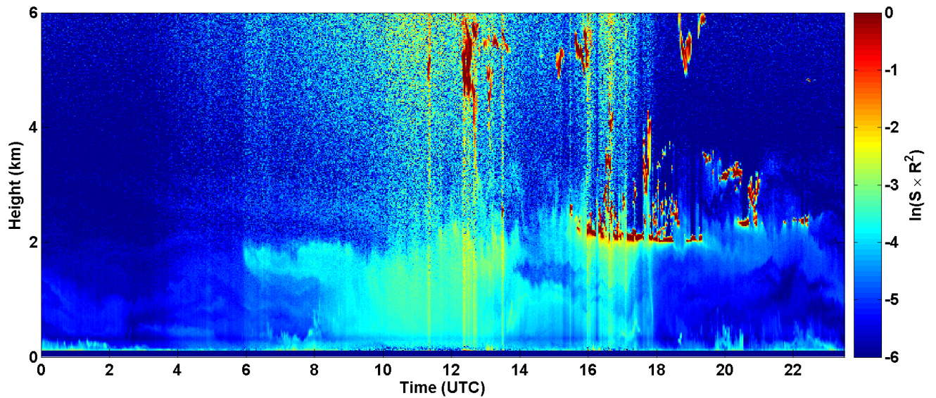
2017-05-24 RCS quick look CHM15k - ILVA LIDAR2 PARCHI
