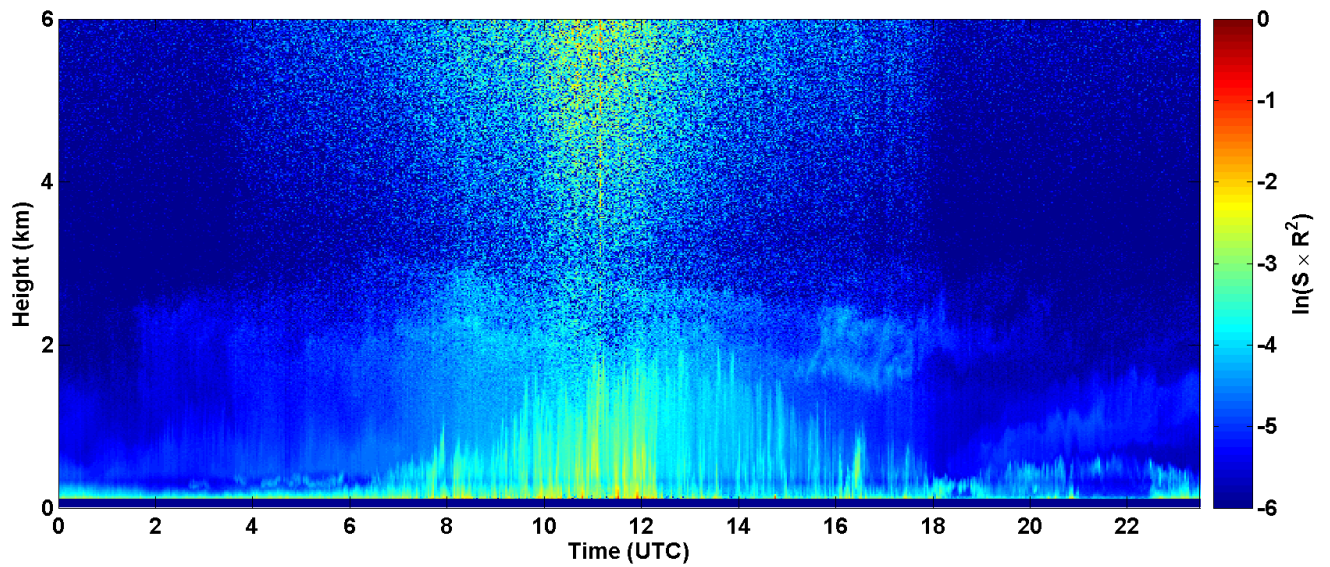
2017-05-22 RCS quick look CHM15k - ILVA LIDAR2 PARCHI
