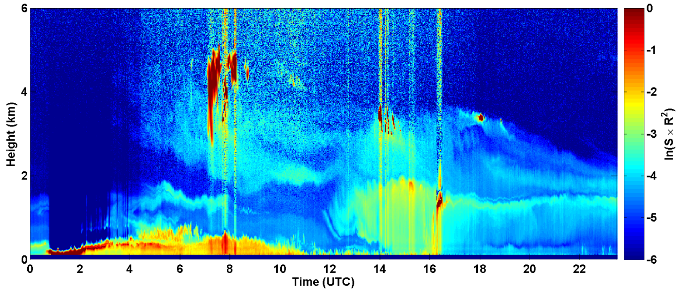
2017-05-06 RCS quick look CHM15k - ILVA LIDAR3 AGGLOMERATO
