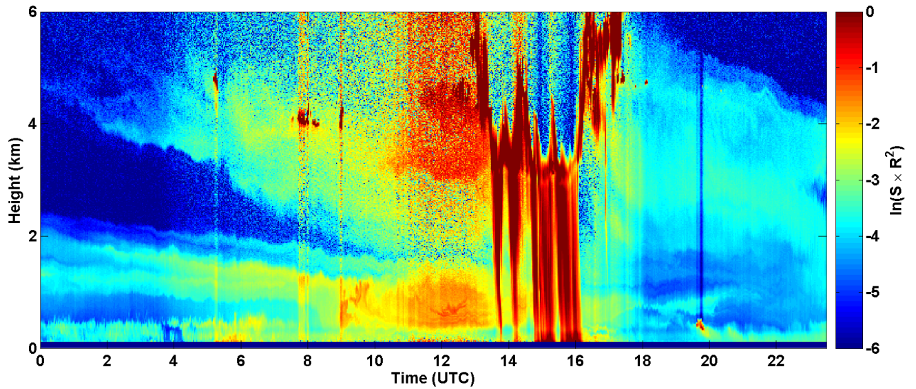
2017-05-06 RCS quick look CHM15k - ILVA LIDAR2 PARCHI
