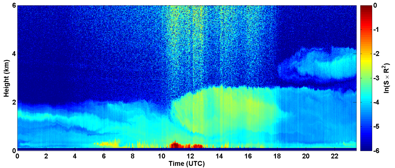
2017-05-20 RCS quick look CHM15k - ILVA LIDAR3 AGGLOMERATO
