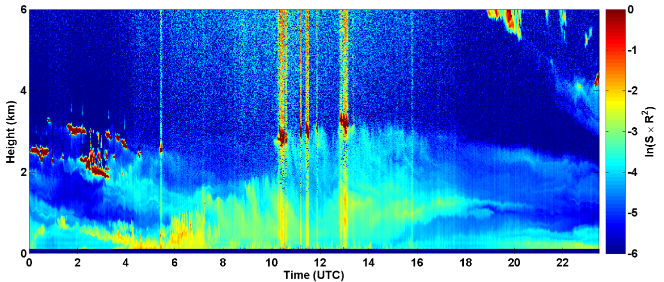
2017-05-10 RCS quick look CHM15k - ILVA LIDAR3 AGGLOMERATO
