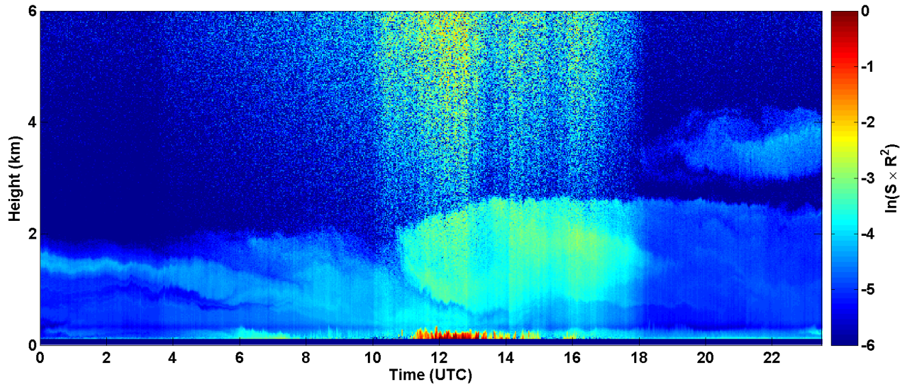
2017-05-20 RCS quick look CHM15k - ILVA LIDAR2 PARCHI
