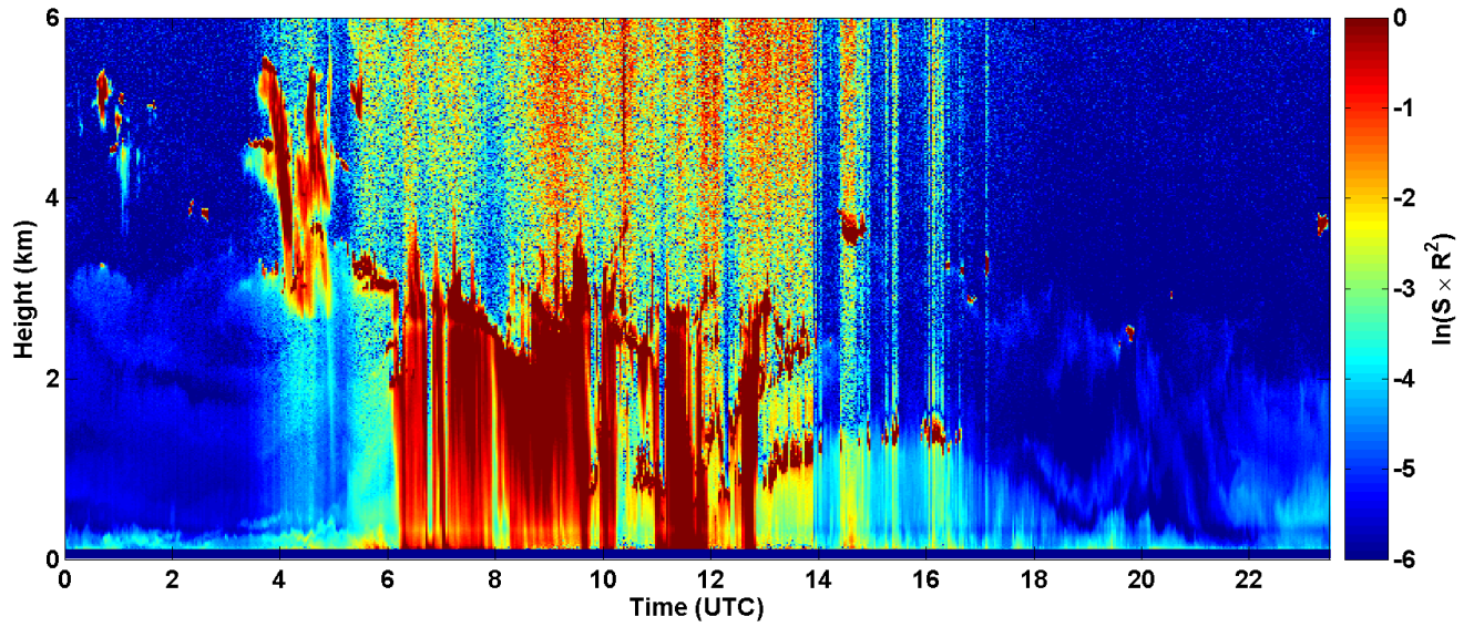
2017-05-26 RCS quick look CHM15k - ILVA LIDAR2 PARCHI
