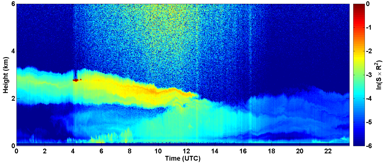
2017-05-02 RCS quick look CHM15k - ILVA LIDAR2 PARCHI
