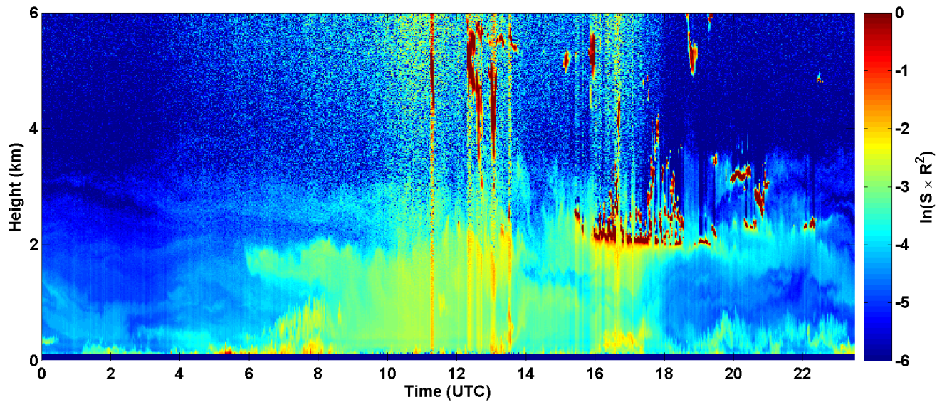
2017-05-24 RCS quick look CHM15k - ILVA LIDAR3 AGGLOMERATO
