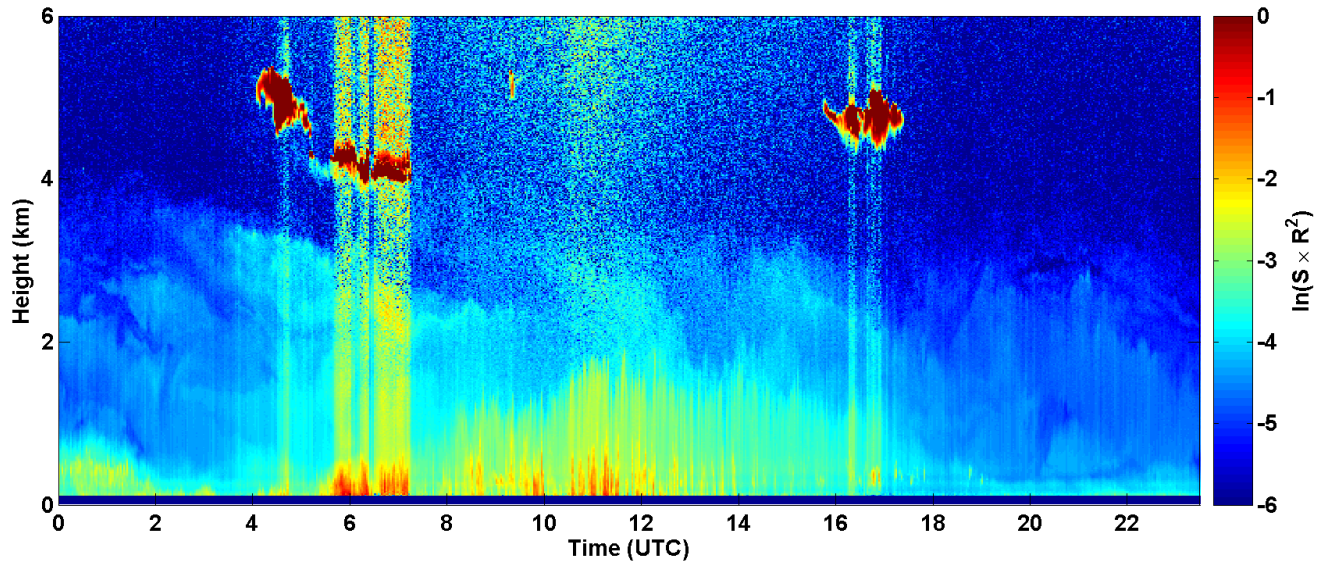
2017-05-18 RCS quick look CHM15k - ILVA LIDAR3 AGGLOMERATO
