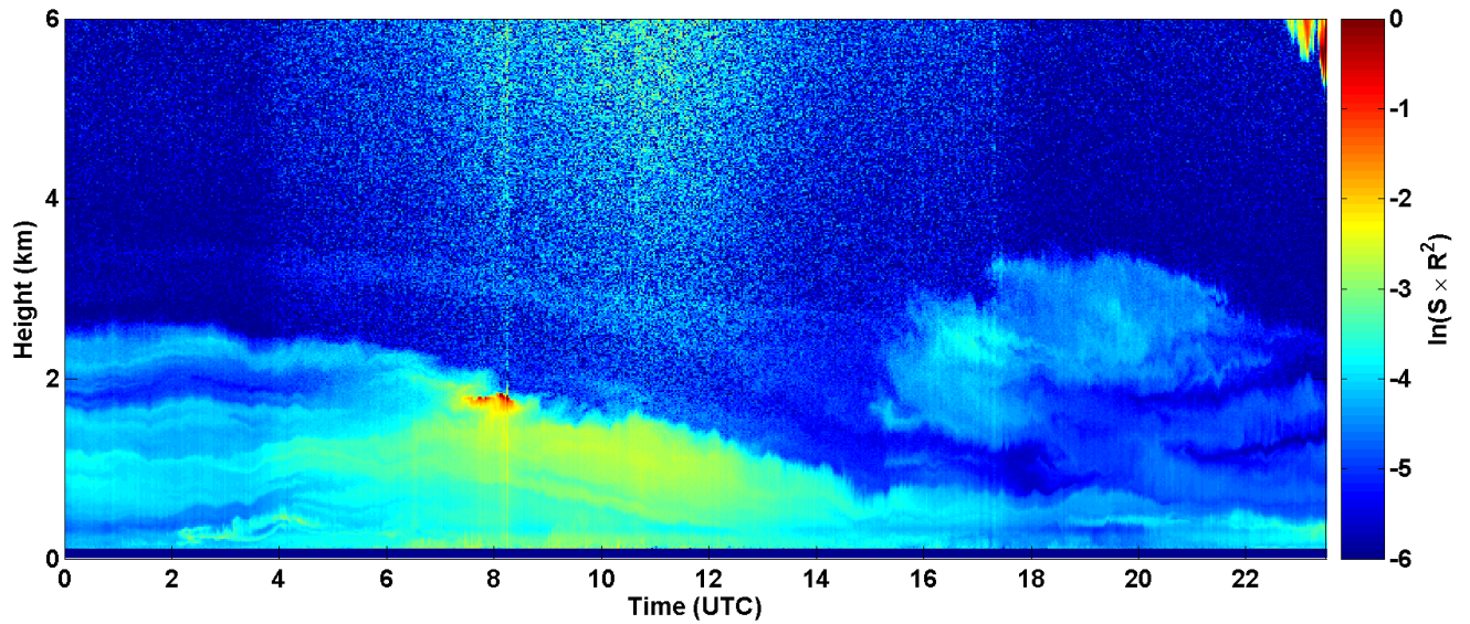
2017-05-04 RCS quick look CHM15k - ILVA LIDAR2 PARCHI
