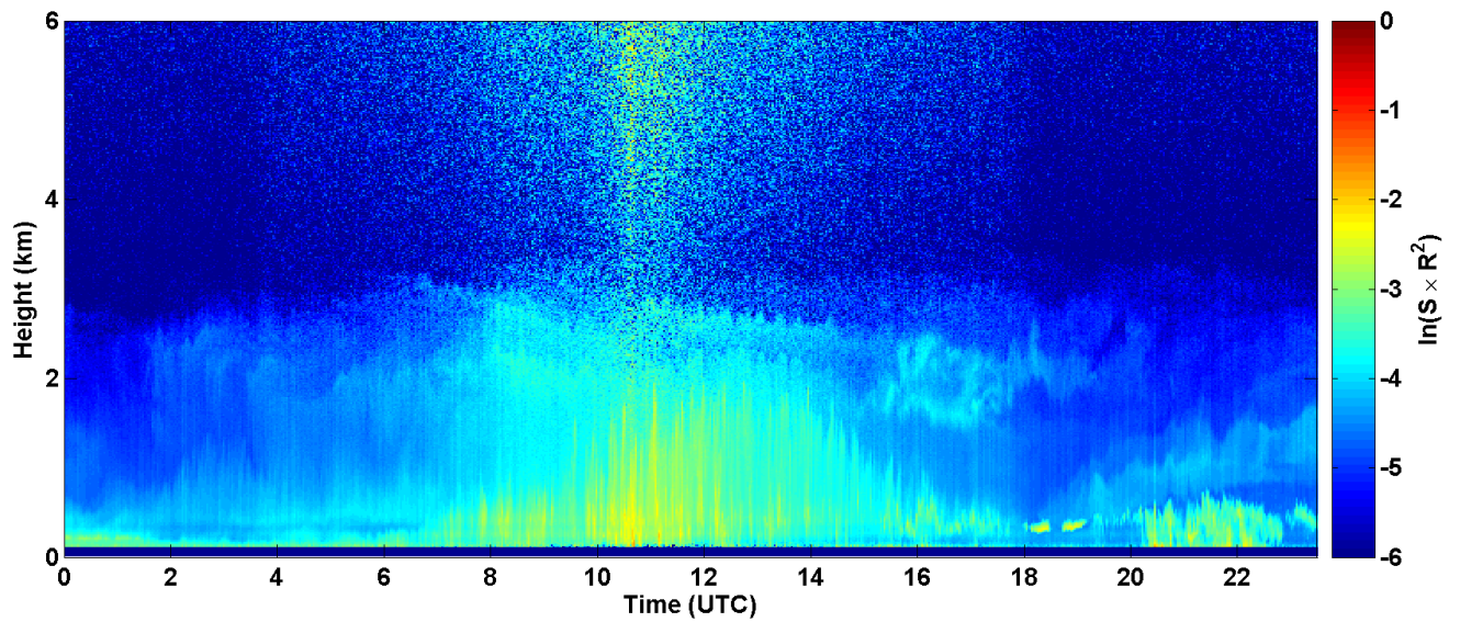
2017-05-22 RCS quick look CHM15k - ILVA LIDAR3 AGGLOMERATO
