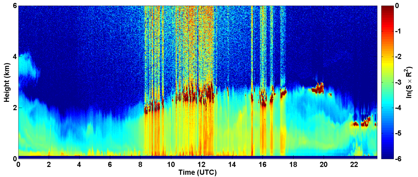
2017-05-08 RCS quick look CHM15k - ILVA LIDAR3 AGGLOMERATO
