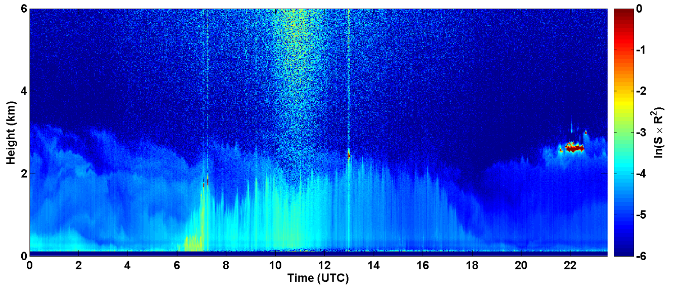
2017-05-28 RCS quick look CHM15k - ILVA LIDAR3 AGGLOMERATO
