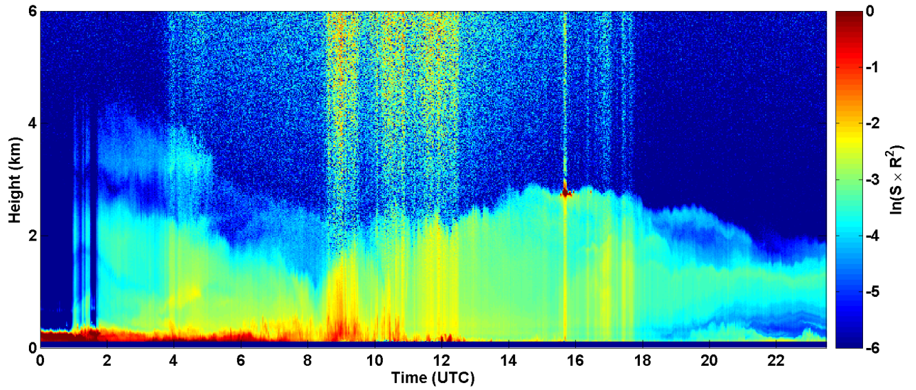
2017-05-14 RCS quick look CHM15k - ILVA LIDAR3 AGGLOMERATO
