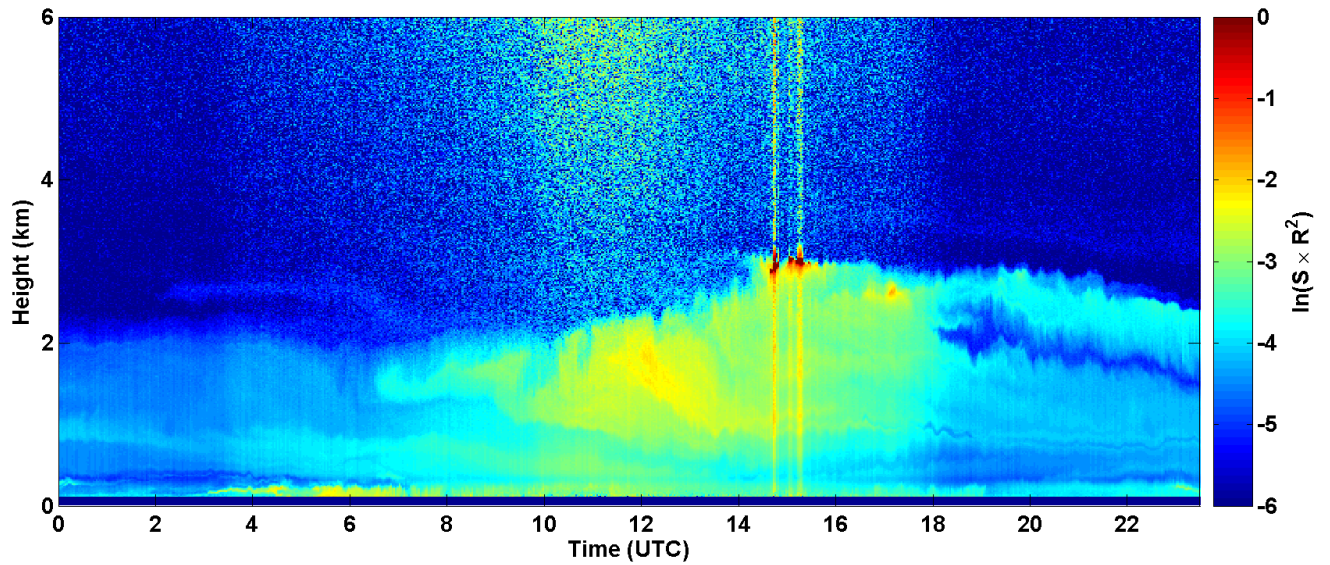
2017-05-30 RCS quick look CHM15k - ILVA LIDAR2 PARCHI
