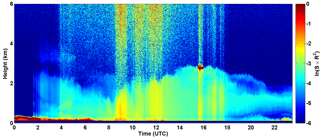
2017-05-14 RCS quick look CHM15k - ILVA LIDAR2 PARCHI
