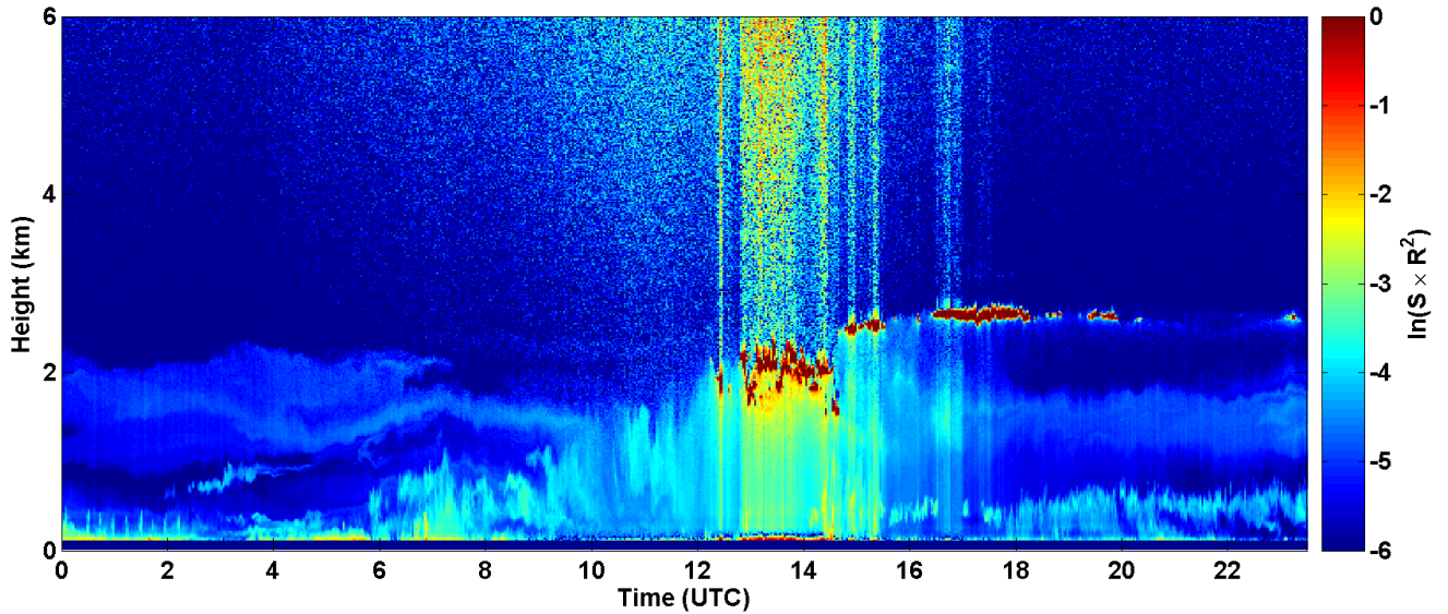
2017-05-02 RCS quick look CHM15k - ILVA LIDAR3 AGGLOMERATO
