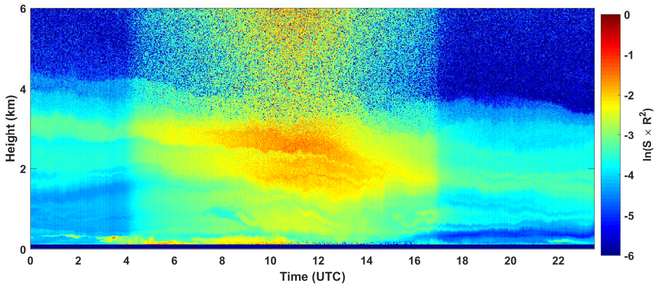
2018-04-26 RCS quick look CHM15k - ILVA LIDAR2 PARCHI
