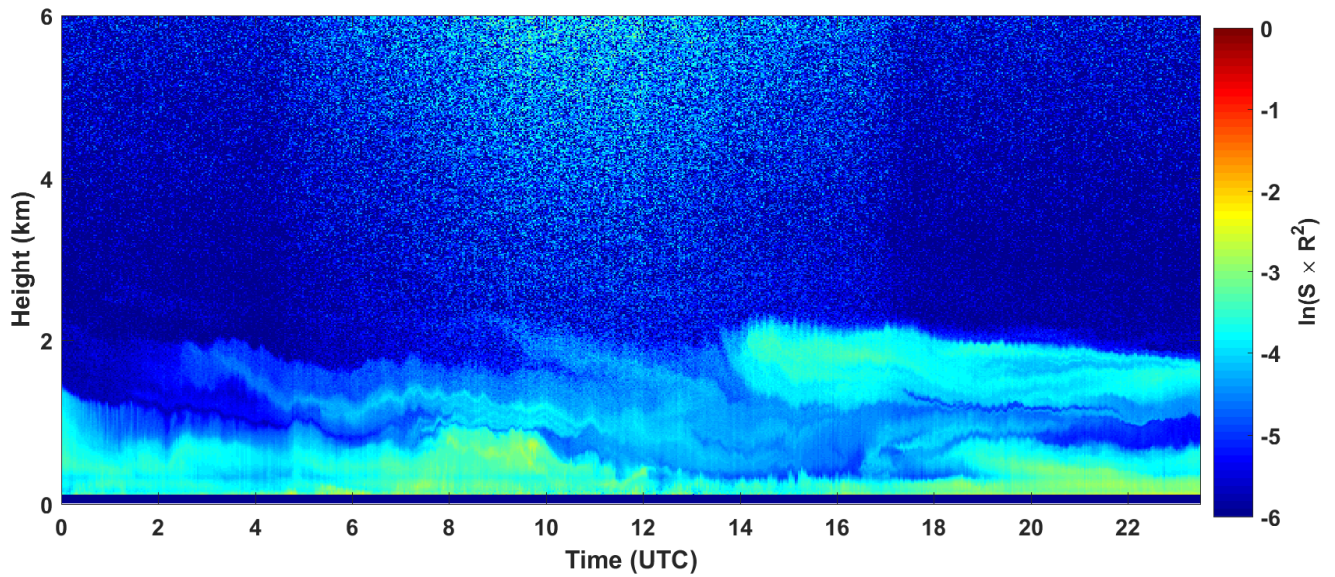
2018-04-02 RCS quick look CHM15k - ILVA LIDAR2 PARCHI
