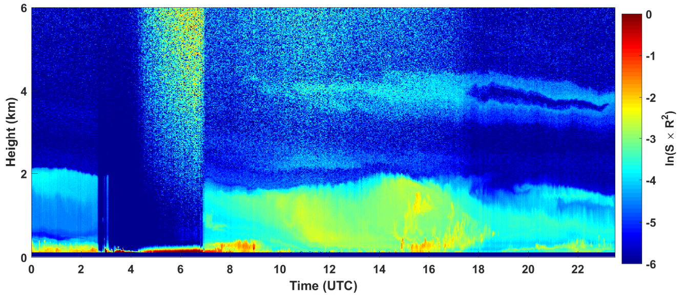
2018-04-24 RCS quick look CHM15k - ILVA LIDAR3 AGGLOMERATO
