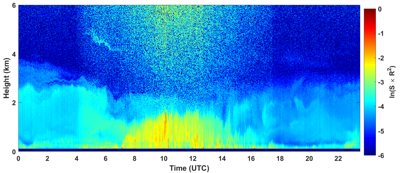
2018-04-20 RCS quick look CHM15k - ILVA LIDAR2 PARCHI
