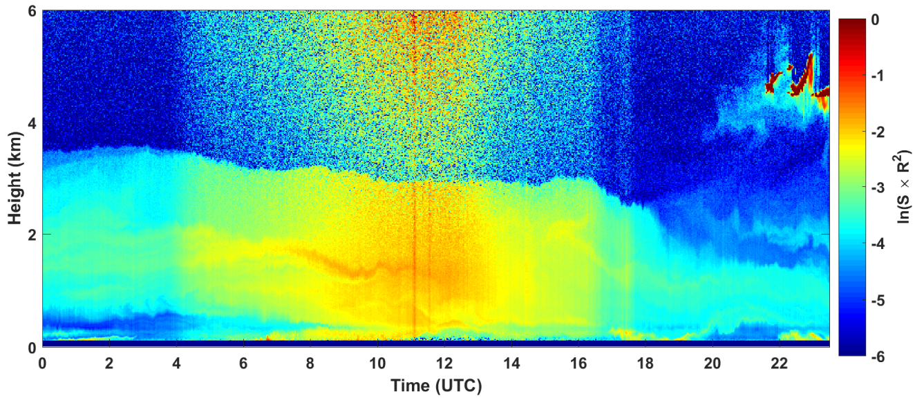
2018-04-28 RCS quick look CHM15k - ILVA LIDAR2 PARCHI
