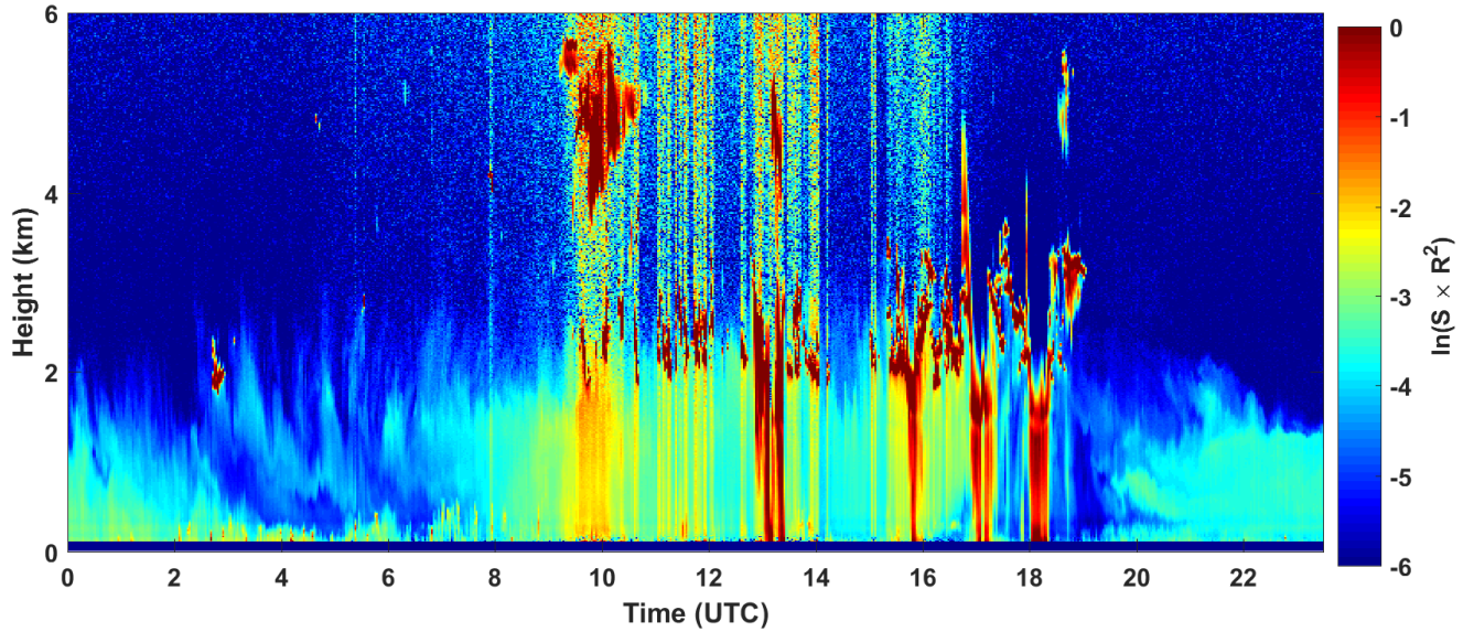
2018-04-02 RCS quick look CHM15k - ILVA LIDAR3 AGGLOMERATO
