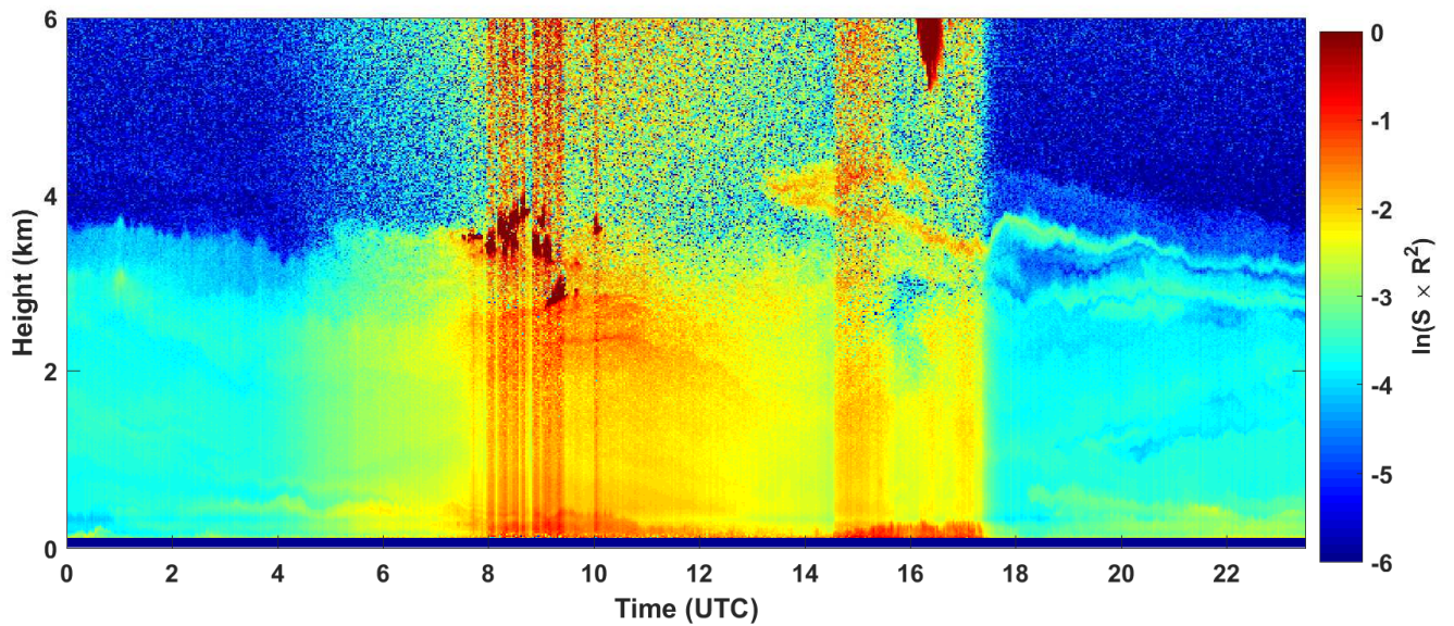
2018-04-30 RCS quick look CHM15k - ILVA LIDAR2 PARCHI
