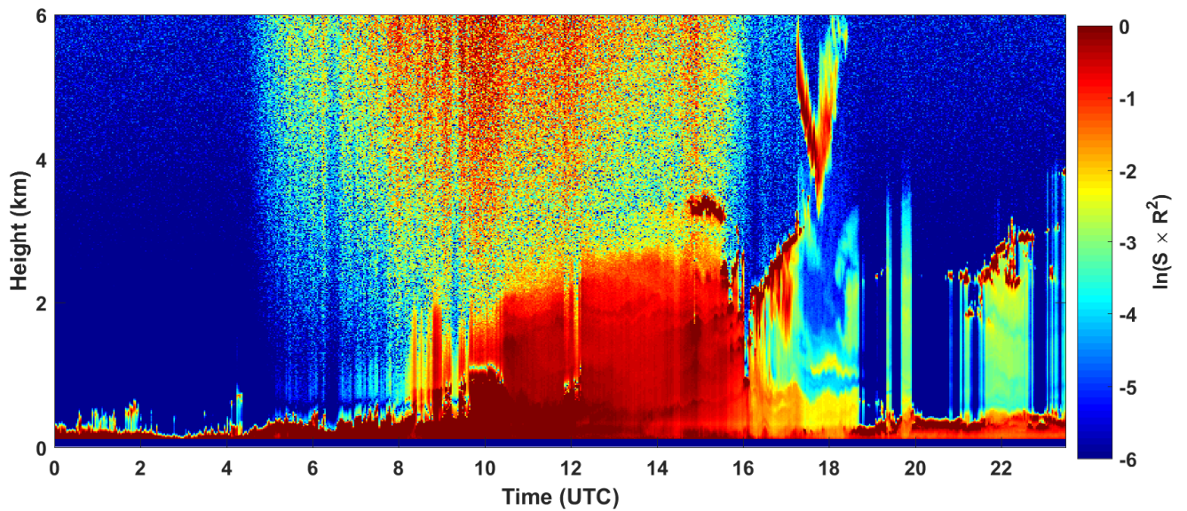
2018-04-16 RCS quick look CHM15k - ILVA LIDAR2 PARCHI
