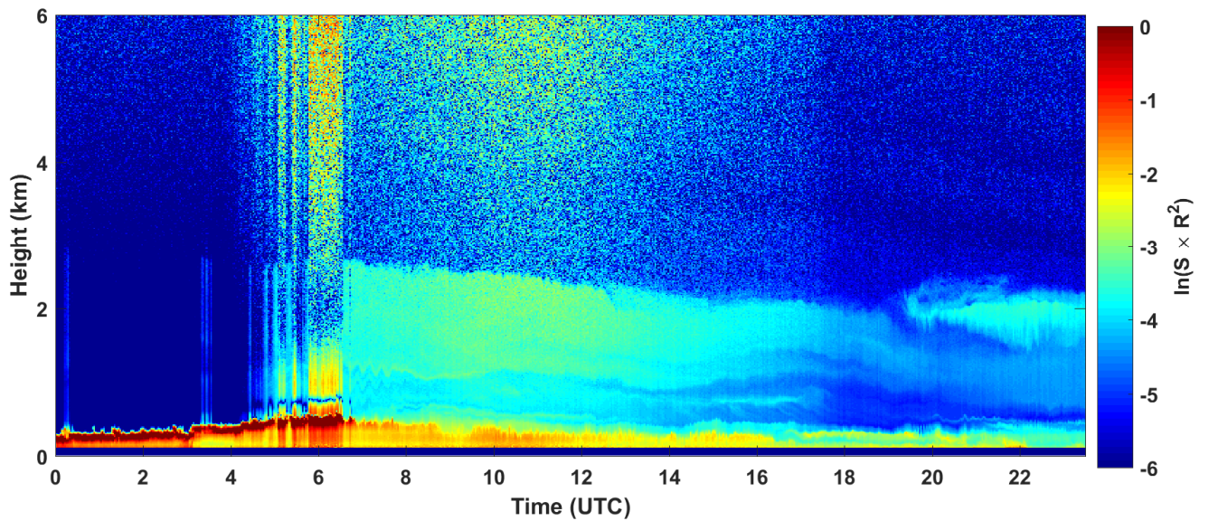
2018-04-22 RCS quick look CHM15k - ILVA LIDAR2 PARCHI
