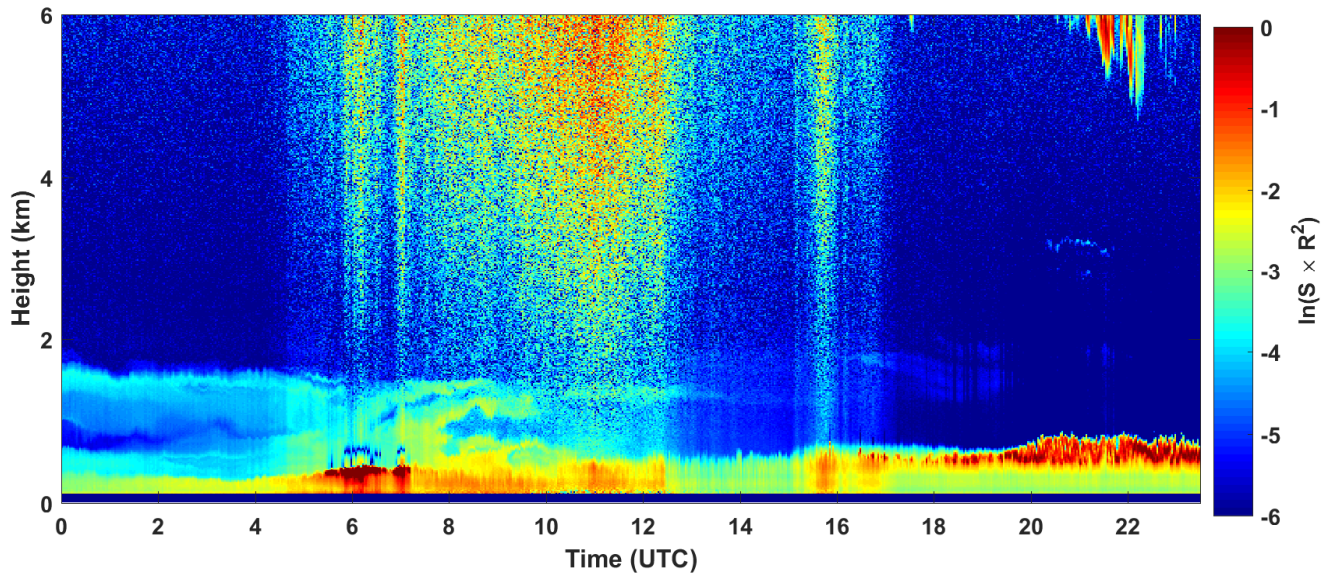
2018-04-04 RCS quick look CHM15k - ILVA LIDAR2 PARCHI
