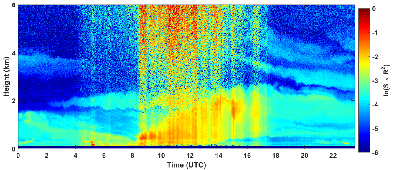
2018-04-24 RCS quick look CHM15k - ILVA LIDAR2 PARCHI
