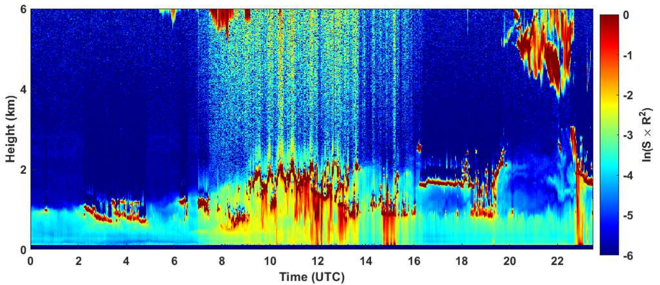
2020-11-28 RCS quick look CHM15k - ILVA LIDAR3 AGGLOMERATO
