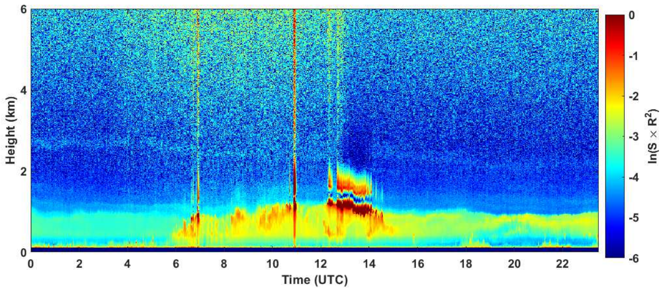
2020-11-26 RCS quick look CHM15k - ILVA LIDAR2 PARCHI
