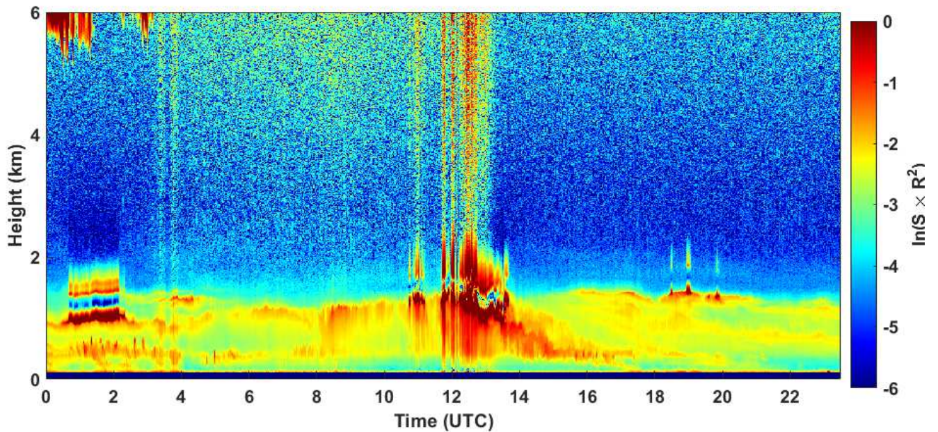
2020-11-02 RCS quick look CHM15k - ILVA LIDAR2 PARCHI
