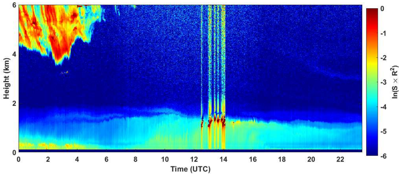
2020-11-26 RCS quick look CHM15k - ILVA LIDAR3 AGGLOMERATO
