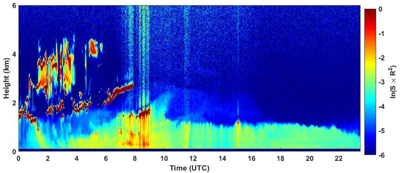
2020-11-30 RCS quick look CHM15k - ILVA LIDAR3 AGGLOMERATO
