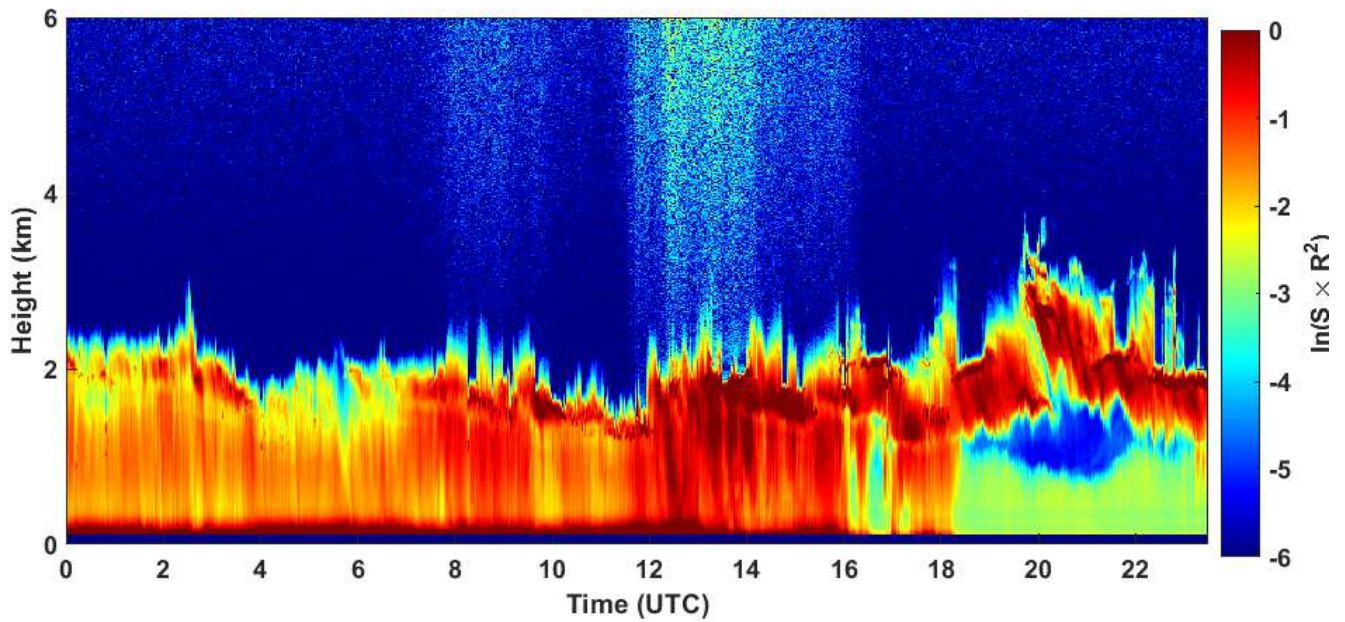
2020-11-22 RCS quick look CHM15k - ILVA LIDAR3 AGGLOMERATO
