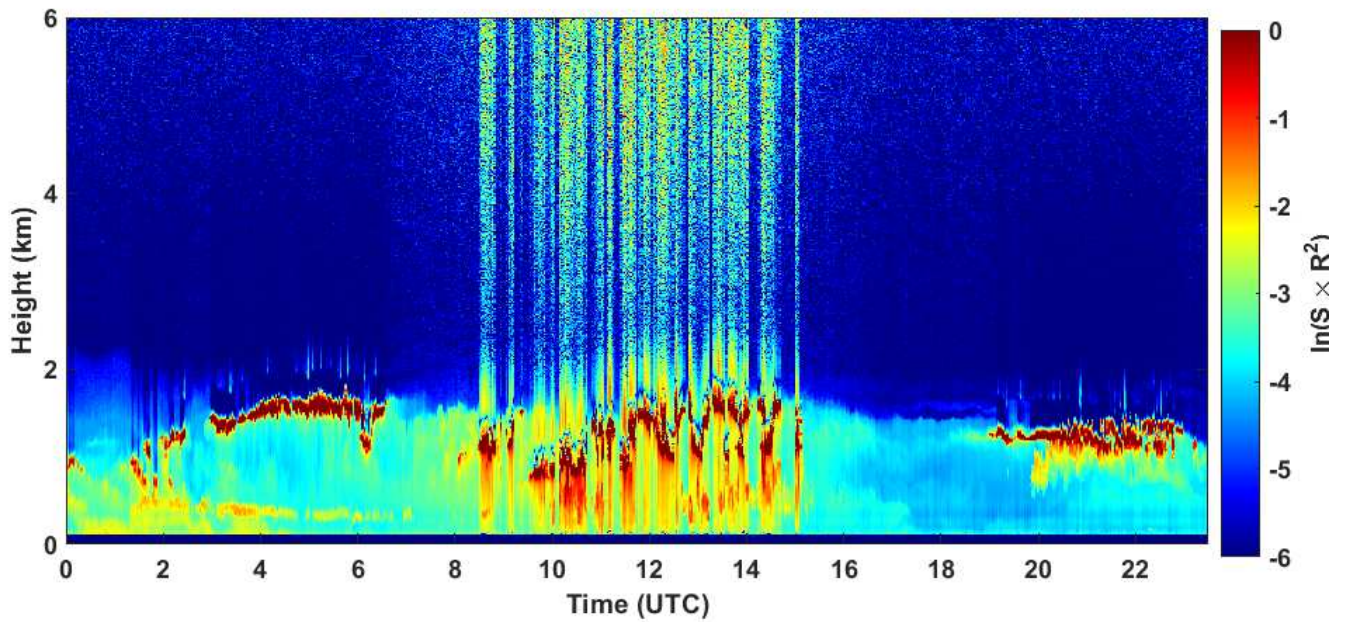
2020-11-20 RCS quick look CHM15k - ILVA LIDAR3 AGGLOMERATO
