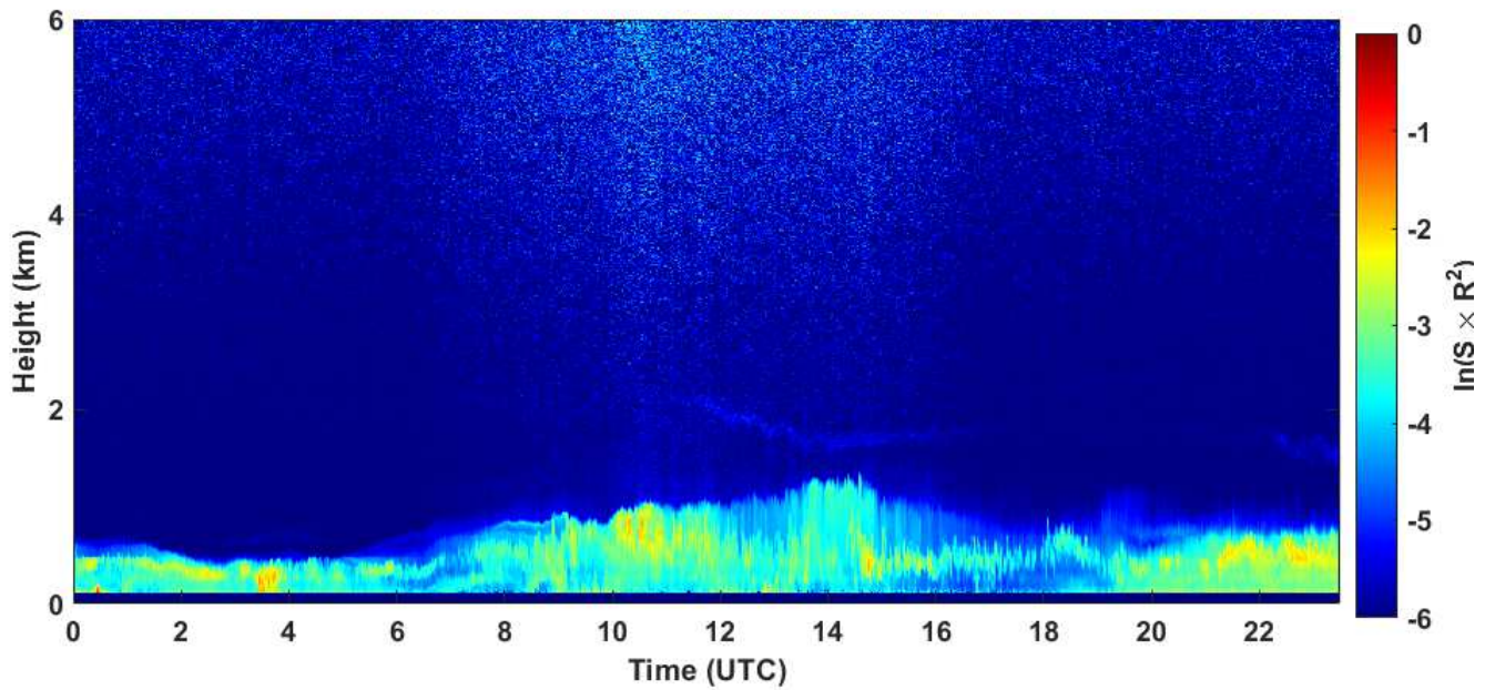
2020-11-10 RCS quick look CHM15k - ILVA LIDAR3 AGGLOMERATO
