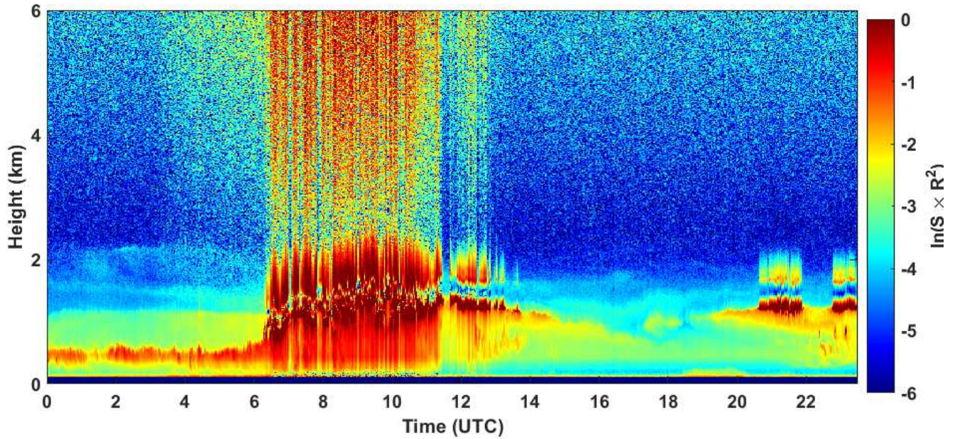
2020-11-12 RCS quick look CHM15k - ILVA LIDAR2 PARCHI
