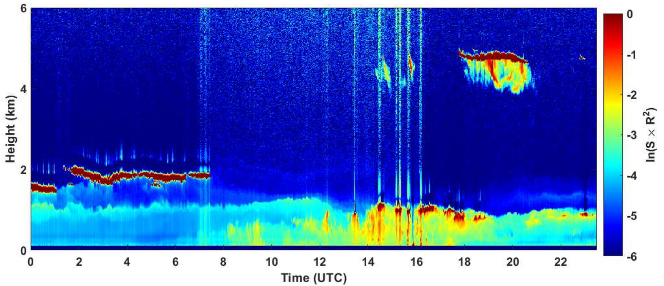
2020-11-24 RCS quick look CHM15k - ILVA LIDAR3 AGGLOMERATO
