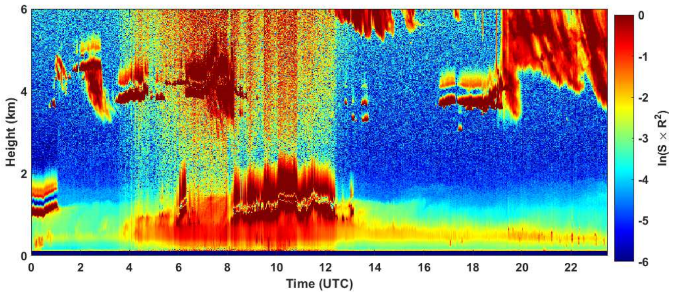
2020-11-24 RCS quick look CHM15k - ILVA LIDAR2 PARCHI
