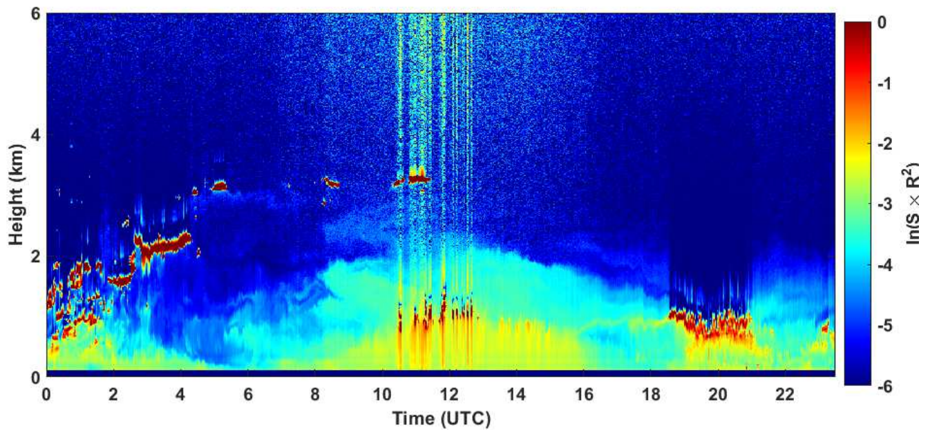
2020-11-18 RCS quick look CHM15k - ILVA LIDAR3 AGGLOMERATO
