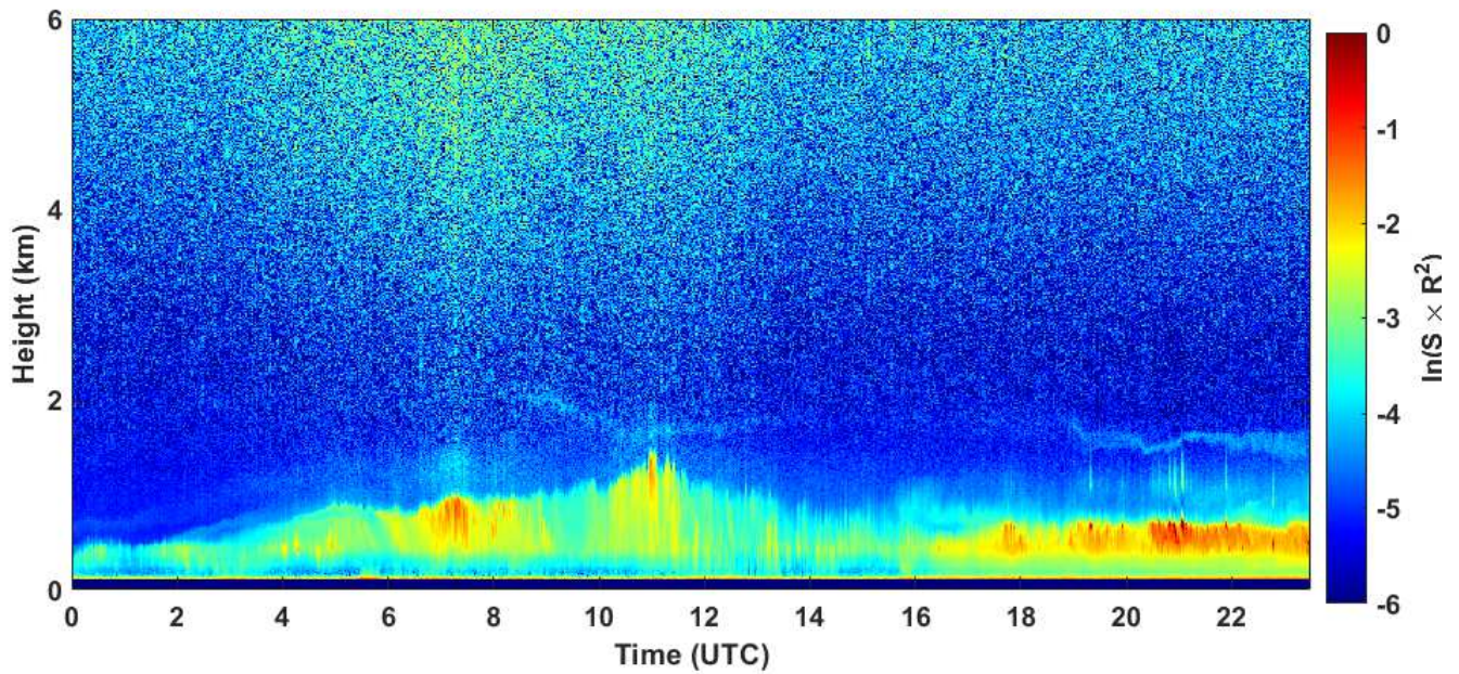
2020-11-10 RCS quick look CHM15k - ILVA LIDAR2 PARCHI
