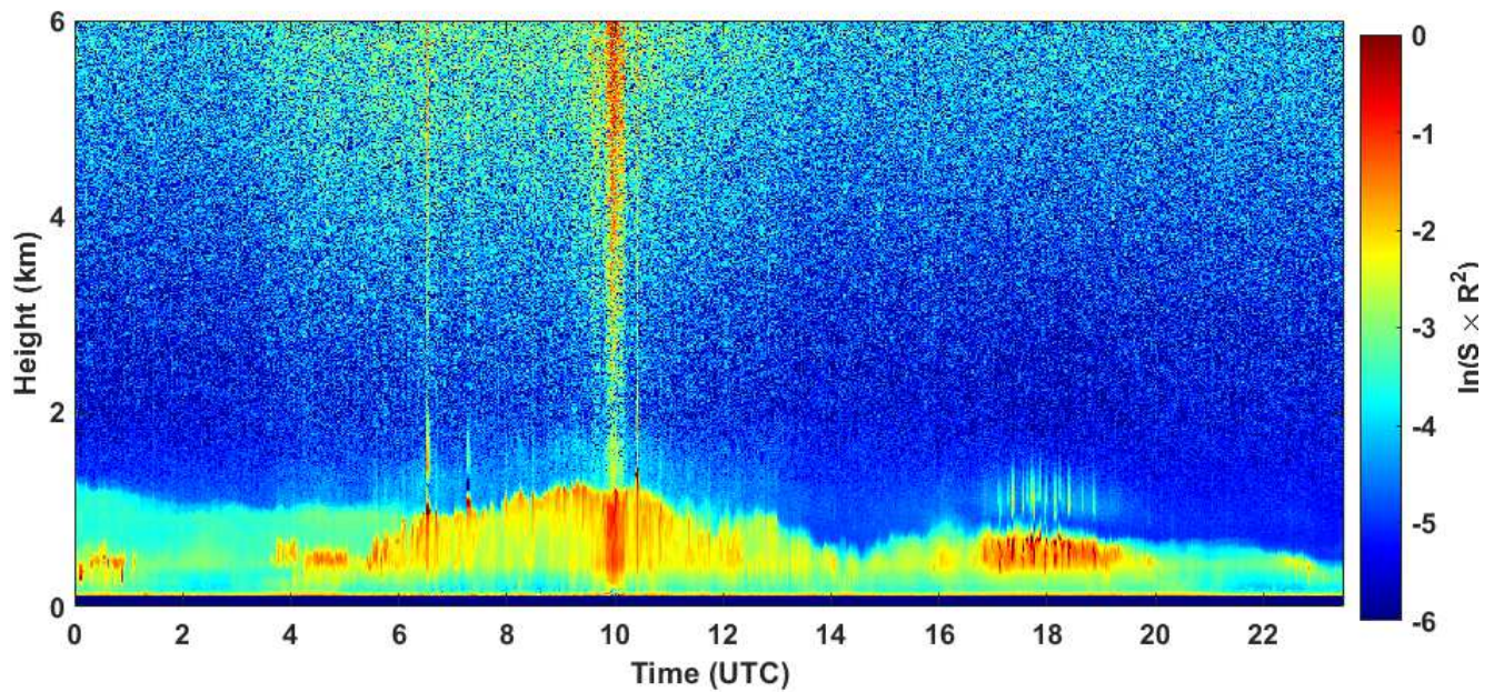
2020-11-08 RCS quick look CHM15k - ILVA LIDAR2 PARCHI
