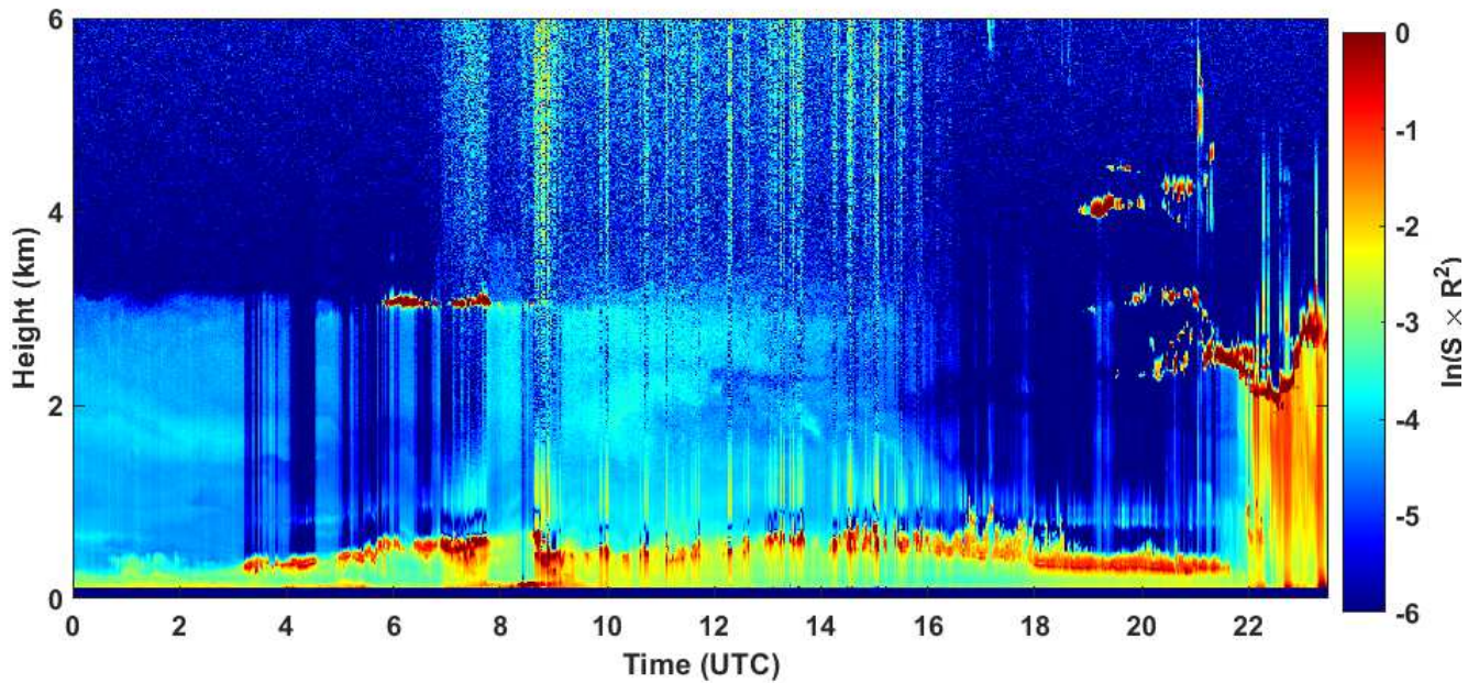
2020-11-16 RCS quick look CHM15k - ILVA LIDAR3 AGGLOMERATO
