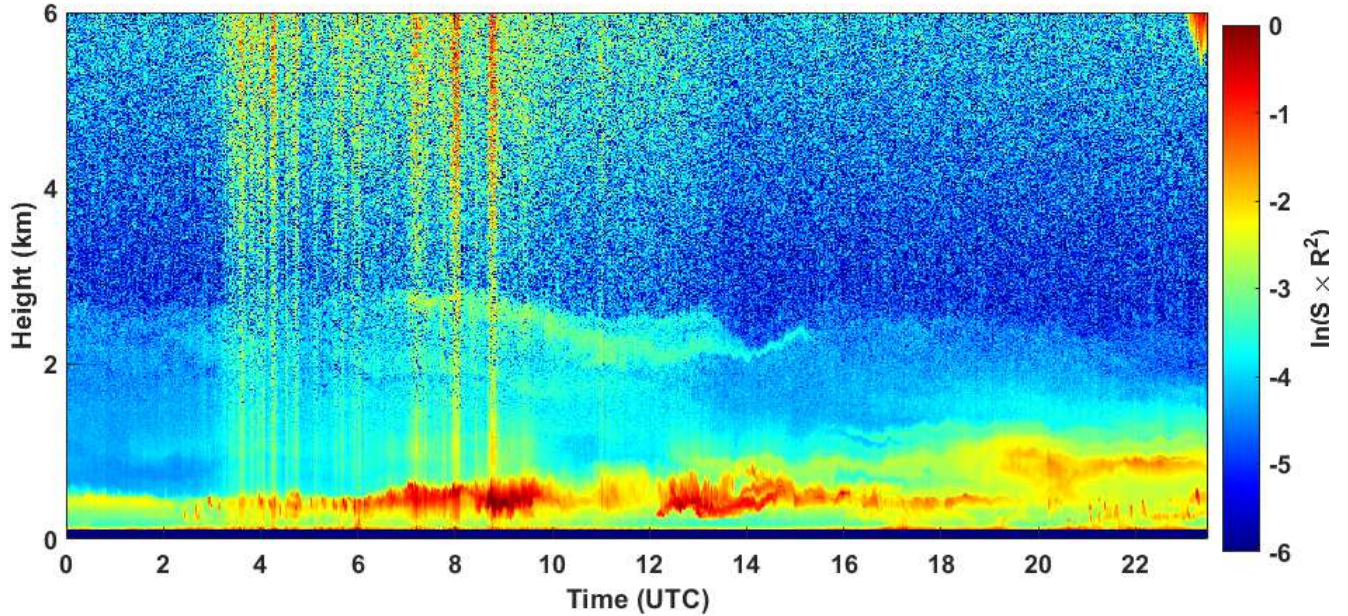
2020-11-02 RCS quick look CHM15k - ILVA LIDAR2 PARCHI
