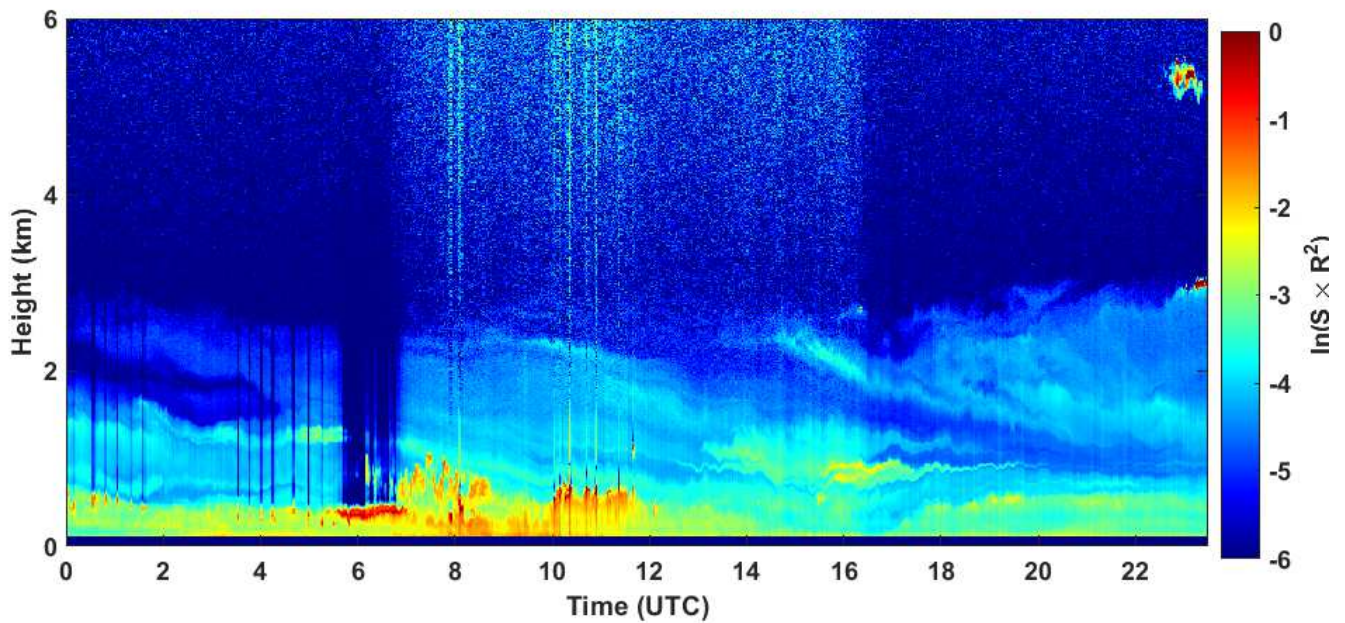
2020-11-14 RCS quick look CHM15k - ILVA LIDAR3 AGGLOMERATO
