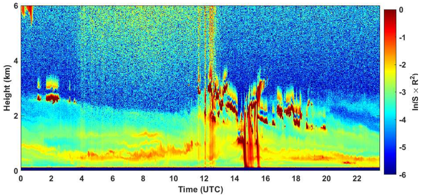
2020-11-14 RCS quick look CHM15k - ILVA LIDAR2 PARCHI
