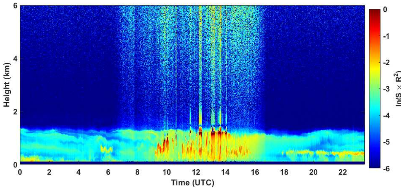
2020-11-04 RCS quick look CHM15k - ILVA LIDAR3 AGGLOMERATO
