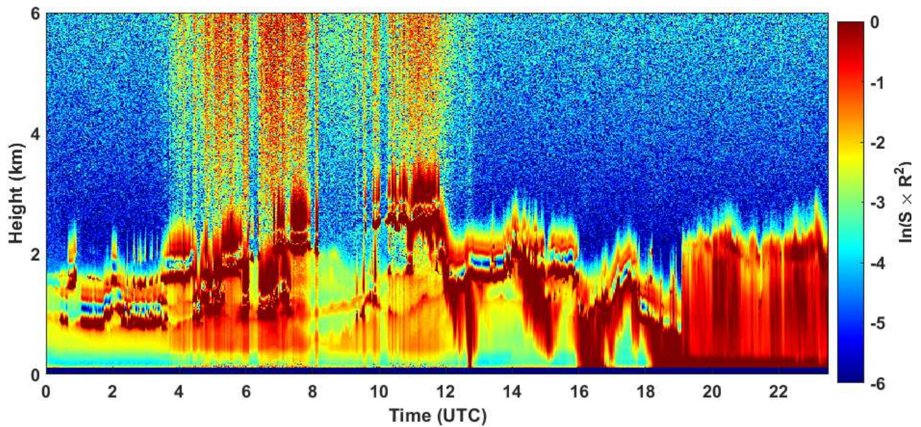
2020-11-20 RCS quick look CHM15k - ILVA LIDAR2 PARCHI
