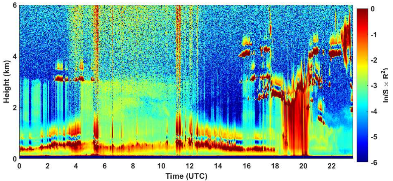
2020-11-16 RCS quick look CHM15k - ILVA LIDAR2 PARCHI
