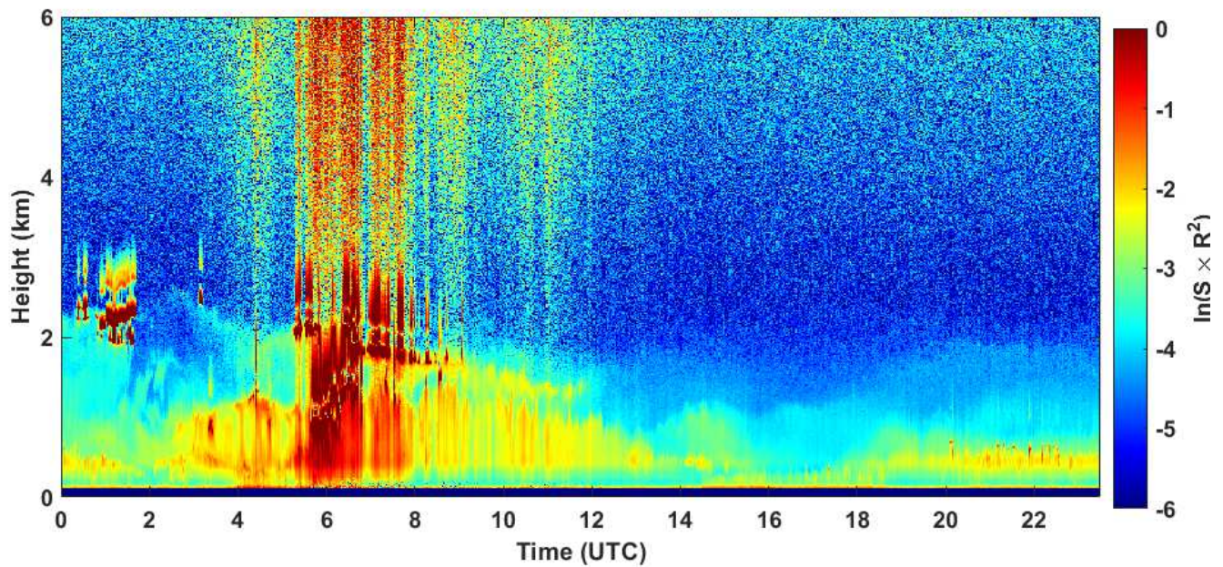
2020-11-06 RCS quick look CHM15k - ILVA LIDAR2 PARCHI
