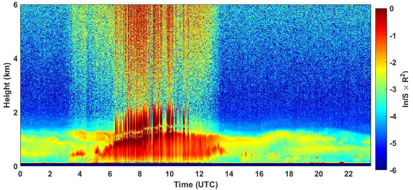
2020-11-04 RCS quick look CHM15k - ILVA LIDAR2 PARCHI
