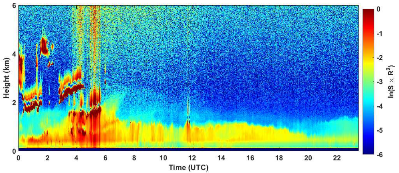
2020-11-30 RCS quick look CHM15k - ILVA LIDAR2 PARCHI
