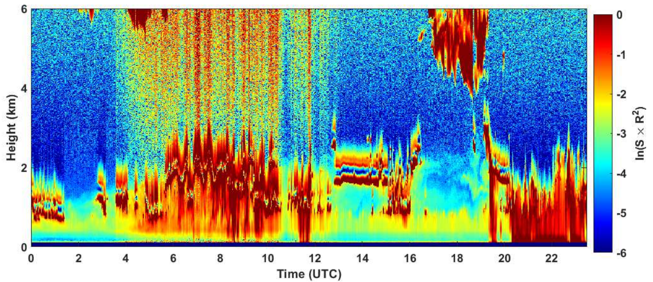
2020-11-28 RCS quick look CHM15k - ILVA LIDAR2 PARCHI
