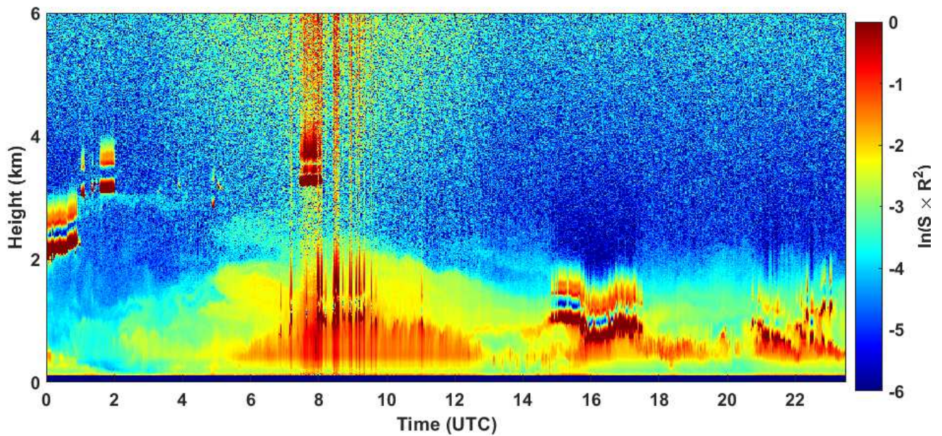
2020-11-18 RCS quick look CHM15k - ILVA LIDAR2 PARCHI
