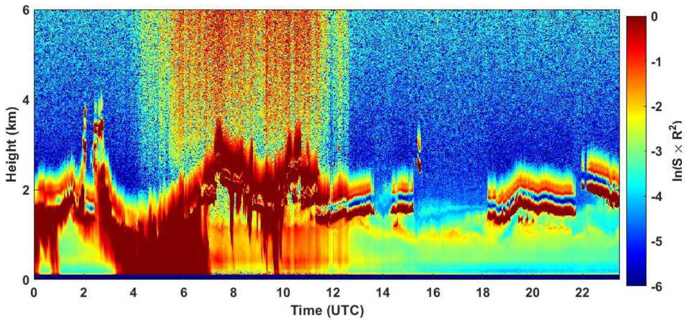
2020-11-22 RCS quick look CHM15k - ILVA LIDAR2 PARCHI
