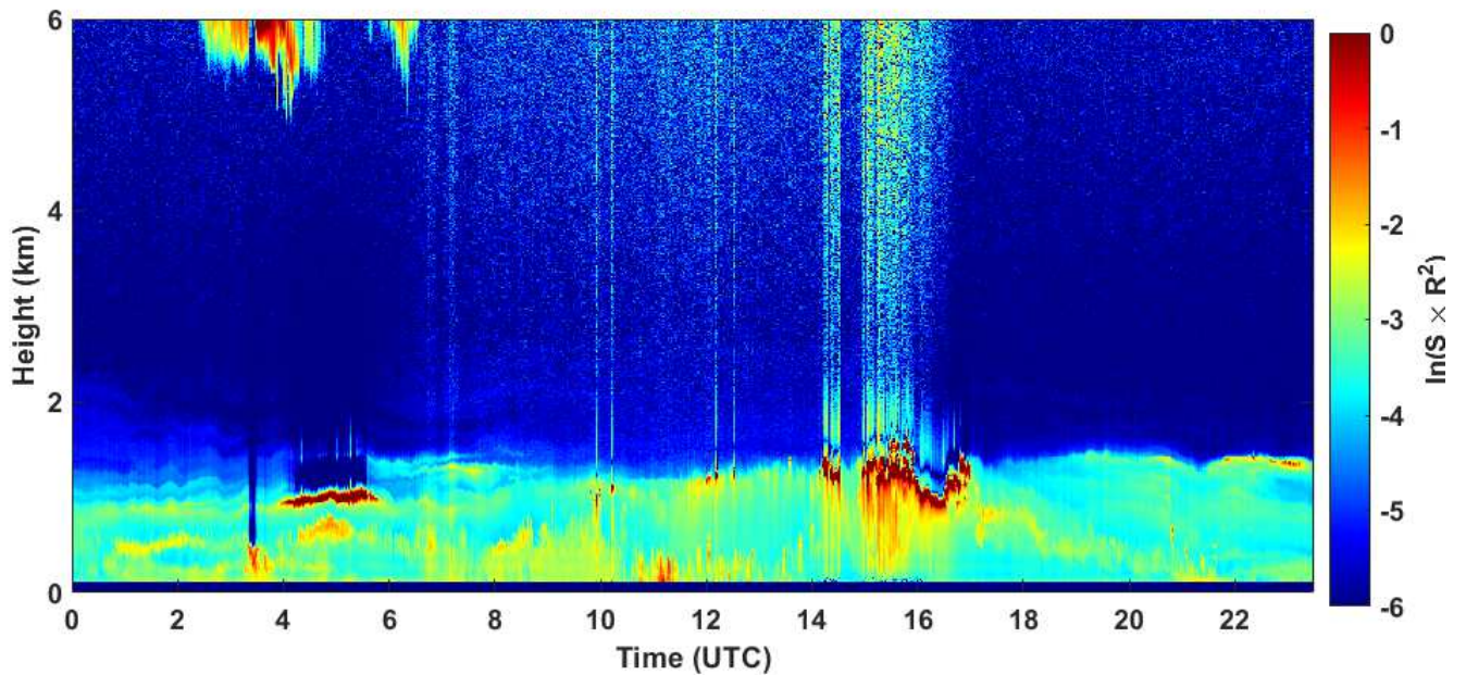
2020-11-02 RCS quick look CHM15k - ILVA LIDAR3 AGGLOMERATO
