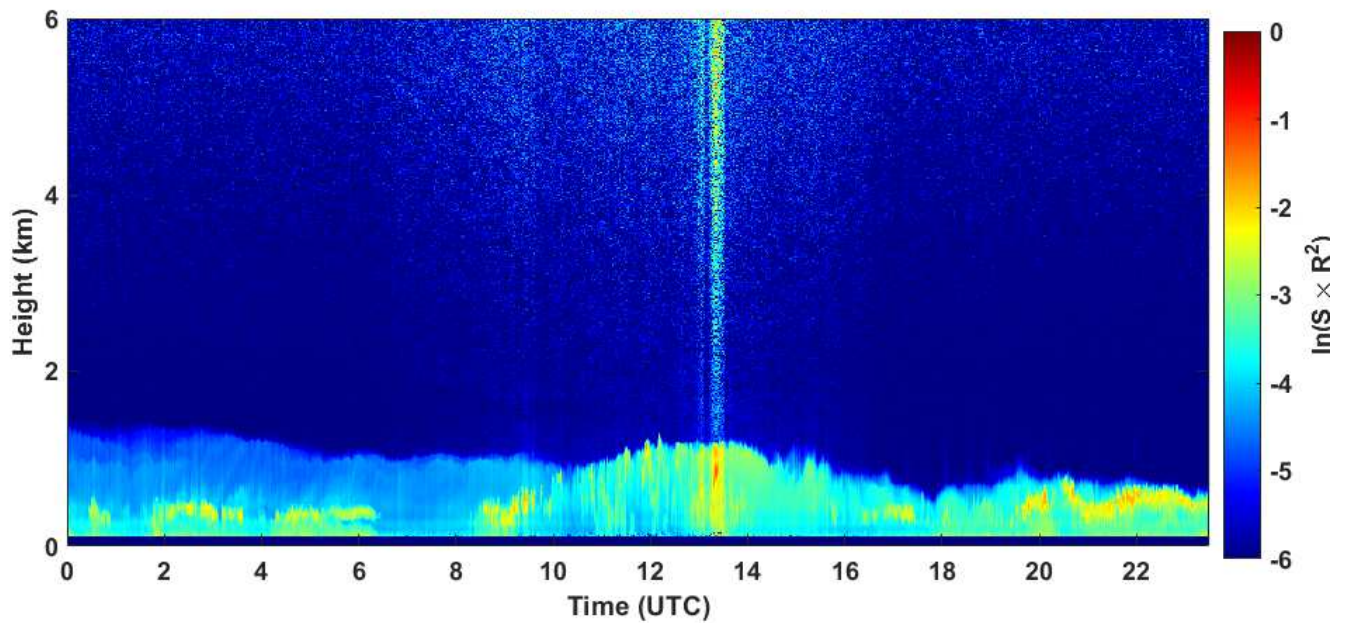
2020-11-08 RCS quick look CHM15k - ILVA LIDAR3 AGGLOMERATO
