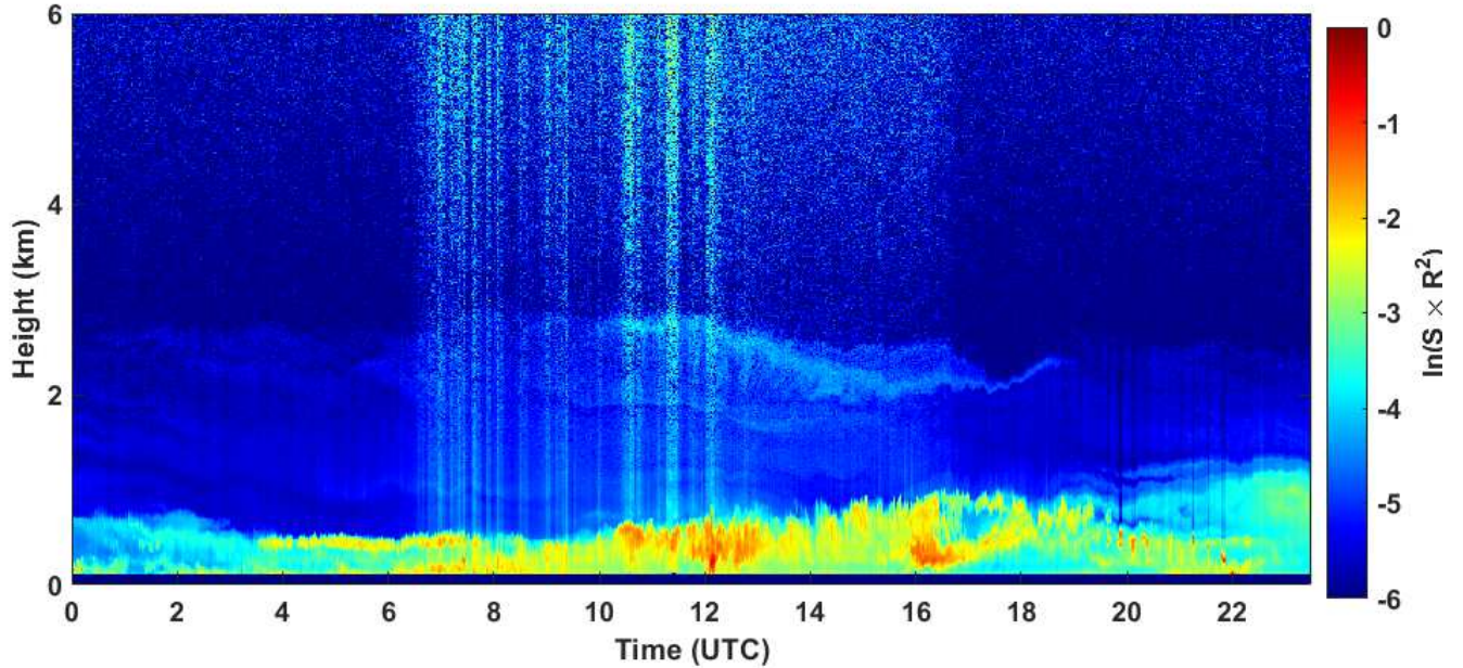
2020-11-02 RCS quick look CHM15k - ILVA LIDAR3 AGGLOMERATO
