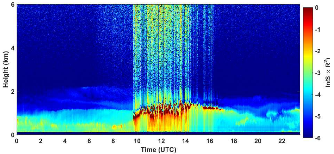
2020-11-12 RCS quick look CHM15k - ILVA LIDAR3 AGGLOMERATO
