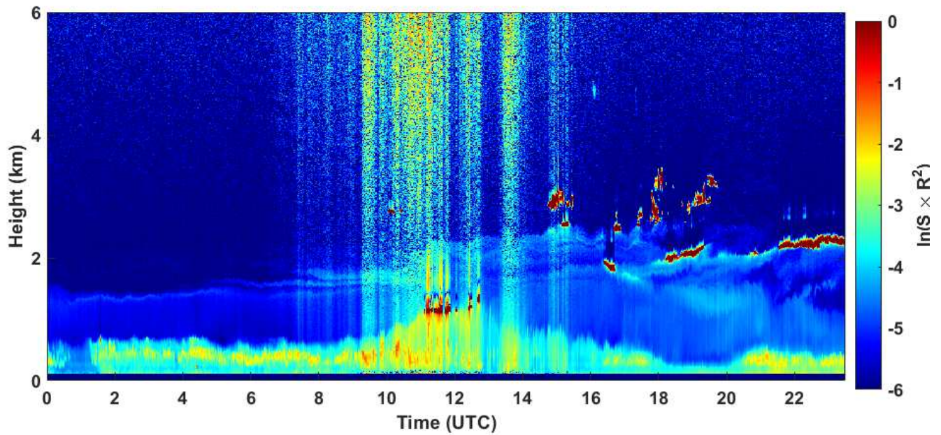
2020-11-06 RCS quick look CHM15k - ILVA LIDAR3 AGGLOMERATO
